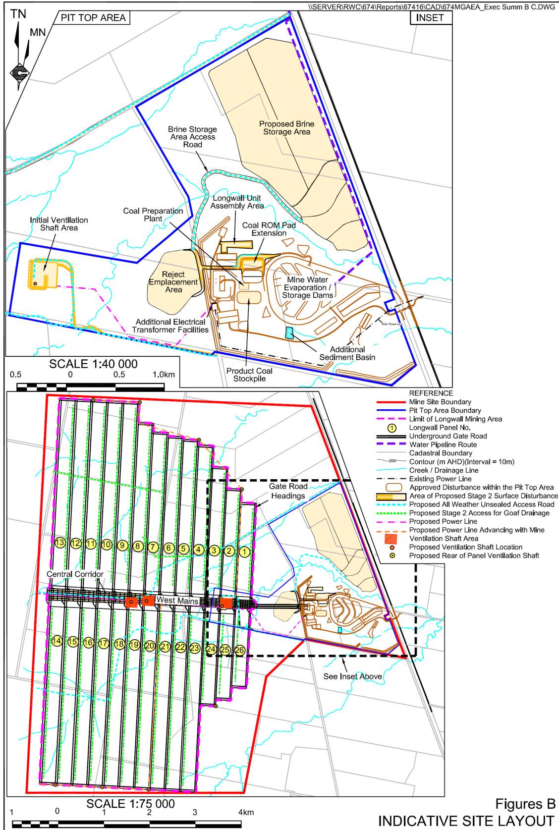
Figure 1: Project Layout
