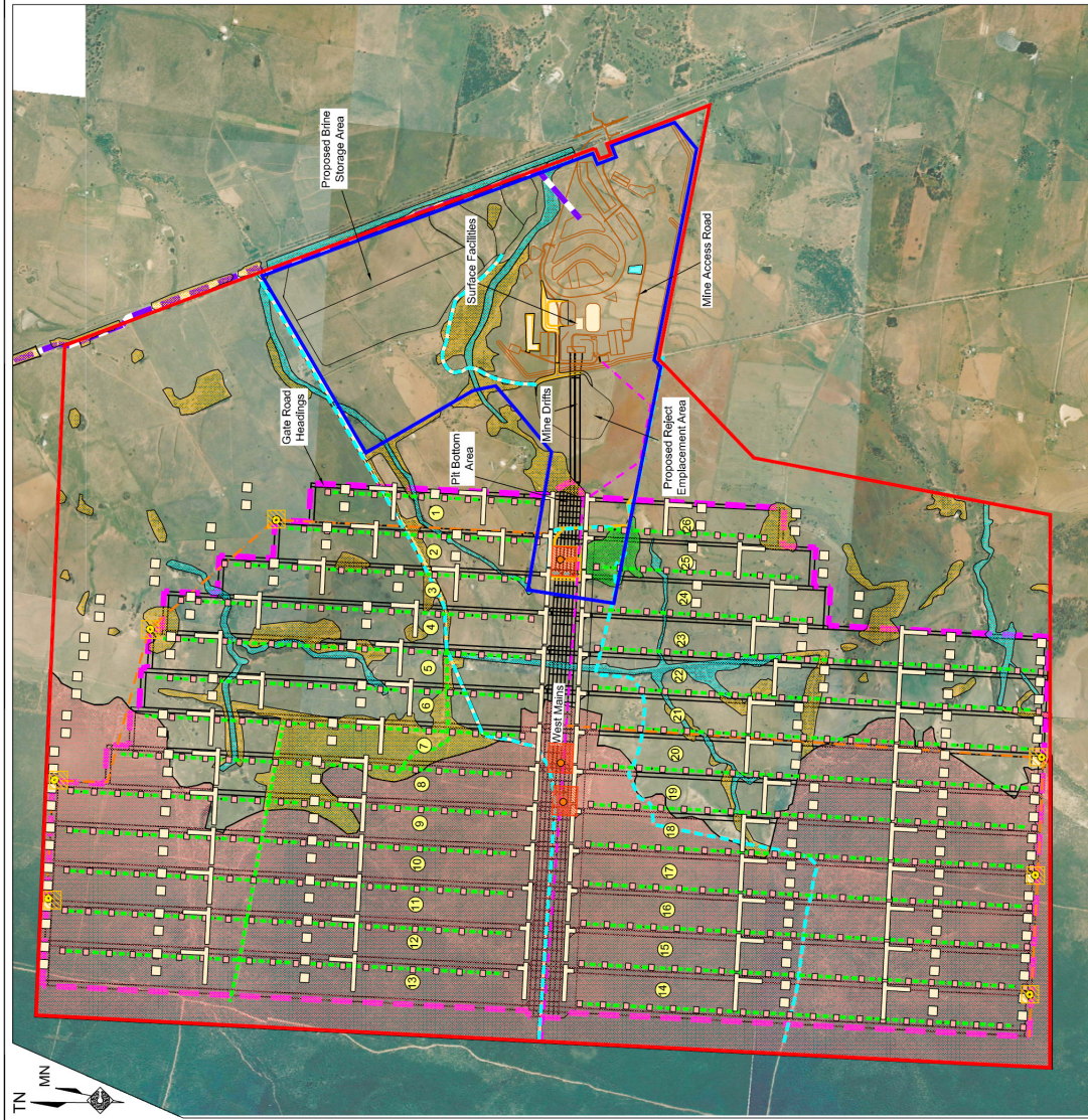
Figure 3: Surface Facilities Layout
