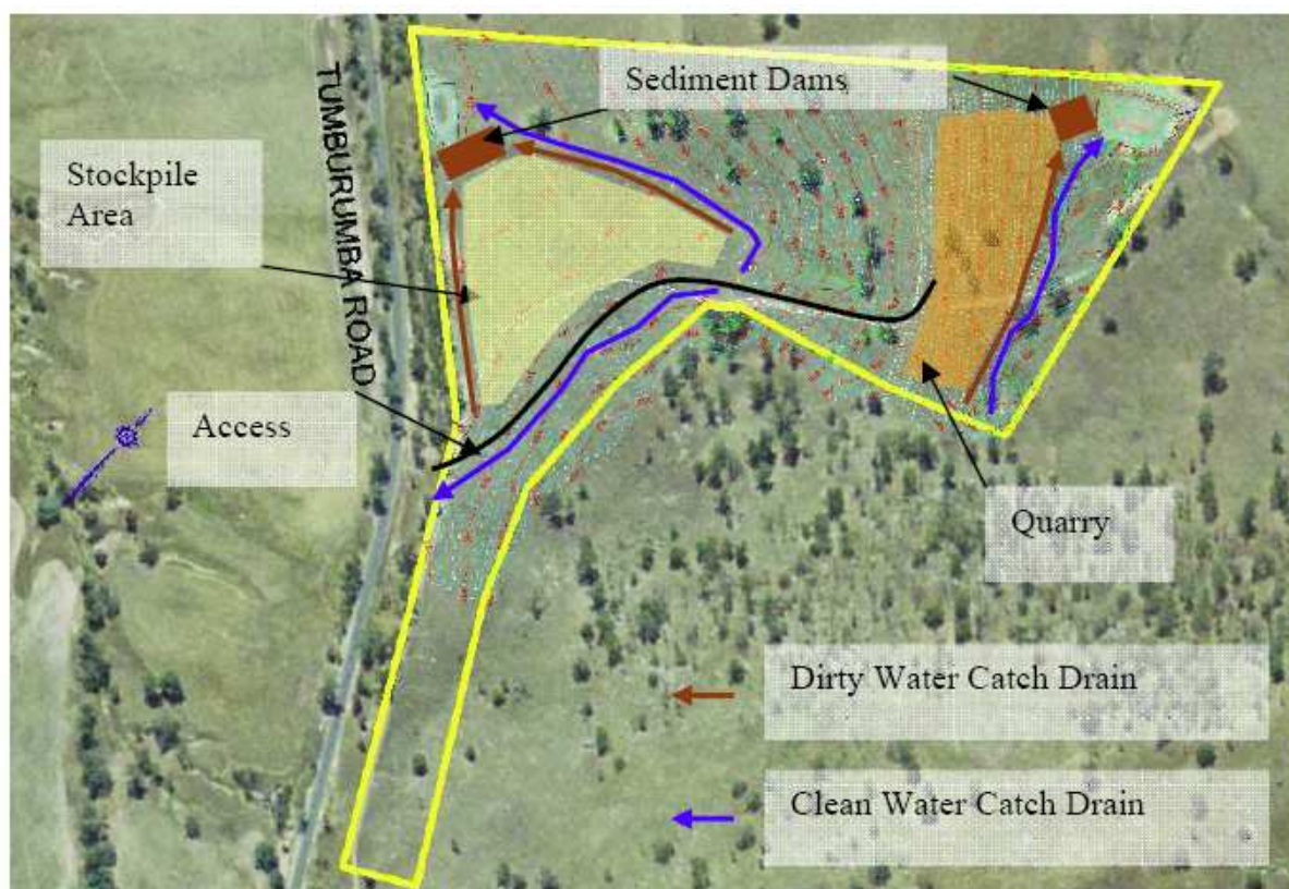
Figure 4. Indicative Erosion and Sediment Control Plan
