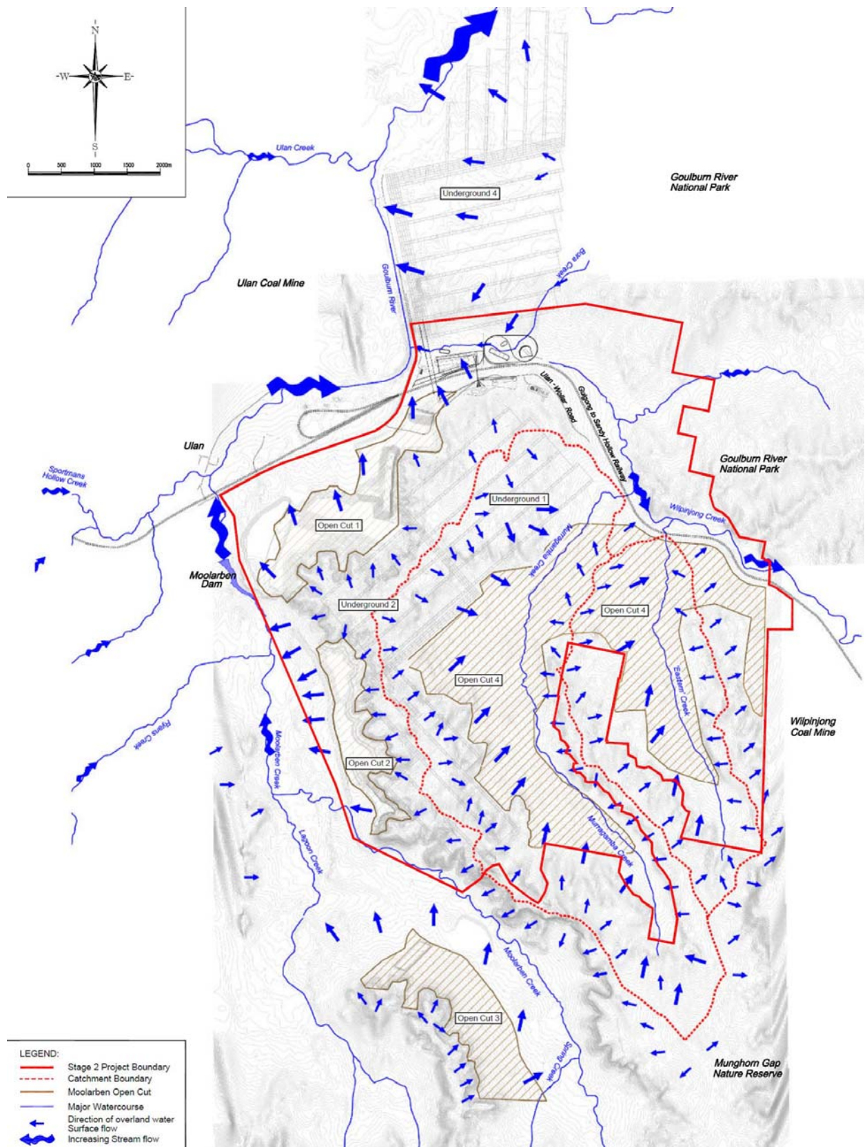
Figure 17: Existing Catchment Surface Water Hydrology
