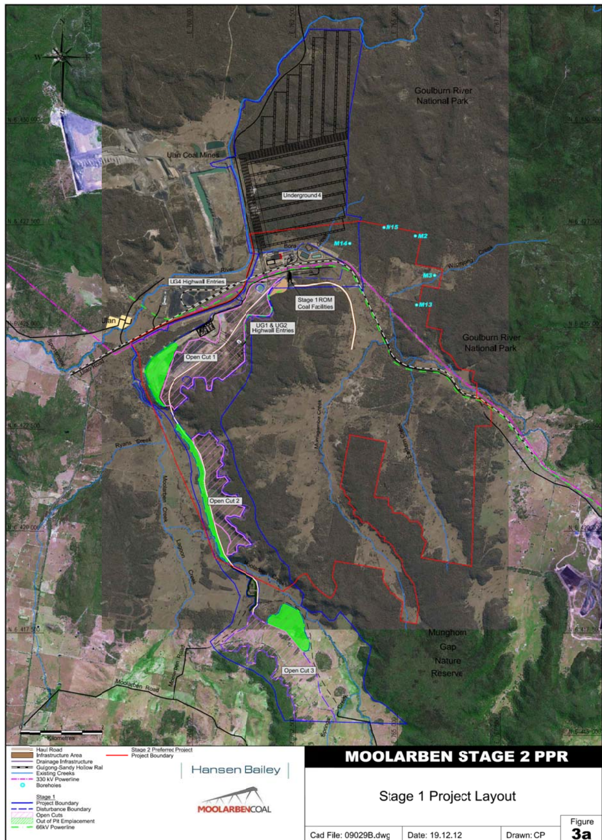
Figure 3: Moolarben Coal Mine – Stage 1 Layout
