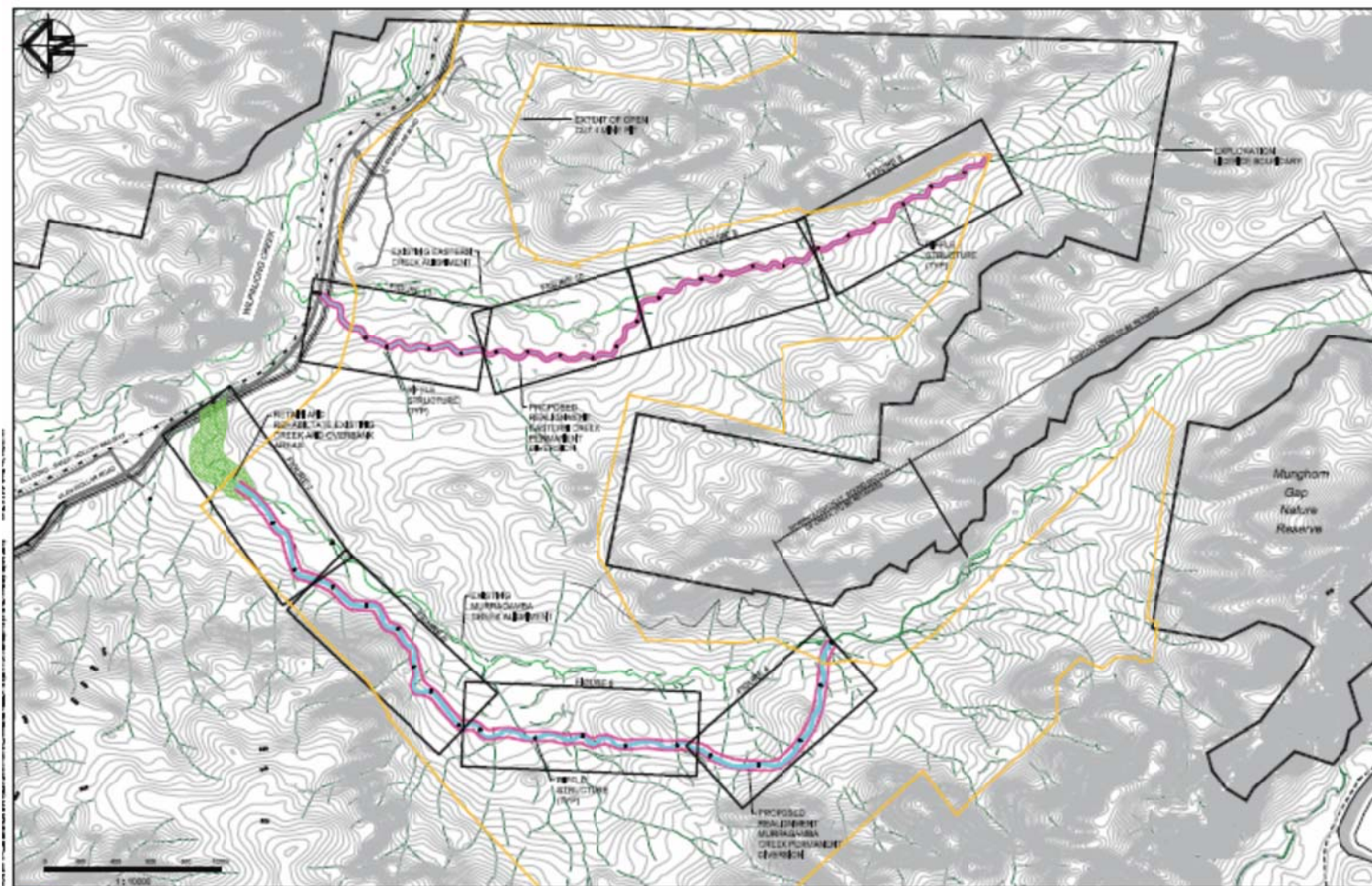
Figure 18: Existing Catchment Surface Water Hydrology
