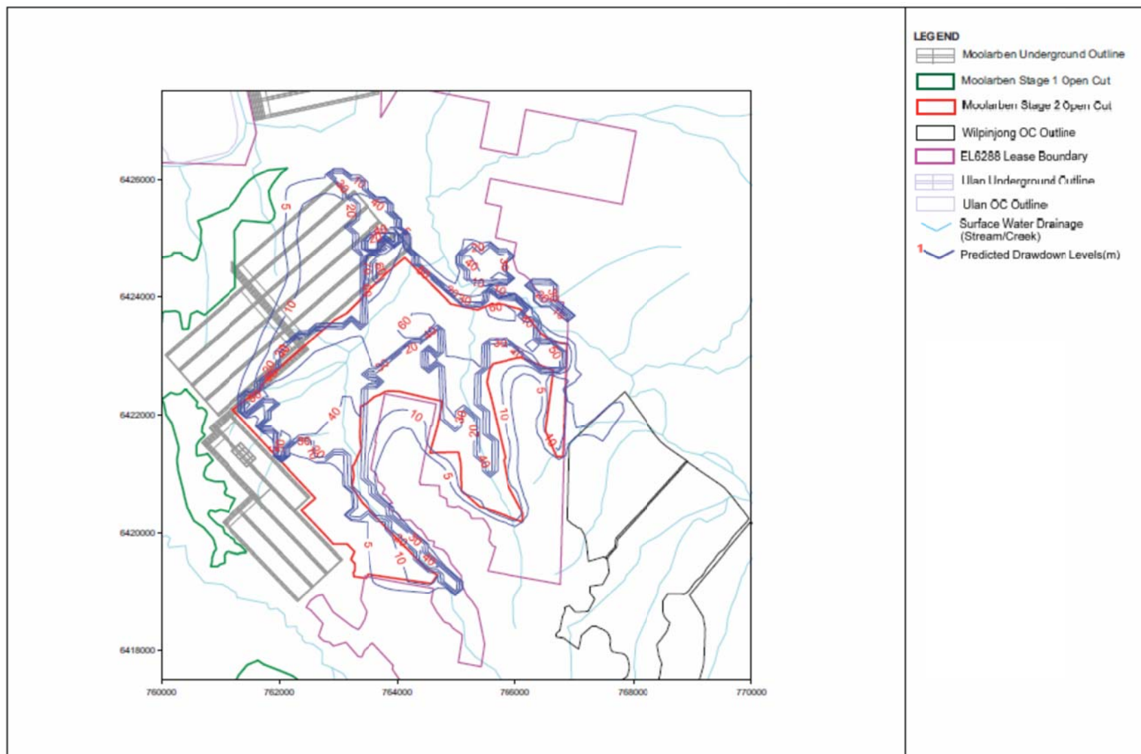
Figure 16: Predicted Groundwater Drawdown in the Lower Permian Coal Measures
