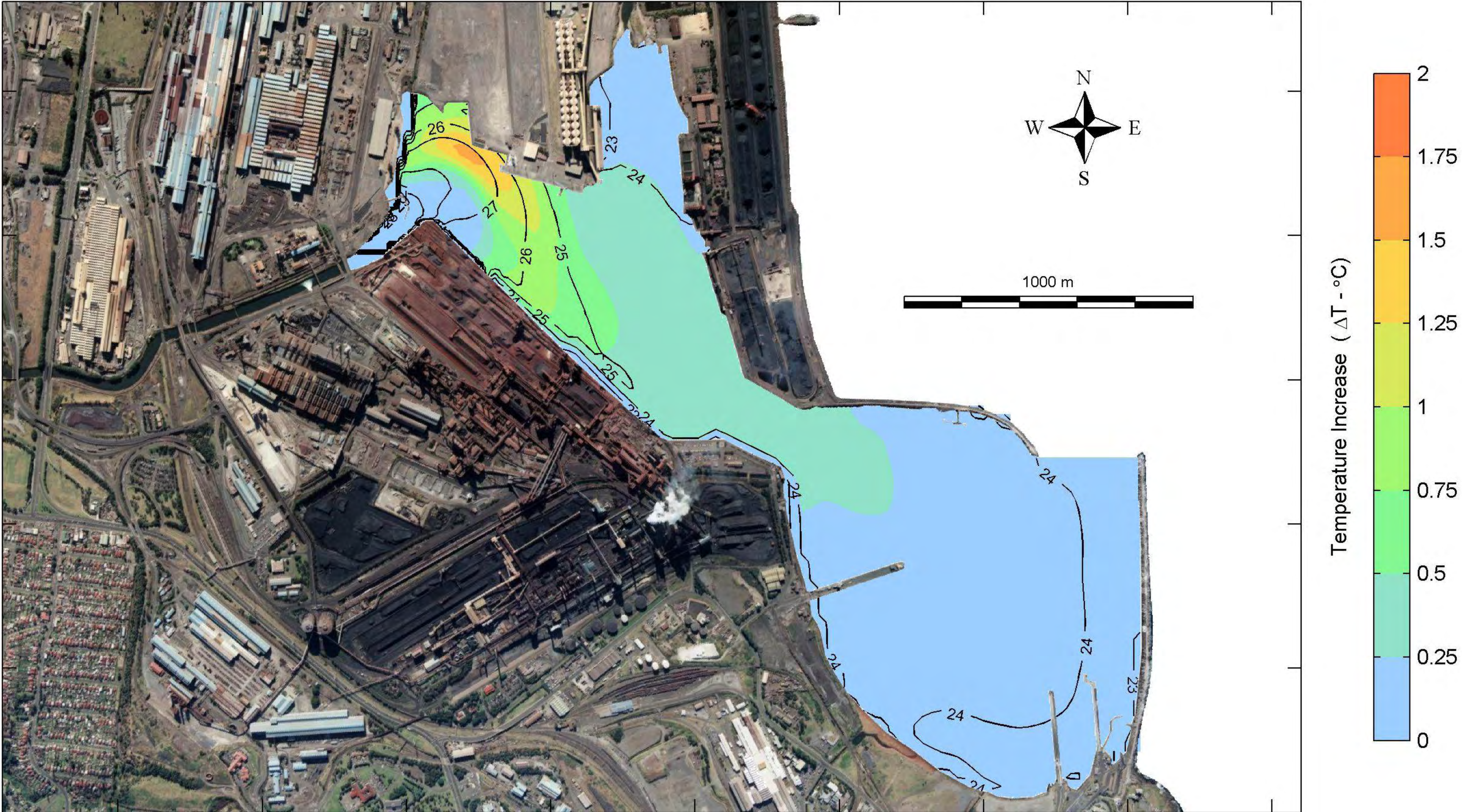
Surface Layer
