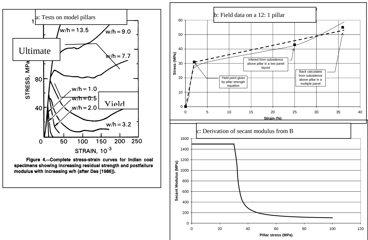
Figure 2 Concepts of pillar behaviour. (a) Laboratory results that show slender pillars ( w/h < 3.2 ) failing and shedding load, and squat pillars ( w/h > 7.7 ) yielding and then work hardening (b) application of laboratory concepts to subsidence in the Southern Coalfield (c) derivation of the secant modulus implied by (b).
