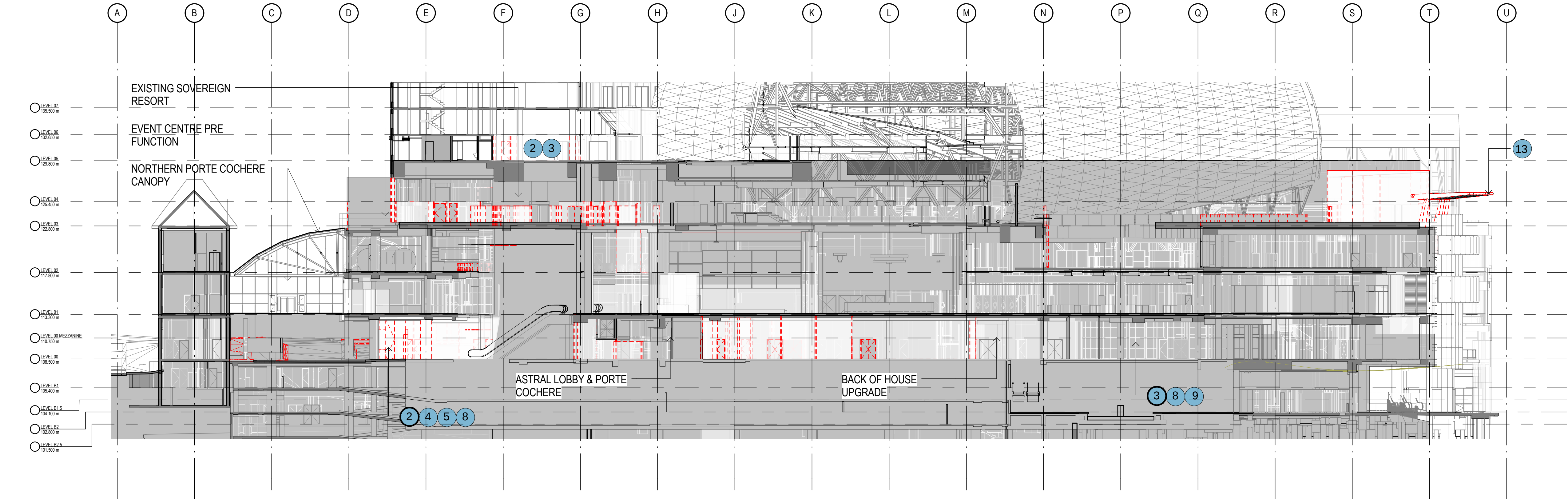
1 SECTION J - EXISTING & DEMOLITION 1: 250
