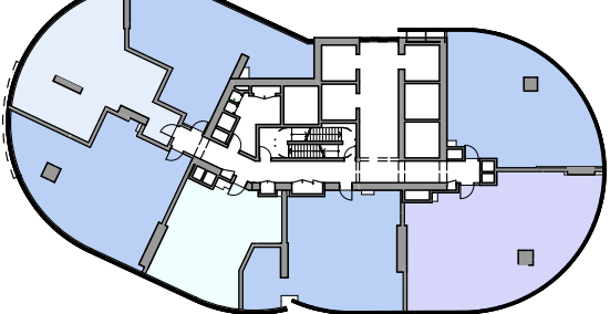
Level 29-39 A21-30
