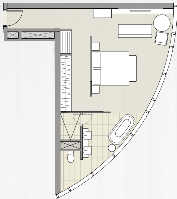
Module C — Corner Executive — 47sqm NLA — 1:100
