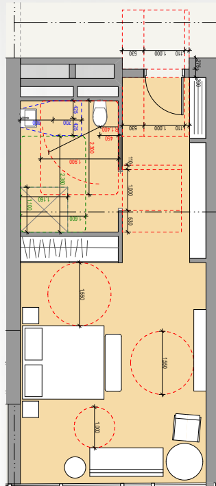
Adaptable / Universal Design Hotel Module — King — 45sqm NLA — 1:100
