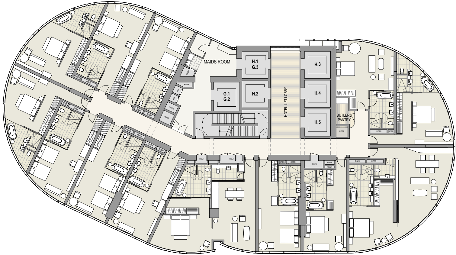
Typical Hotel Plan _ Level 46-58 / H5-H17
