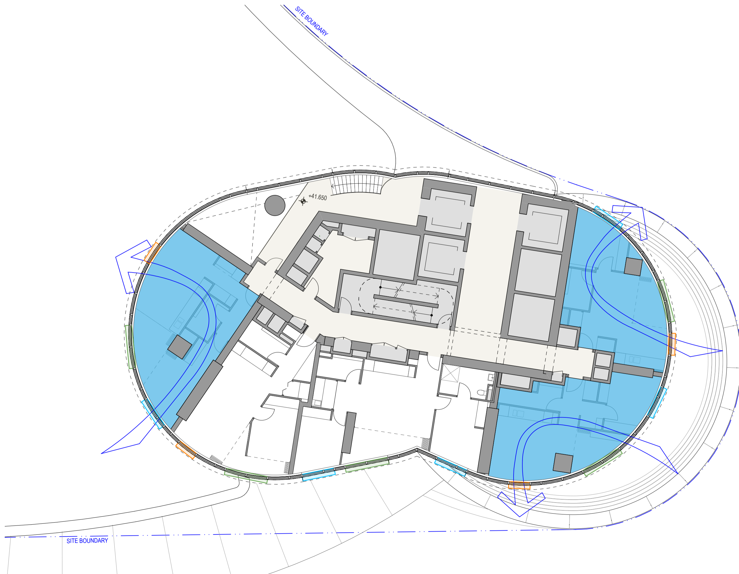
3 PLAN LEVEL 08 A1 1:150
