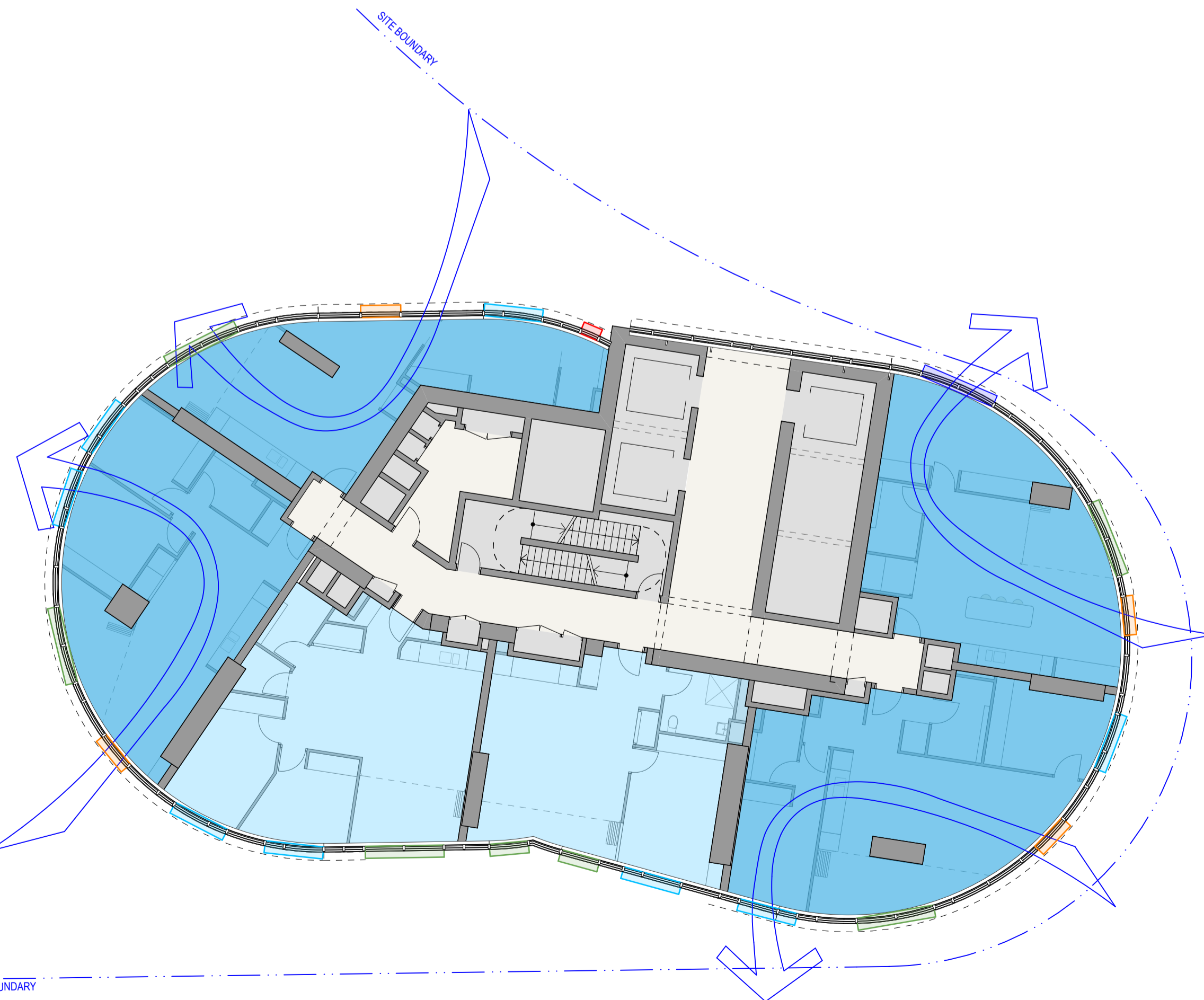
1 PLAN LEVEL 15 A7 1:150 GOOD VENTILATION - 100% (Above Level 09)
