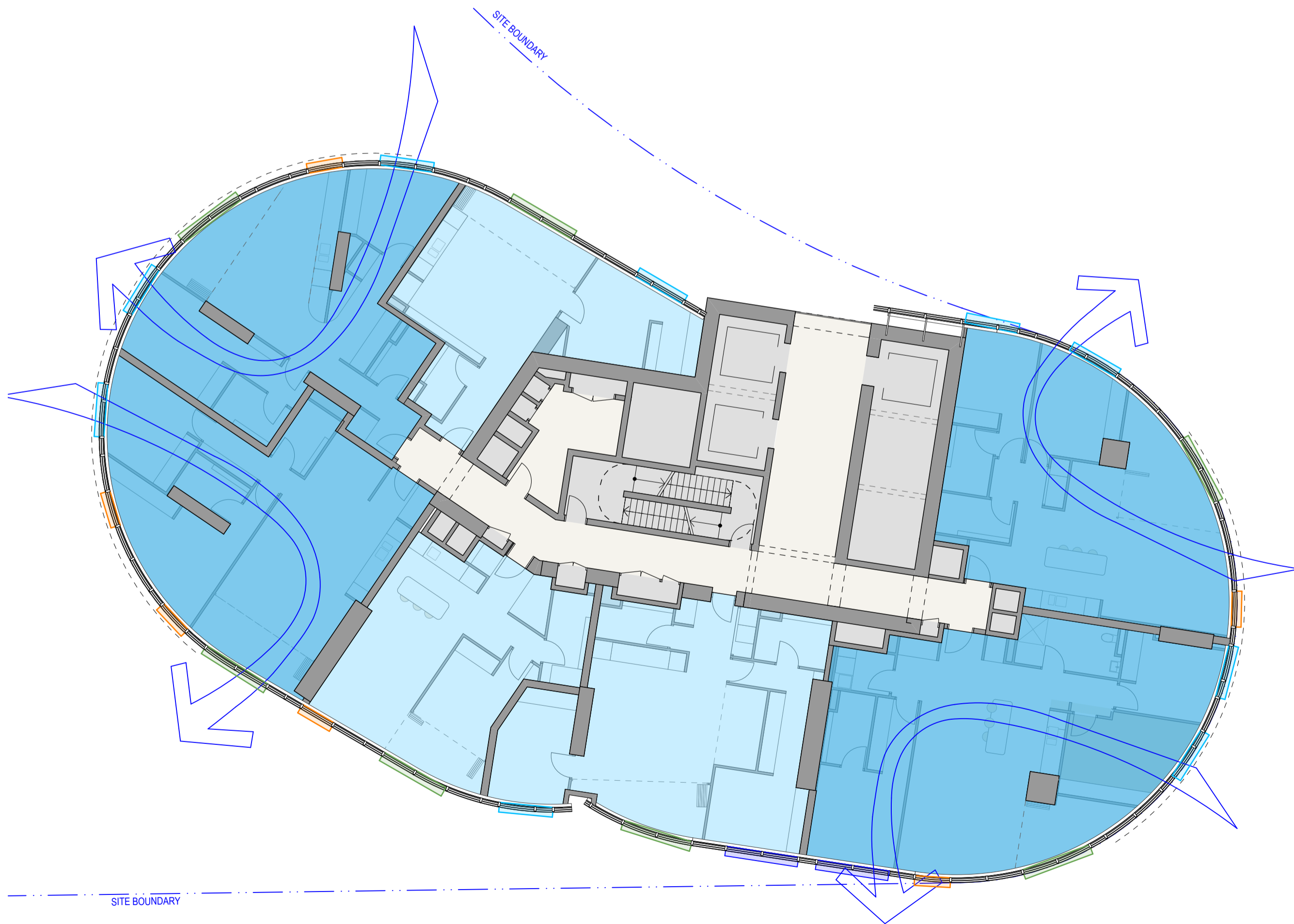
1 PLAN LEVEL 23 A15 1:150 GOOD VENTILATION - 100% (Above Level 09)
