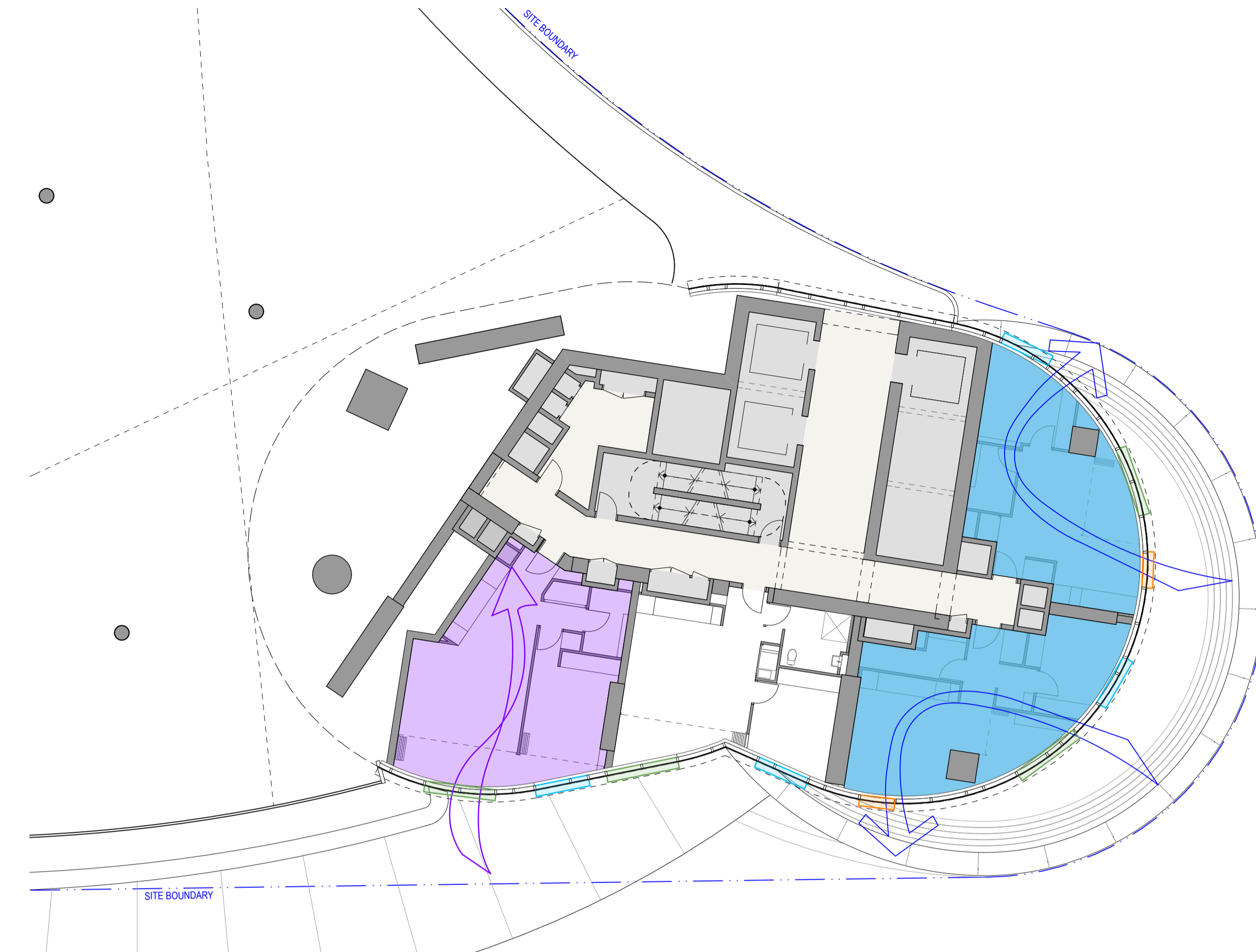
2 PLAN LEVEL 06 A0 1:150
