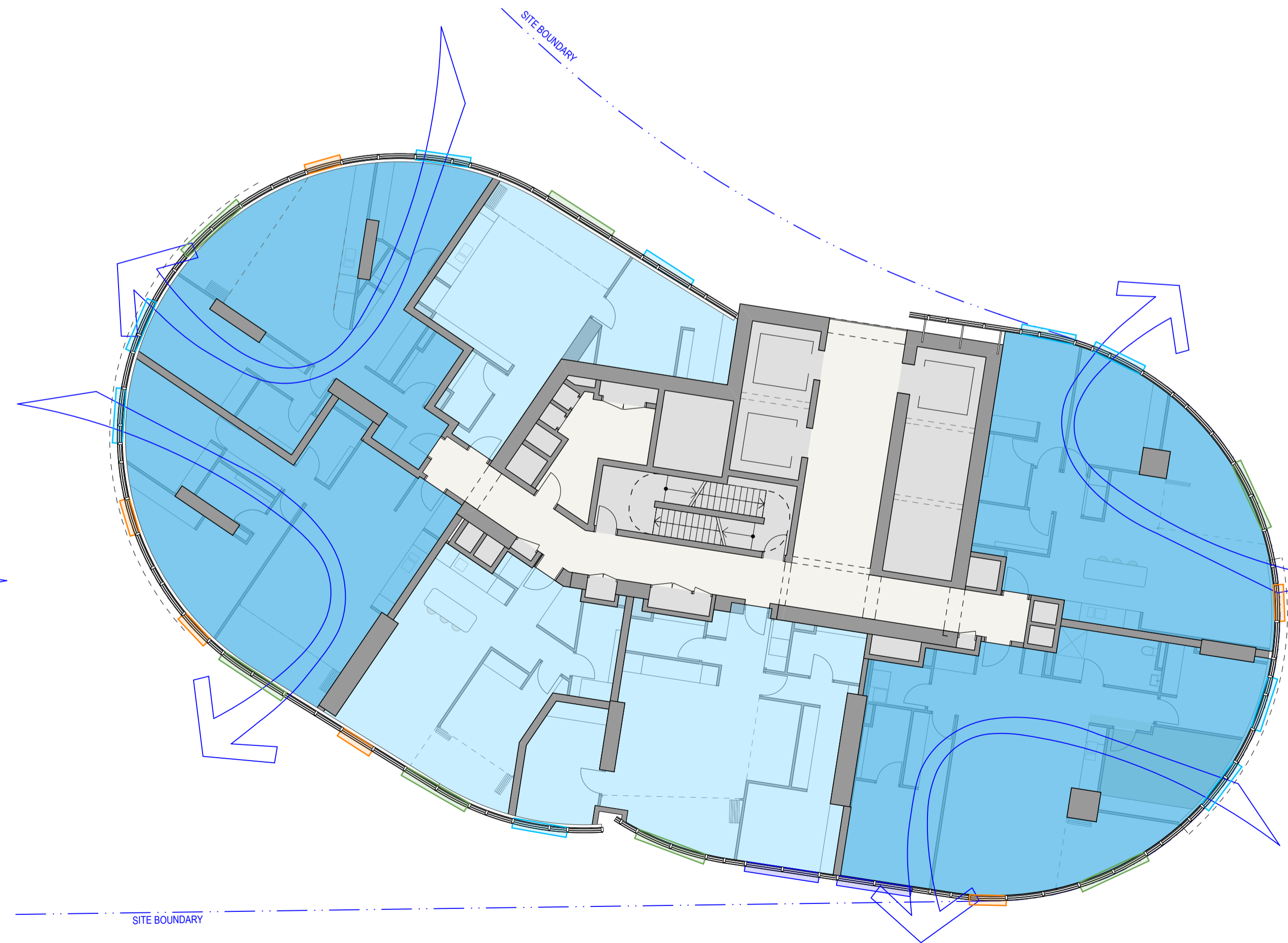
2 PLAN LEVEL 24 A16 1:150 GOOD VENTILATION - 100% (Above Level 09)
