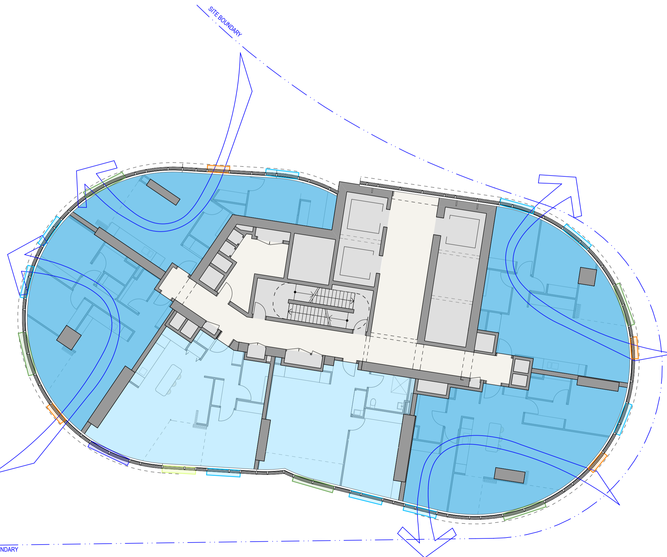
2 PLAN LEVEL 16 A8 1:150 GOOD VENTILATION - 100% (Above Level 09)
