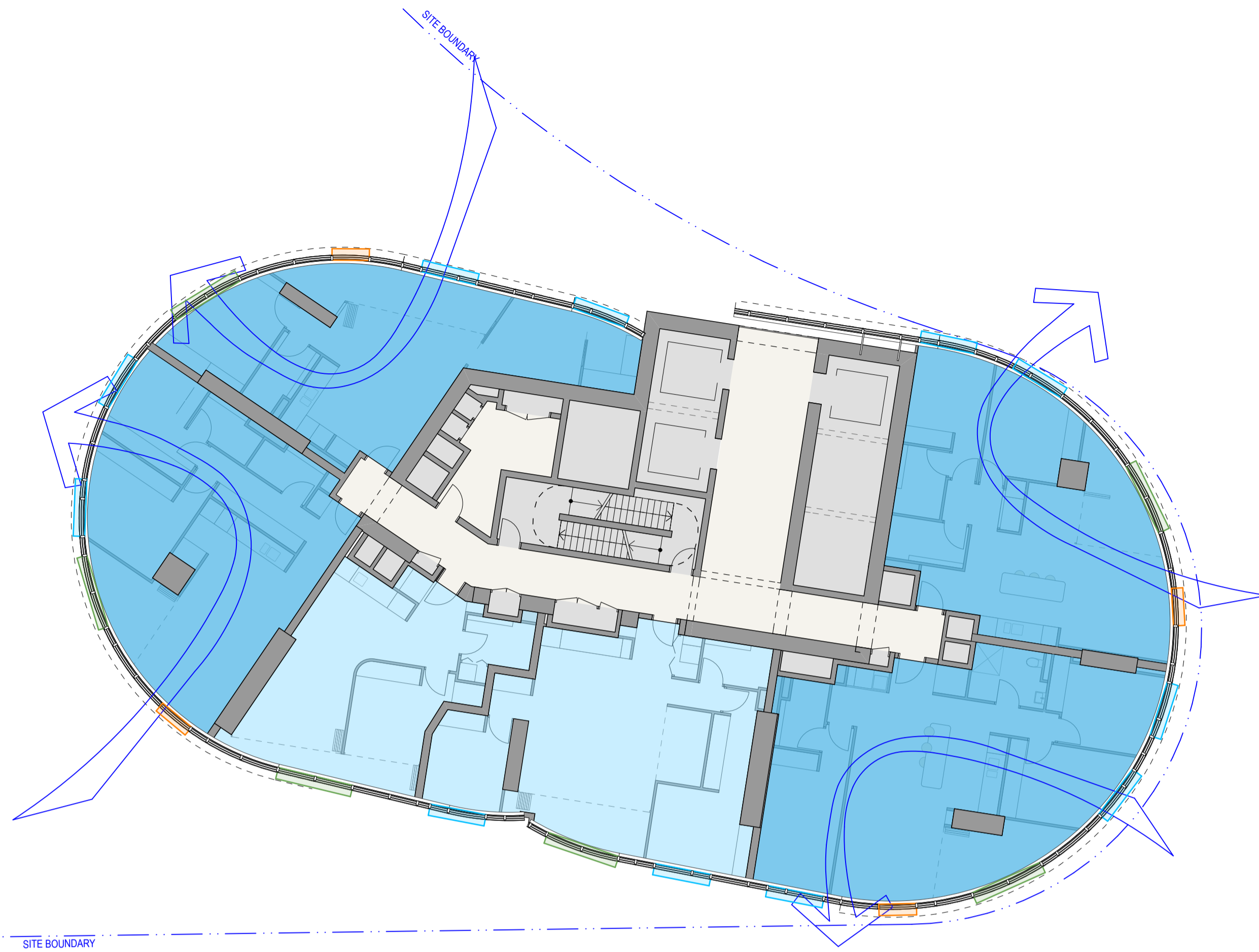
2 PLAN LEVEL 20A12 1:150
