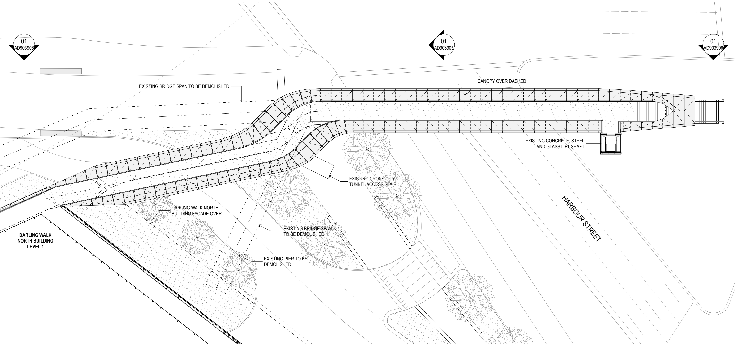
1 GENERAL ARRANGEMENT PLAN 1:250
