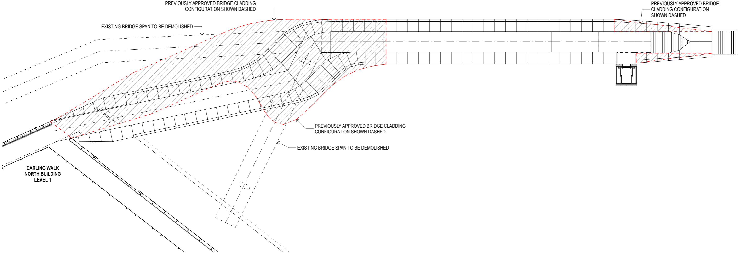
1 COMPARISON PLAN 1:250
