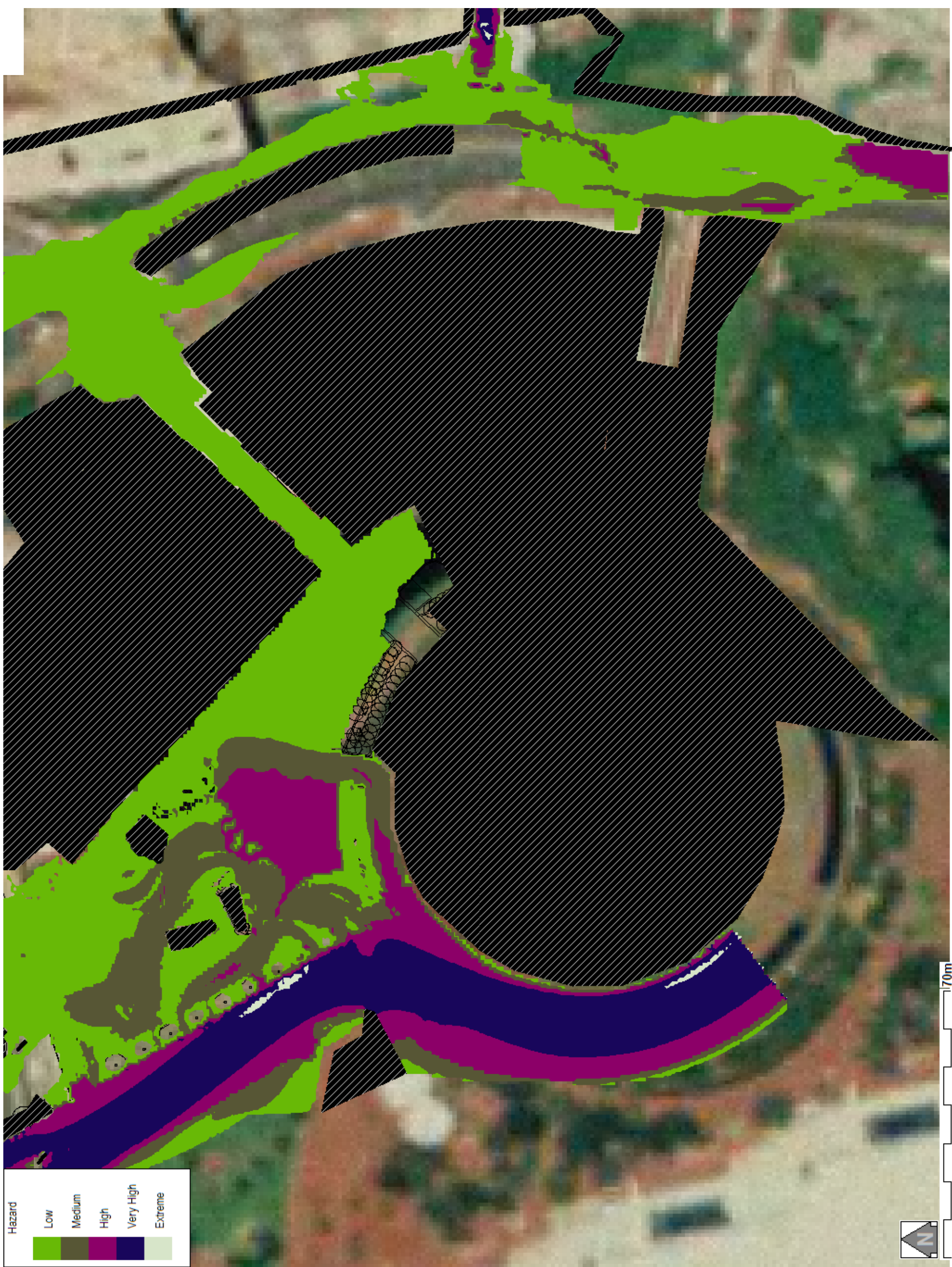
FLOOD STUDY ADDENDUM 3 FLOOD VELOCITY DEPTH PRODUCT AT TUMBALONG PARK PROPOSED 100 YEAR ARI 60 MIN STORM
