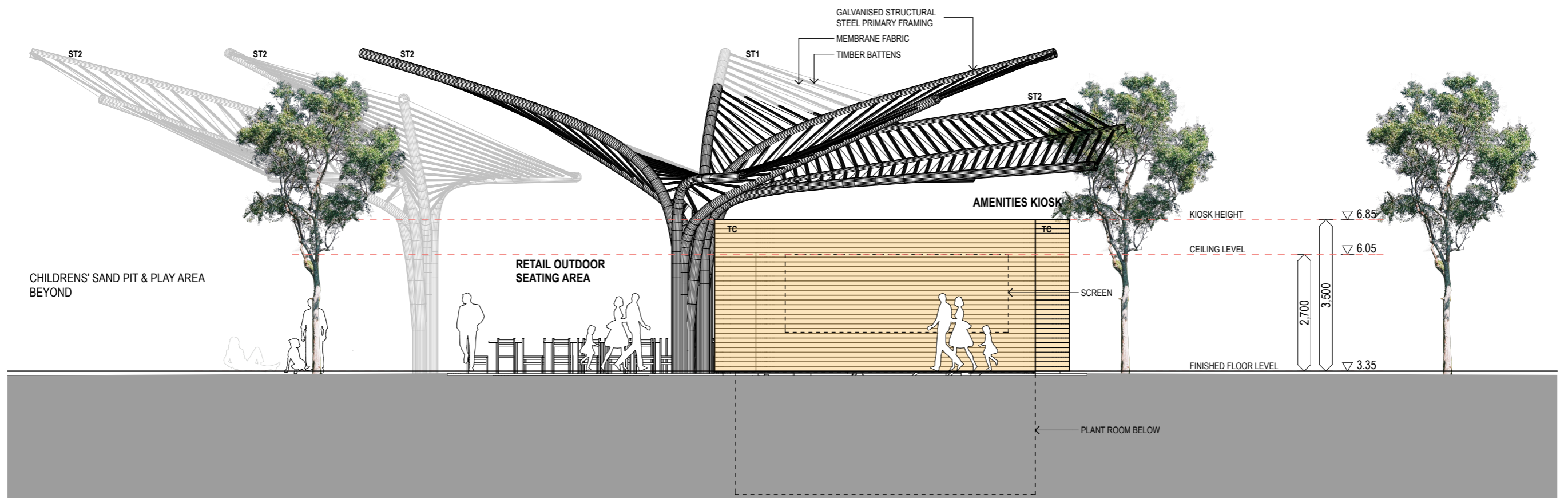
Section 3 1:100
