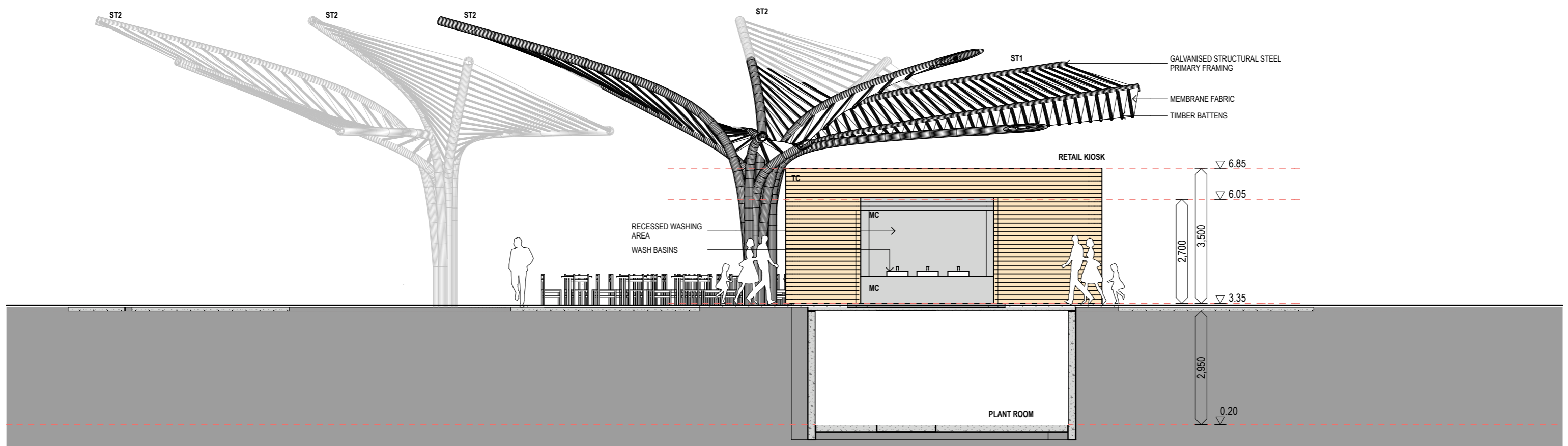
Retail Kiosk Corridor Elevation 1:100
