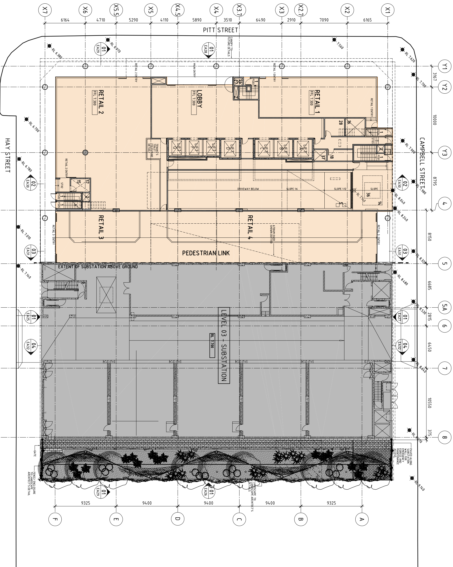
FLOOR PLAN - GROUND LEVEL
