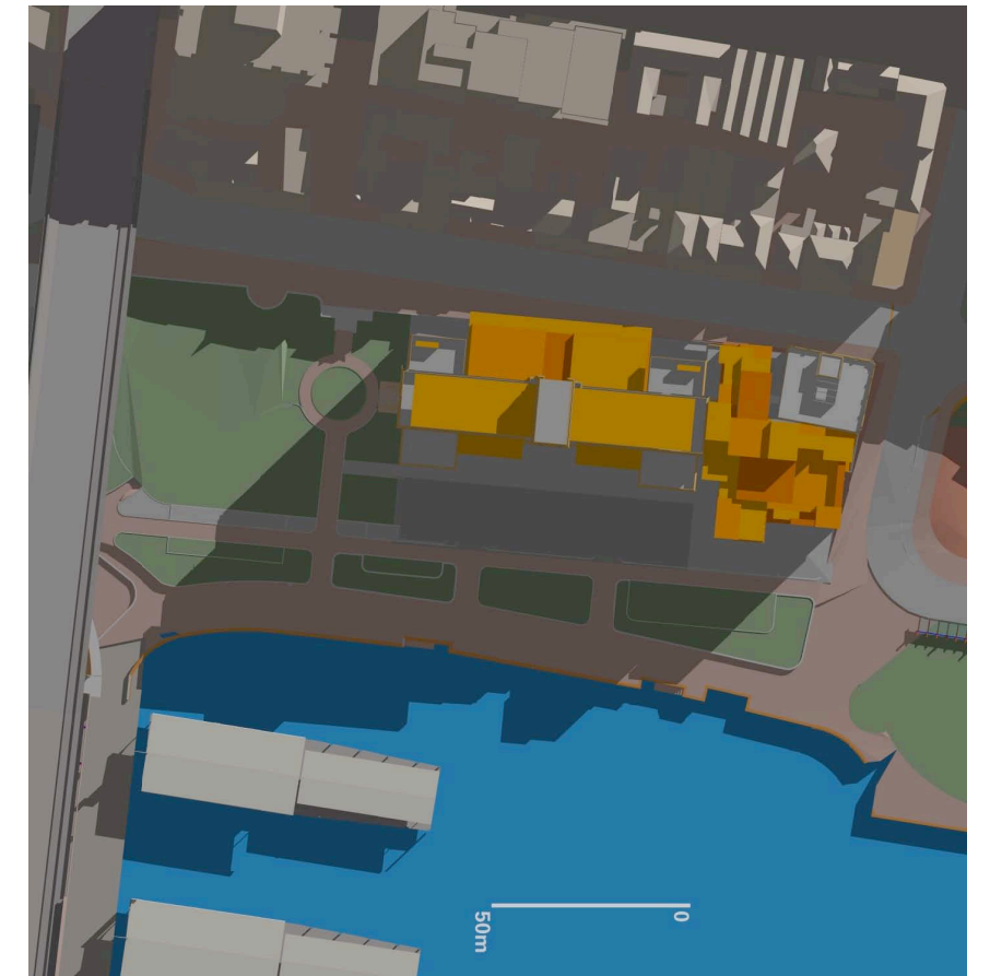
PROPOSED - 21 JUNE 3 P.M.
