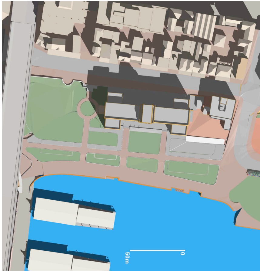
EXISTING - 21 MARCH 9 A.M.
