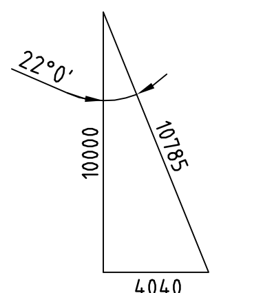
SKIEW DIAGRAM NOT TO SCALE
