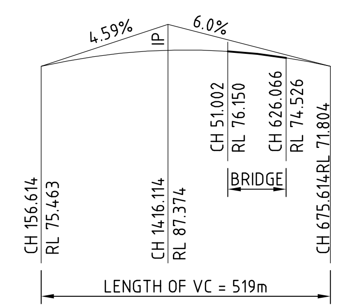
VERTICAL ALIGNMENT DIAGRAM NOT TO SCALE
