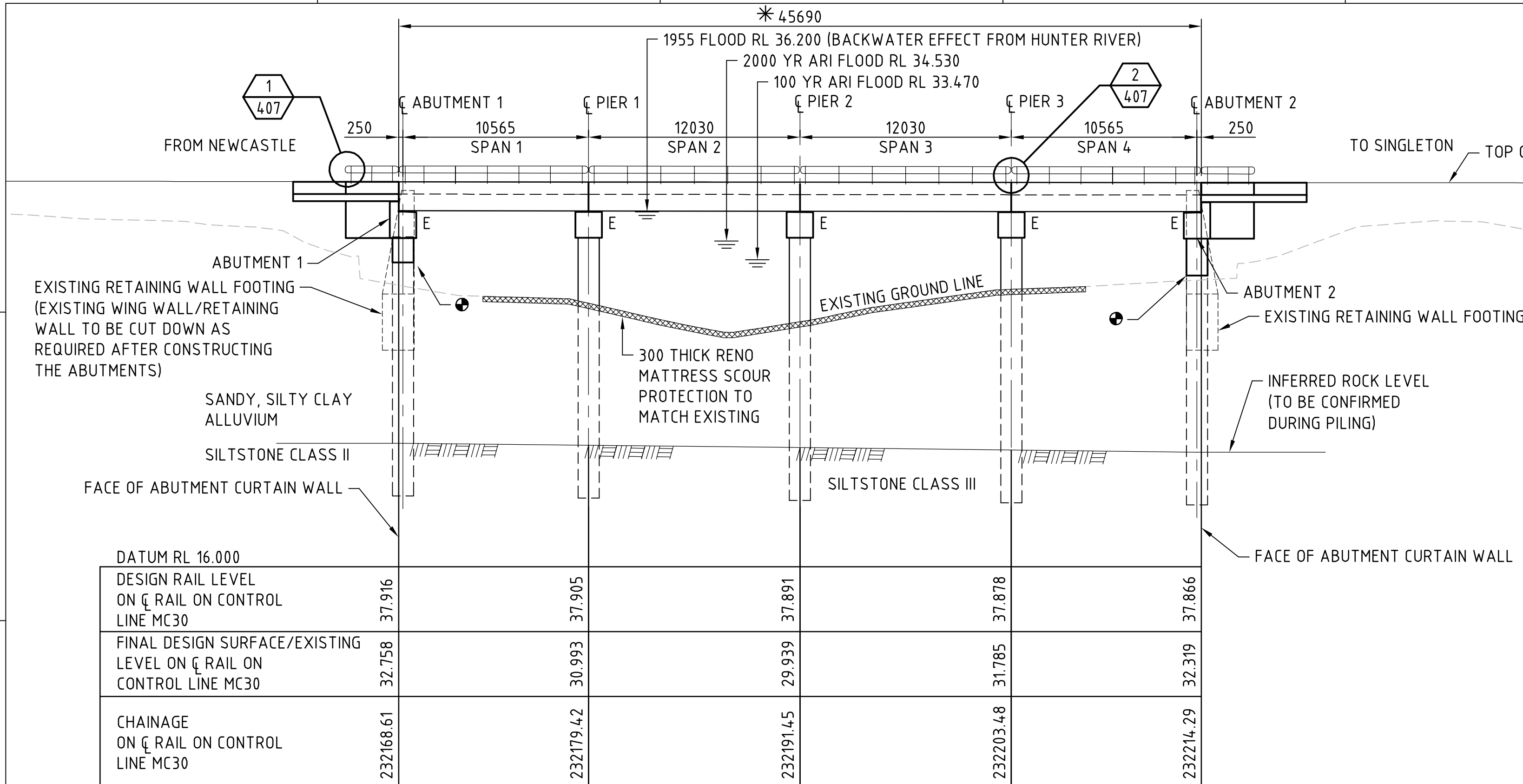
ELEVATION SCALE 1:200
