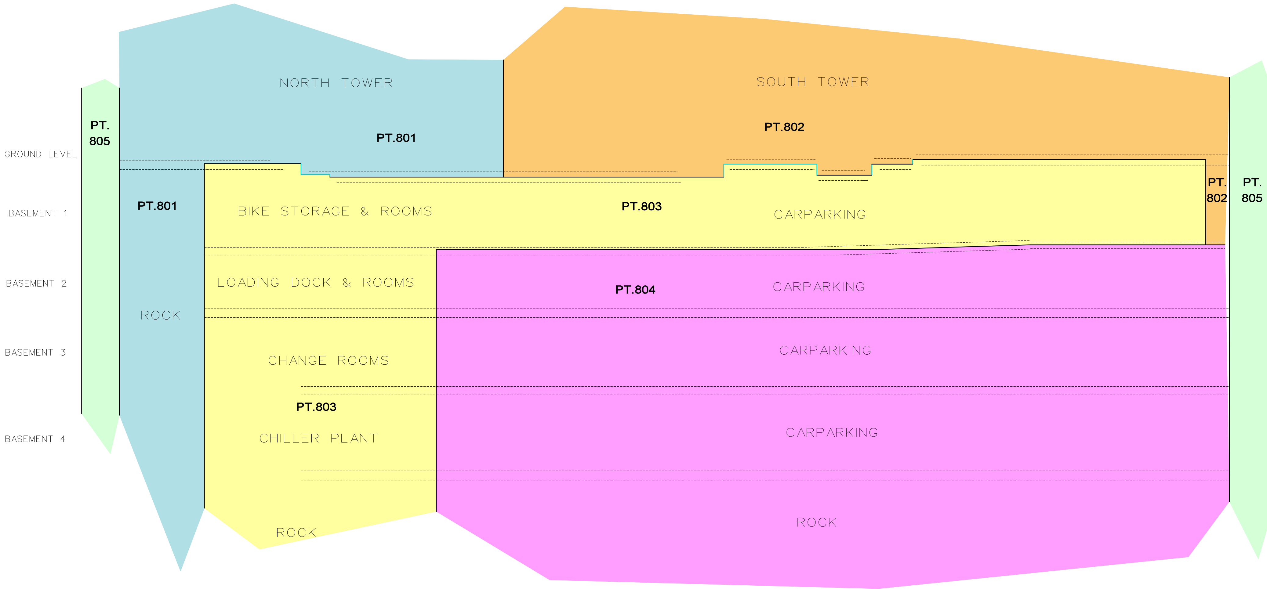
SECTION "Q" - "Q"
