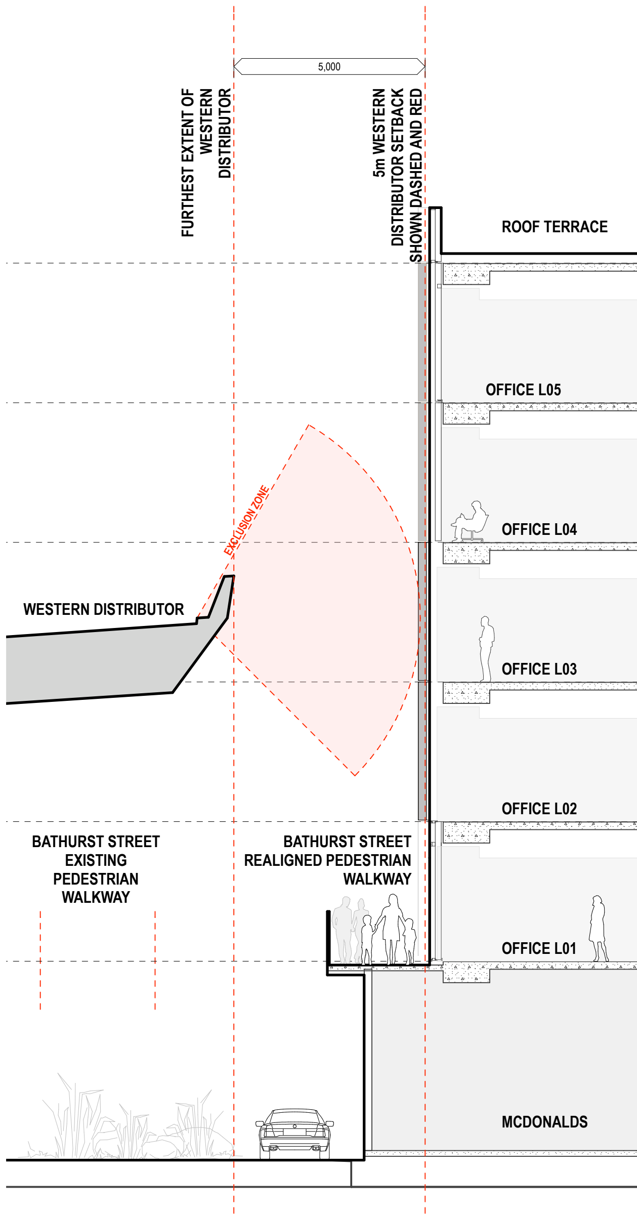
SECTION THROUGH WALKWAY
