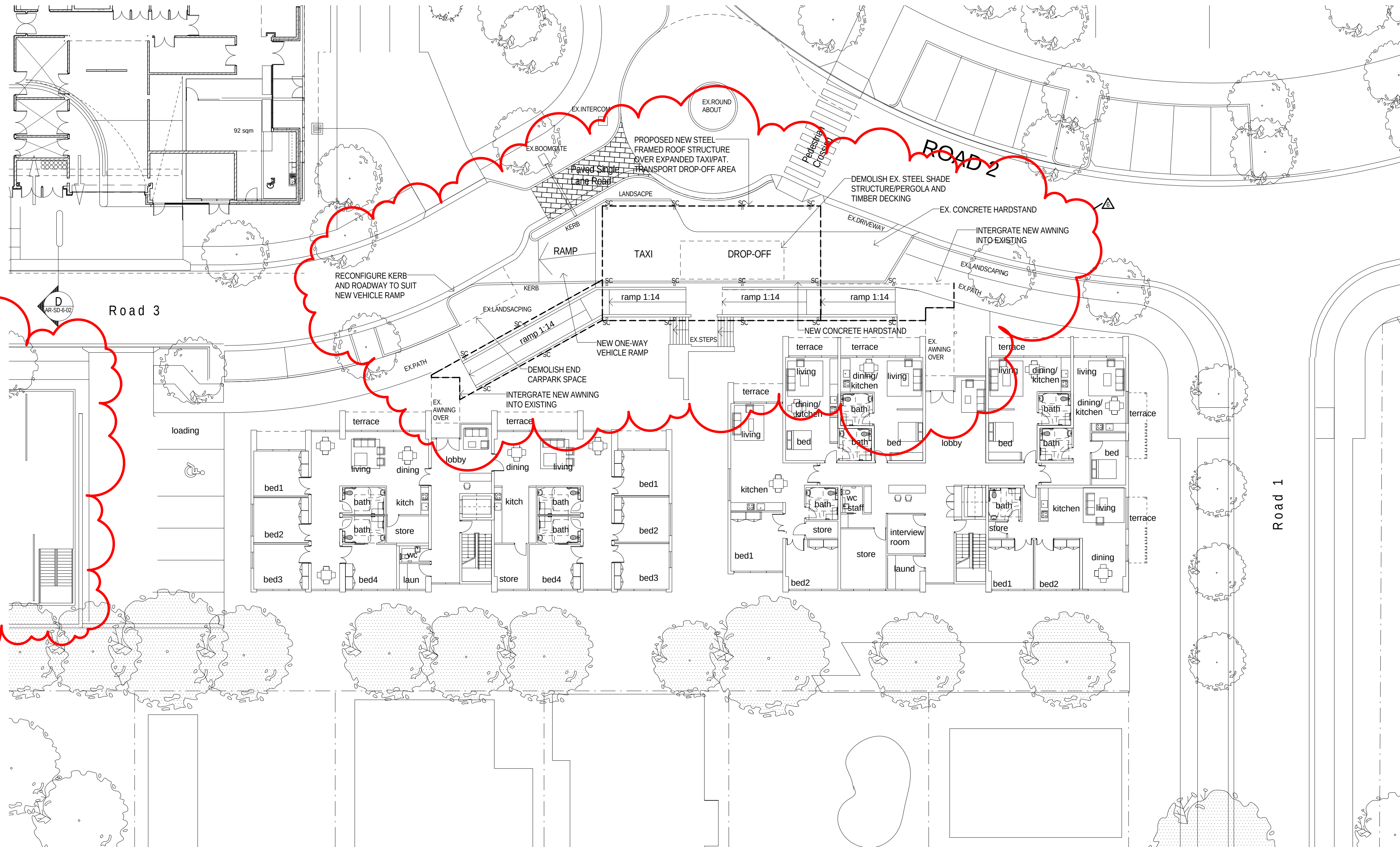
1 GROUND FLOOR PLAN 1:200
