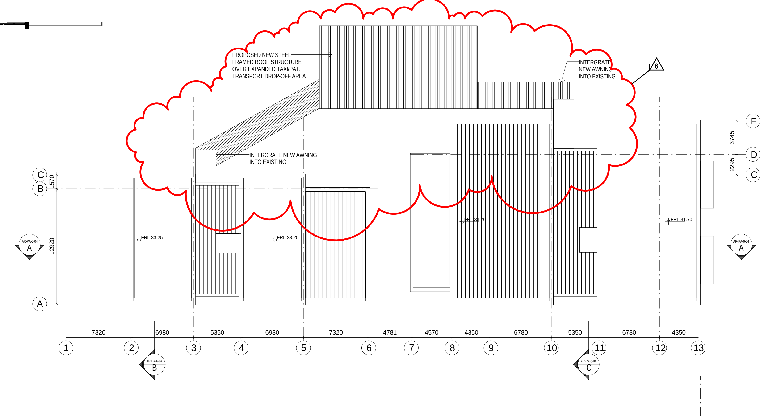
3 ROOF PLAN 1:200
