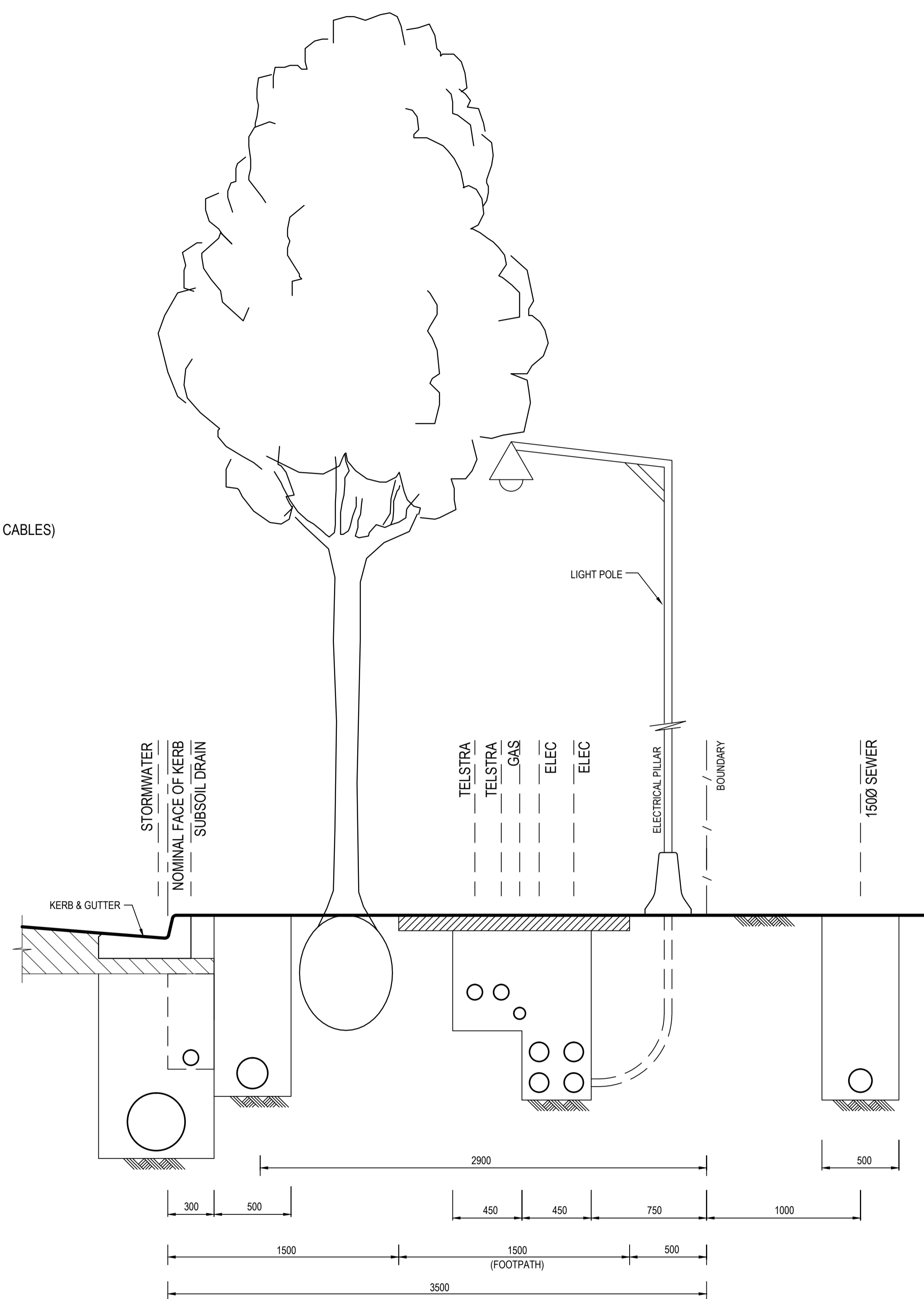
TYPICAL FOOTWAY - ROAD 4 NOT TO SCALE
