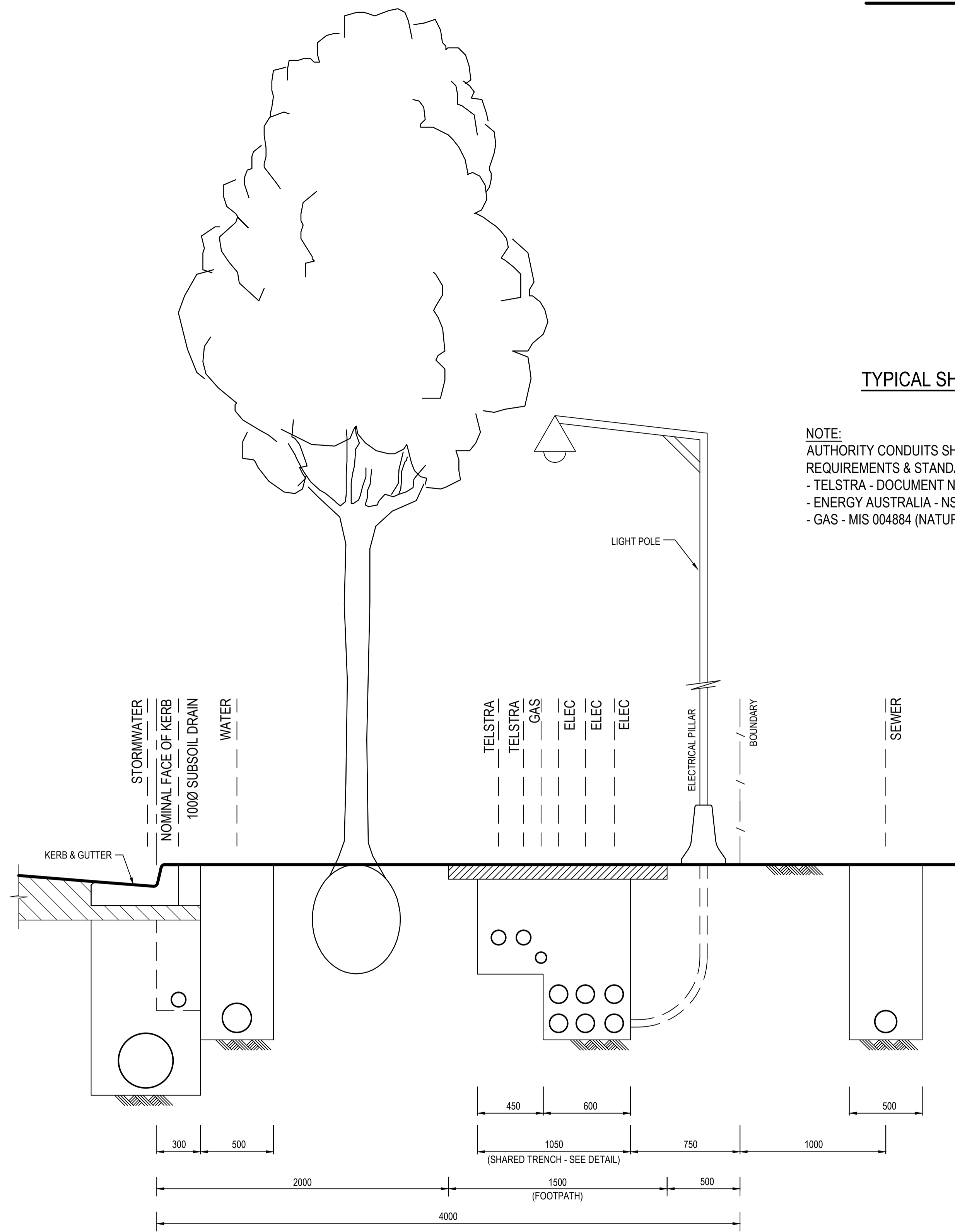
TYPICAL FOOTWAY - ROAD 5 NOT TO SCALE
