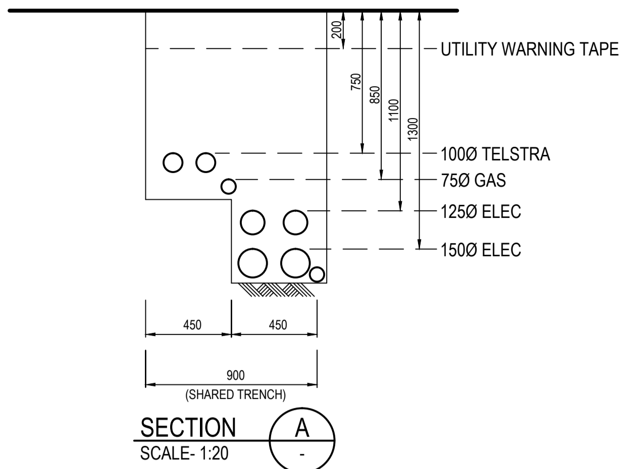
TYPICAL SHARED TRENCH ARRANGMENT
