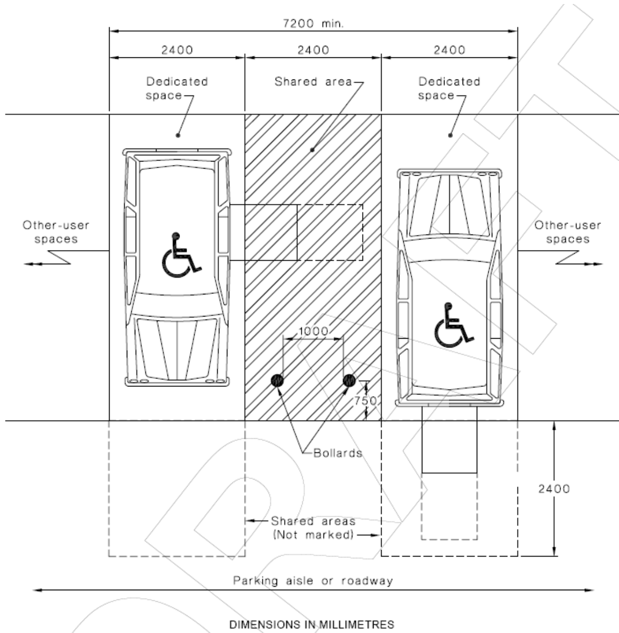
FIGURE 6.3 EXAMPLE OF TWO PARKING SPACES WITH A COMMON SHARED AREA Source: Draft AS2890.6 Parking Facilities - Part 6: Off-street parking for people with disabilities
