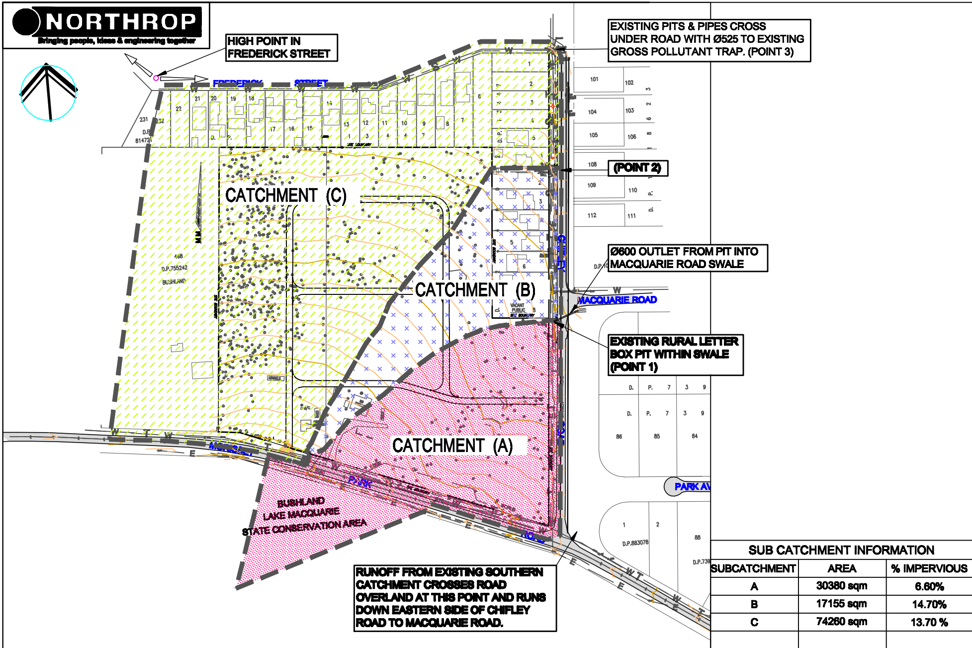
FIGURE 1- Pre-Development catchment plan
