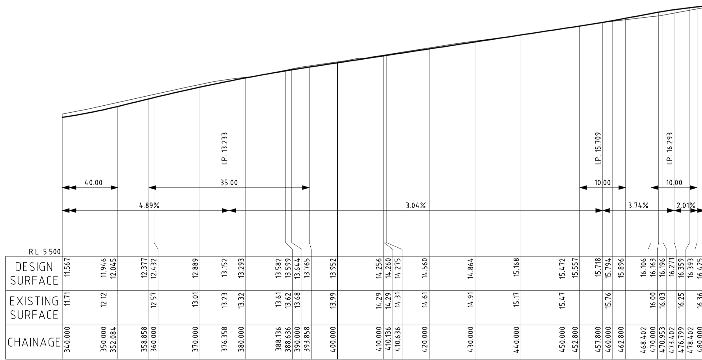
ROAD1 From ch340.000 To ch480.000 Scales: H 1 in500 V 1 in100
