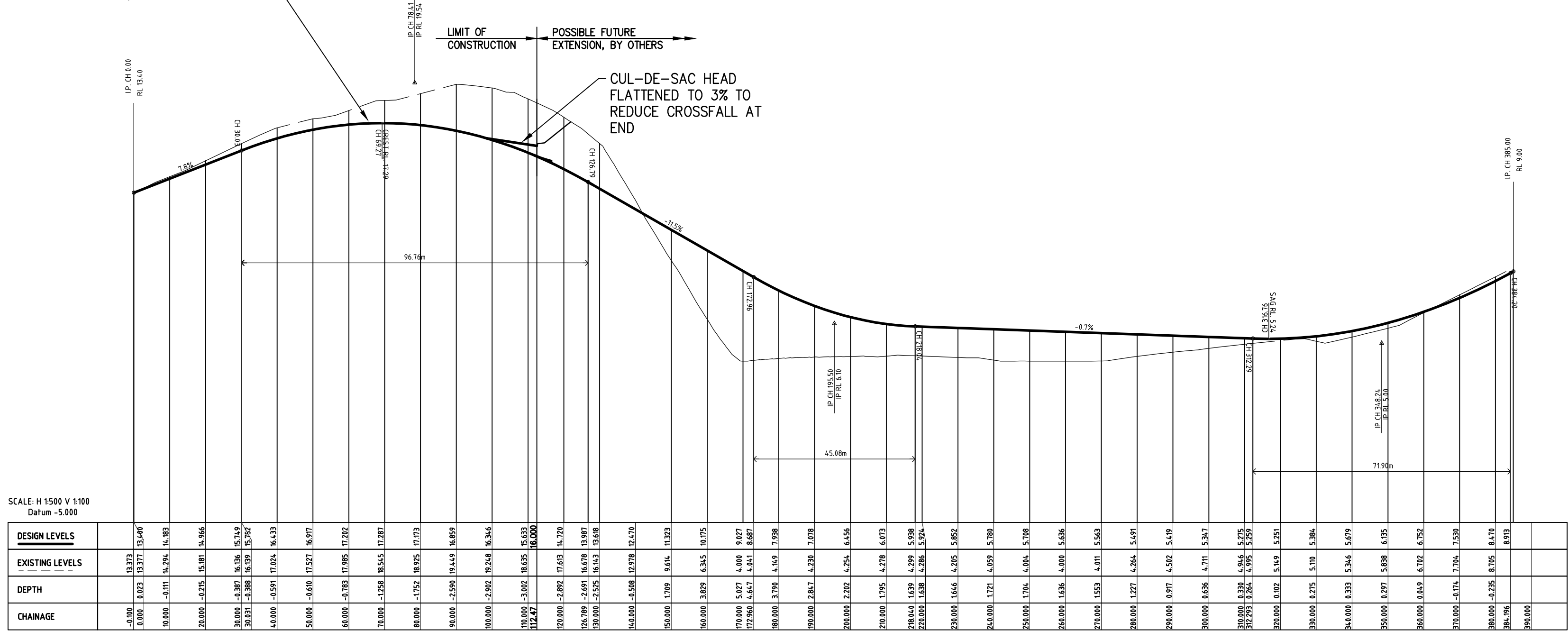
COLLECTOR ROAD LONG SECTION
