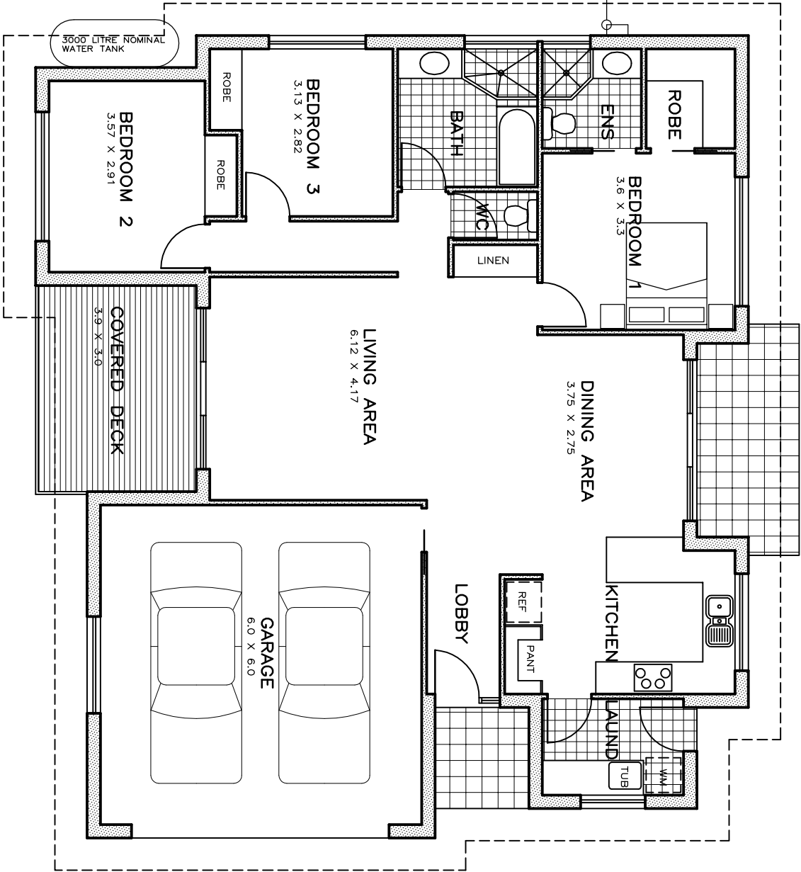
FLOOR PLAN 128.5 SQ. M (EXCLUDING GARAGE) 168.5 SQ. M (INCLUDING GARAGE)
