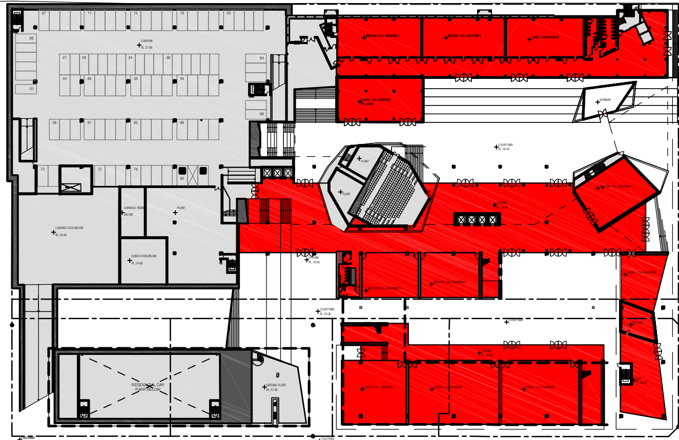
02 GROUND FLOOR
