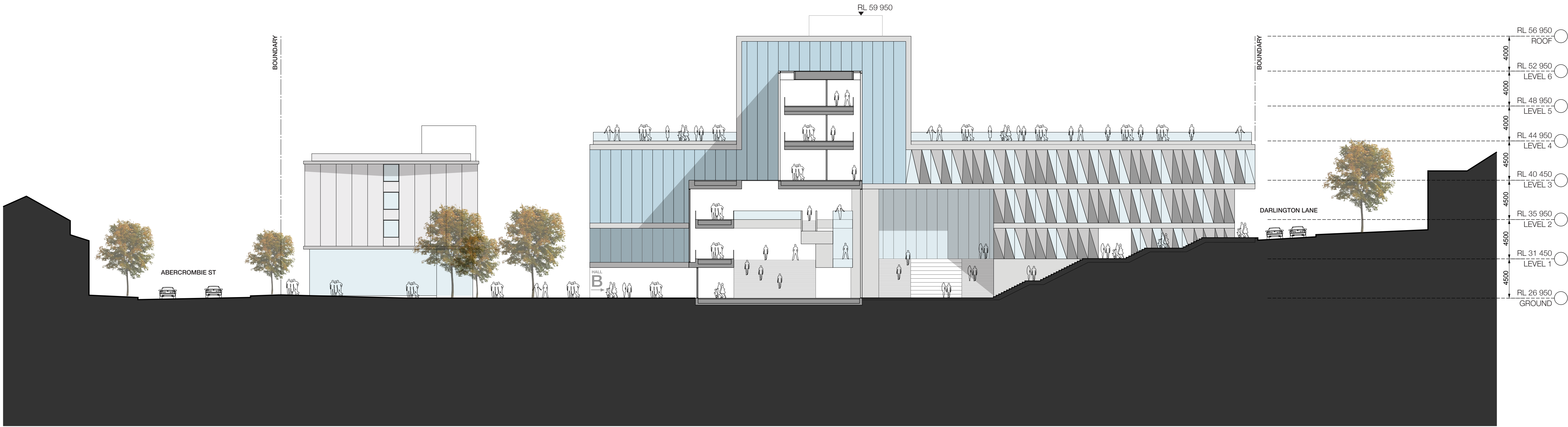
01 SECTION C 1:250 @ A1
