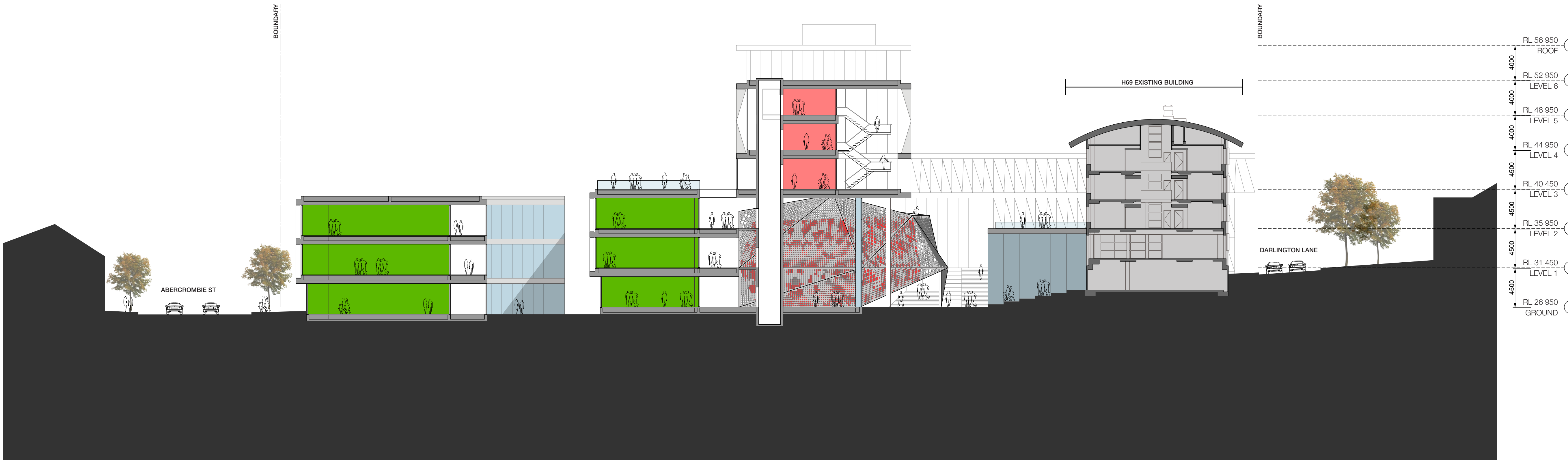
02 SECTION D 1:250 @ A1
