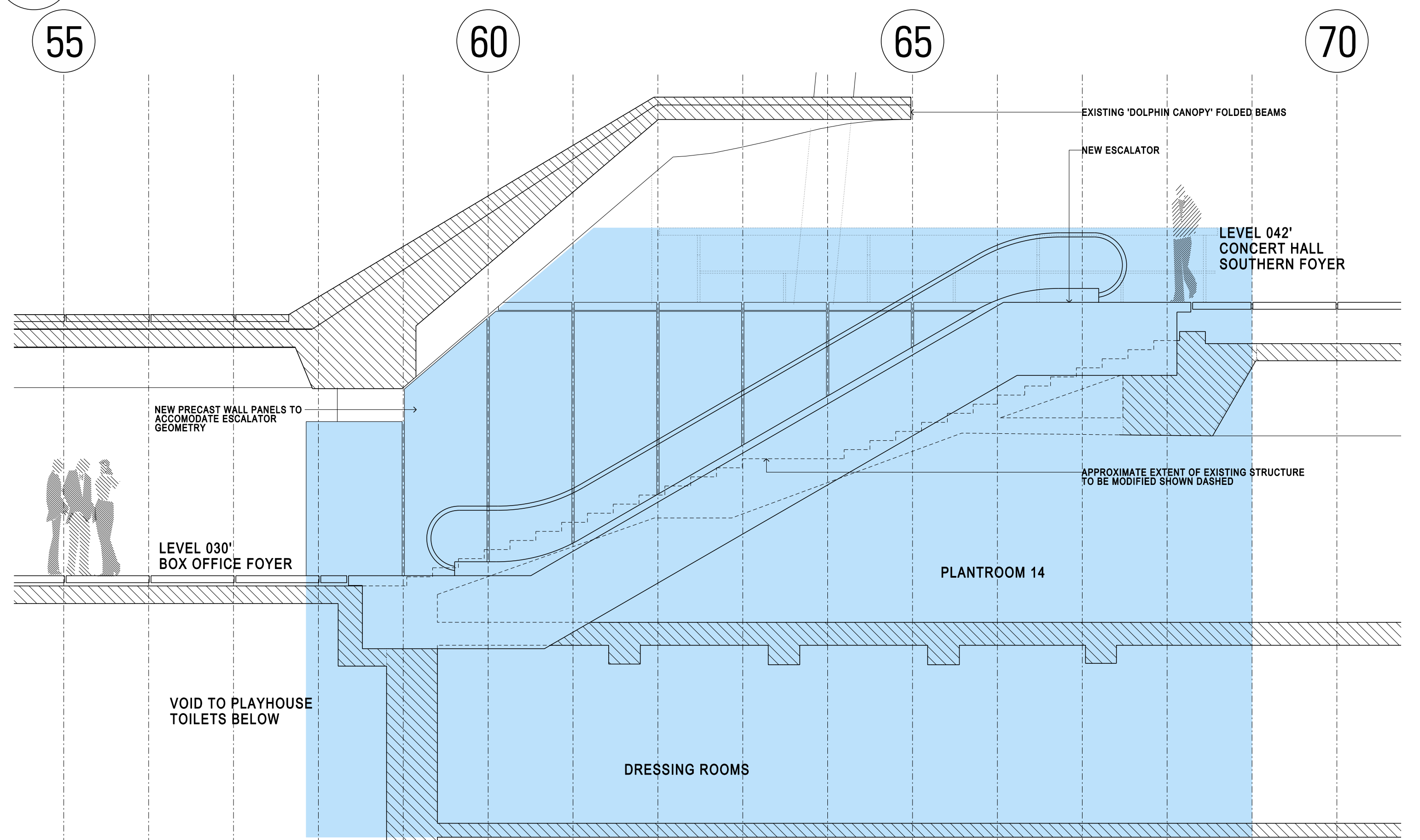
03 SECTION DETAIL: ESCALATOR 02 SCALE 1:50
