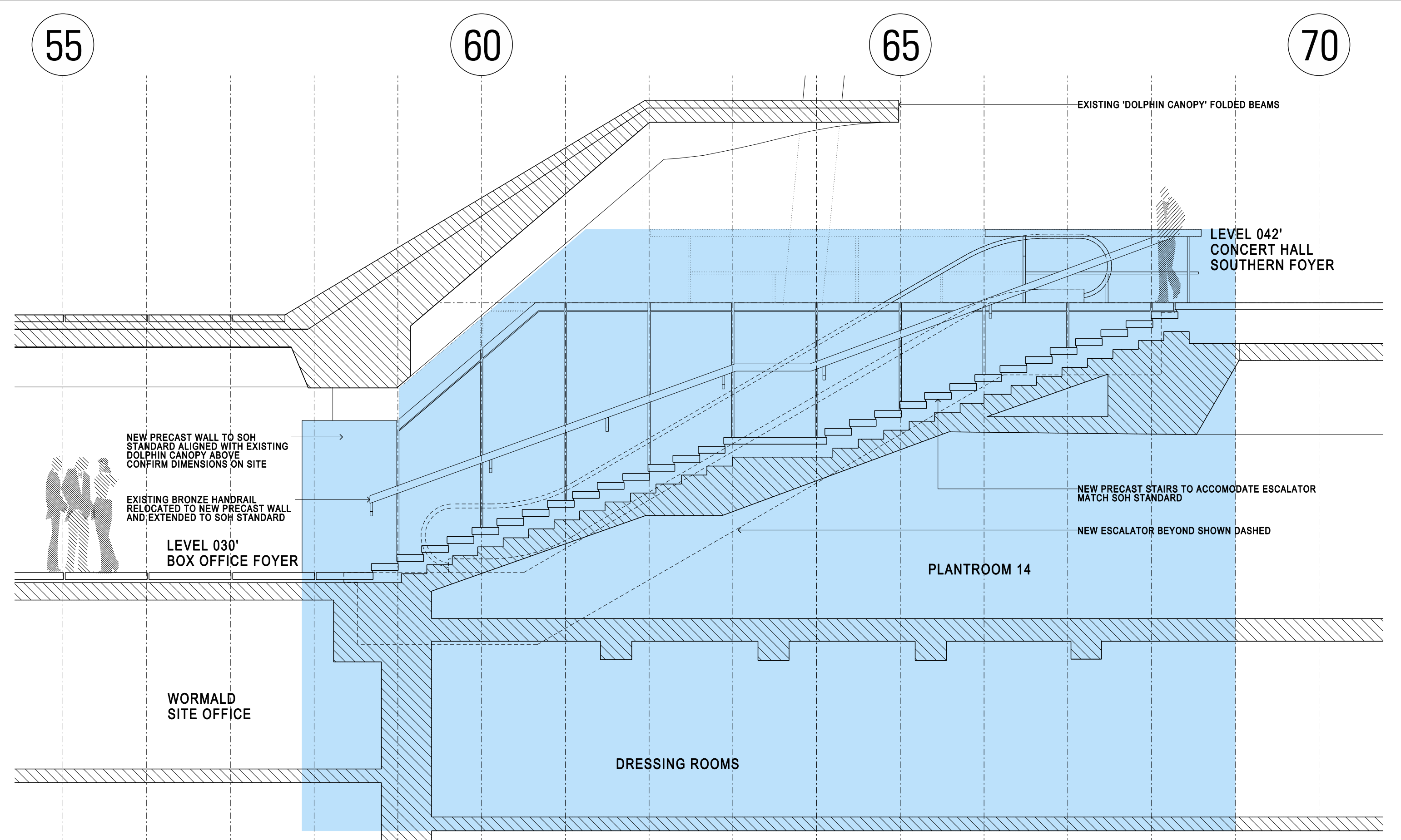
02 SECTION DETAIL: STAIRS TO SOUTHERN FOYER SCALE 1:50
