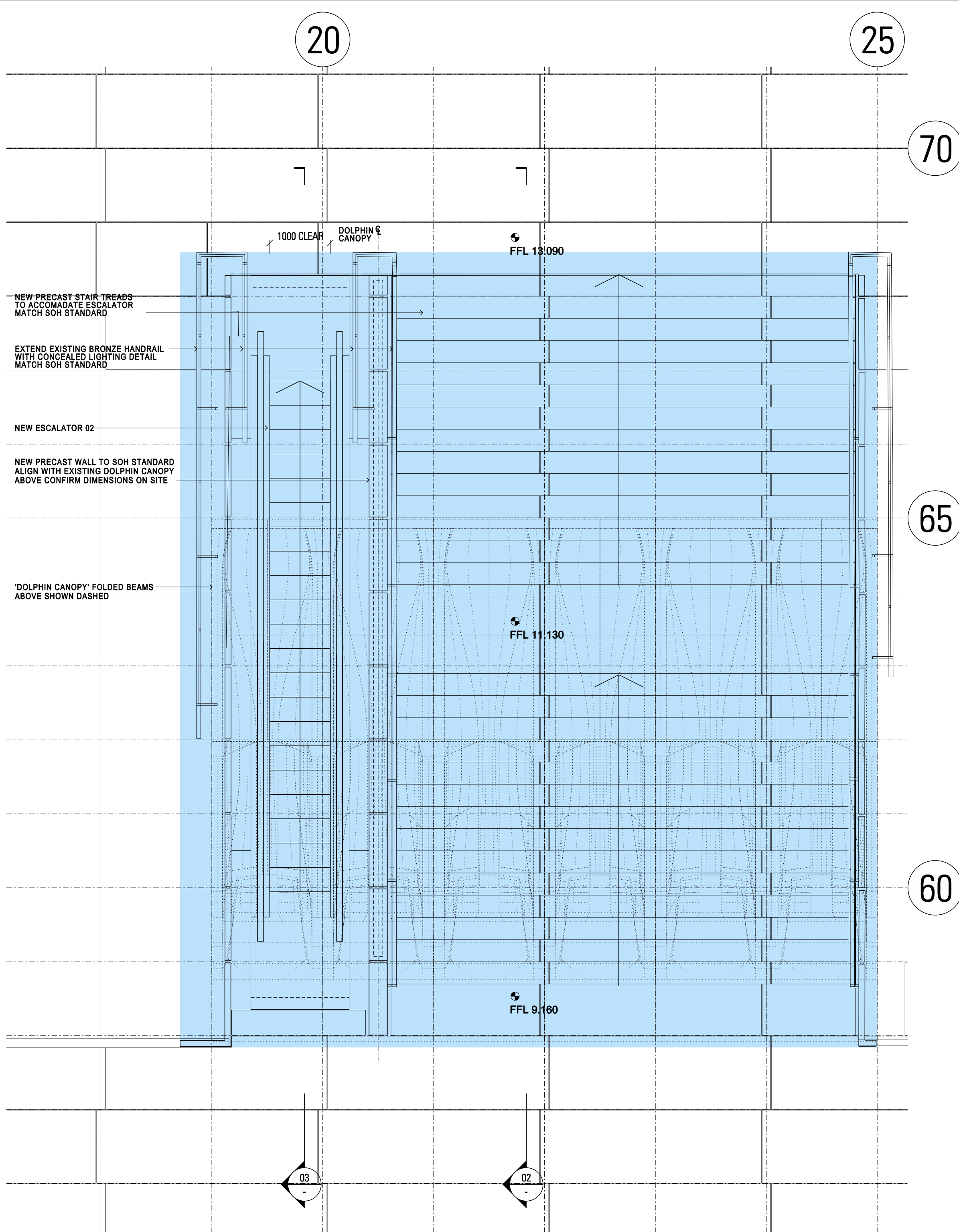
01 PLAN DETAIL: ESCALATOR 02 SCALE 1:50
