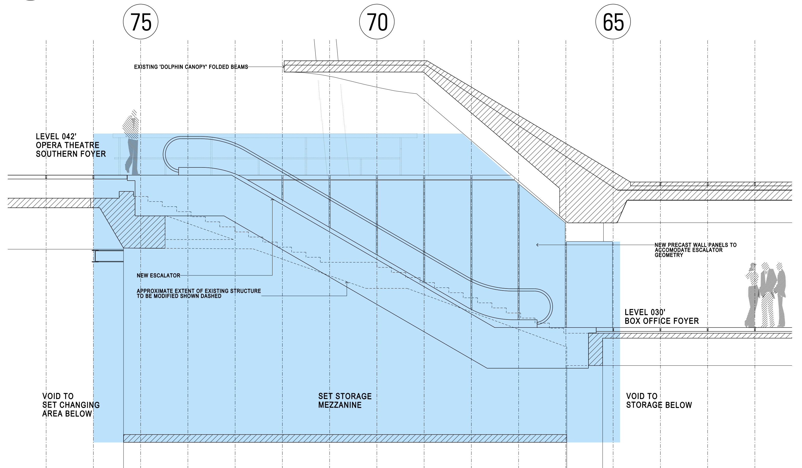
03 SECTION DETAIL: ESCALATOR 01 SCALE 1:50
