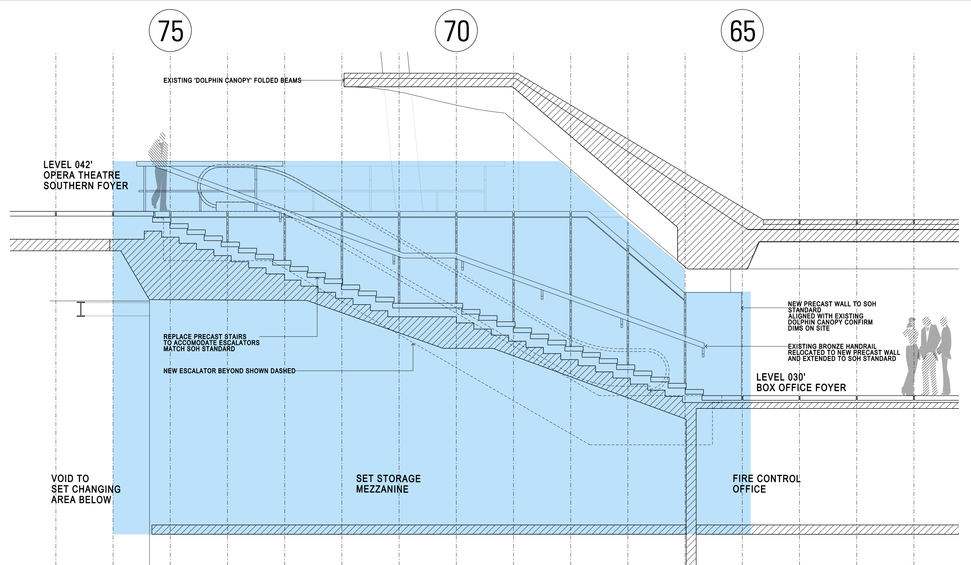
02 SECTION DETAIL: STAIRS TO SOUTHERN FOYER SCALE 1:50
