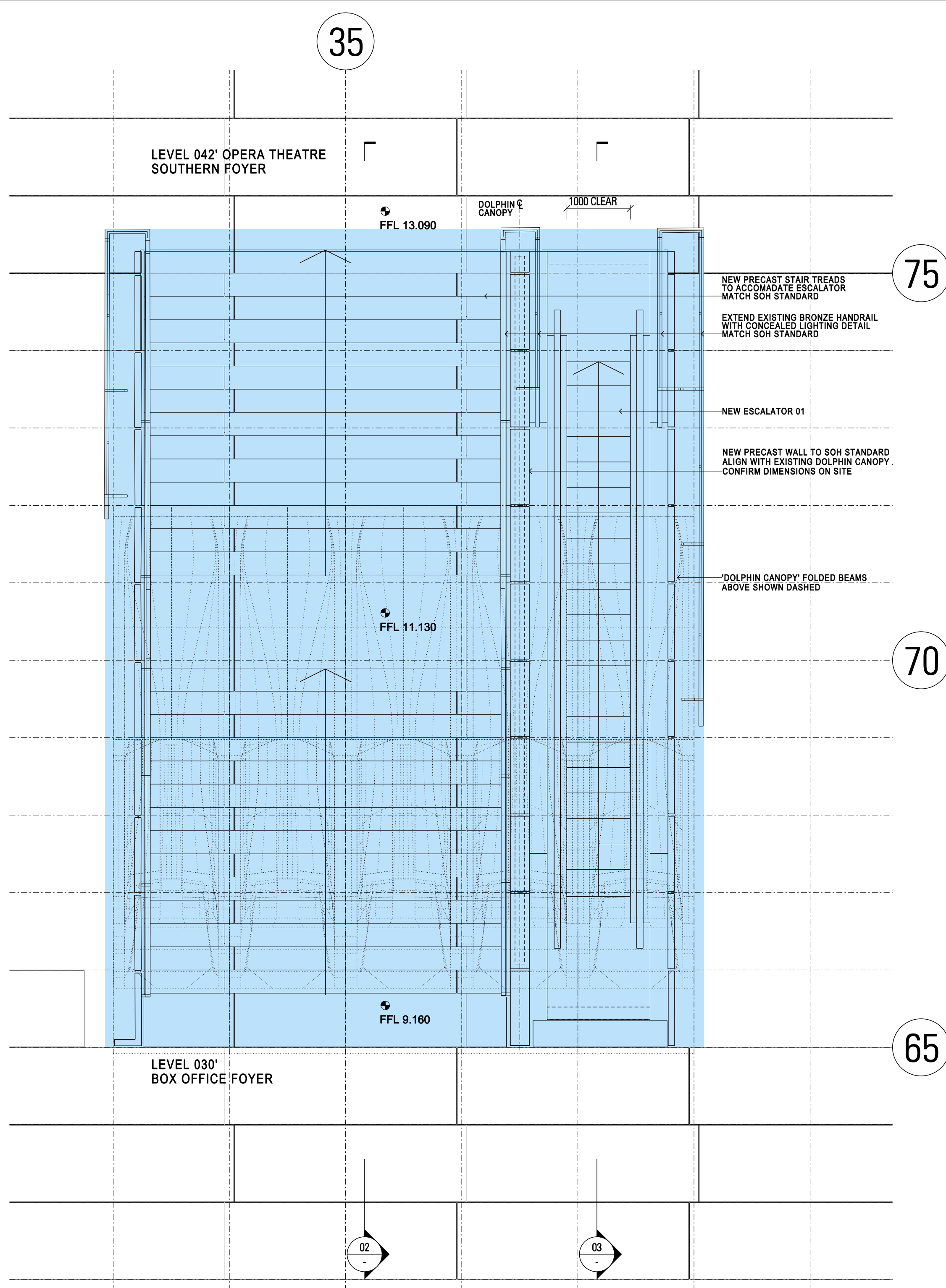
01 PLAN DETAIL: ESCALATOR 01 SCALE 1:50
