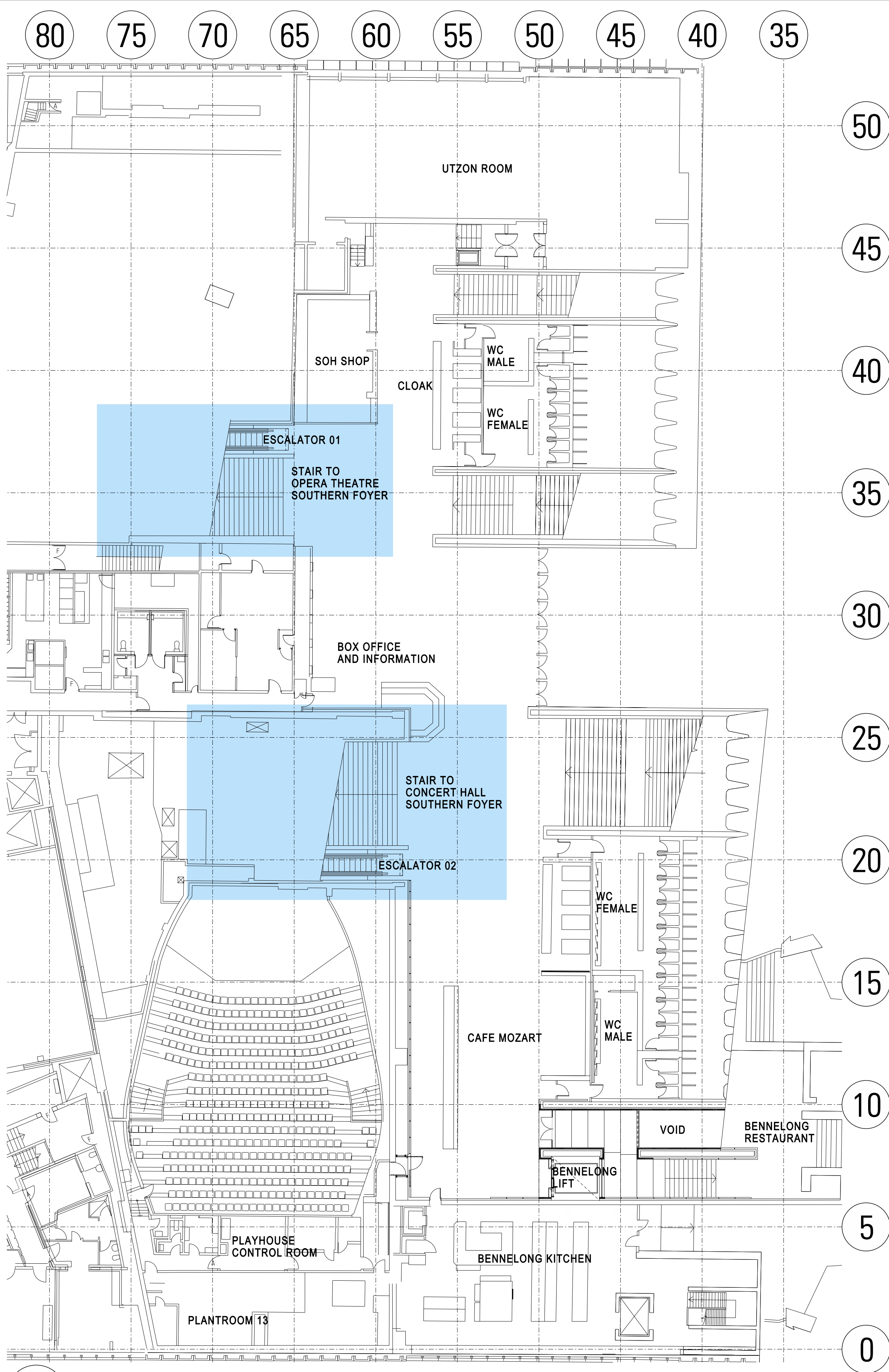
01 LEVEL 030' ESCALATORS LOCATION PLAN SCALE 1:200
