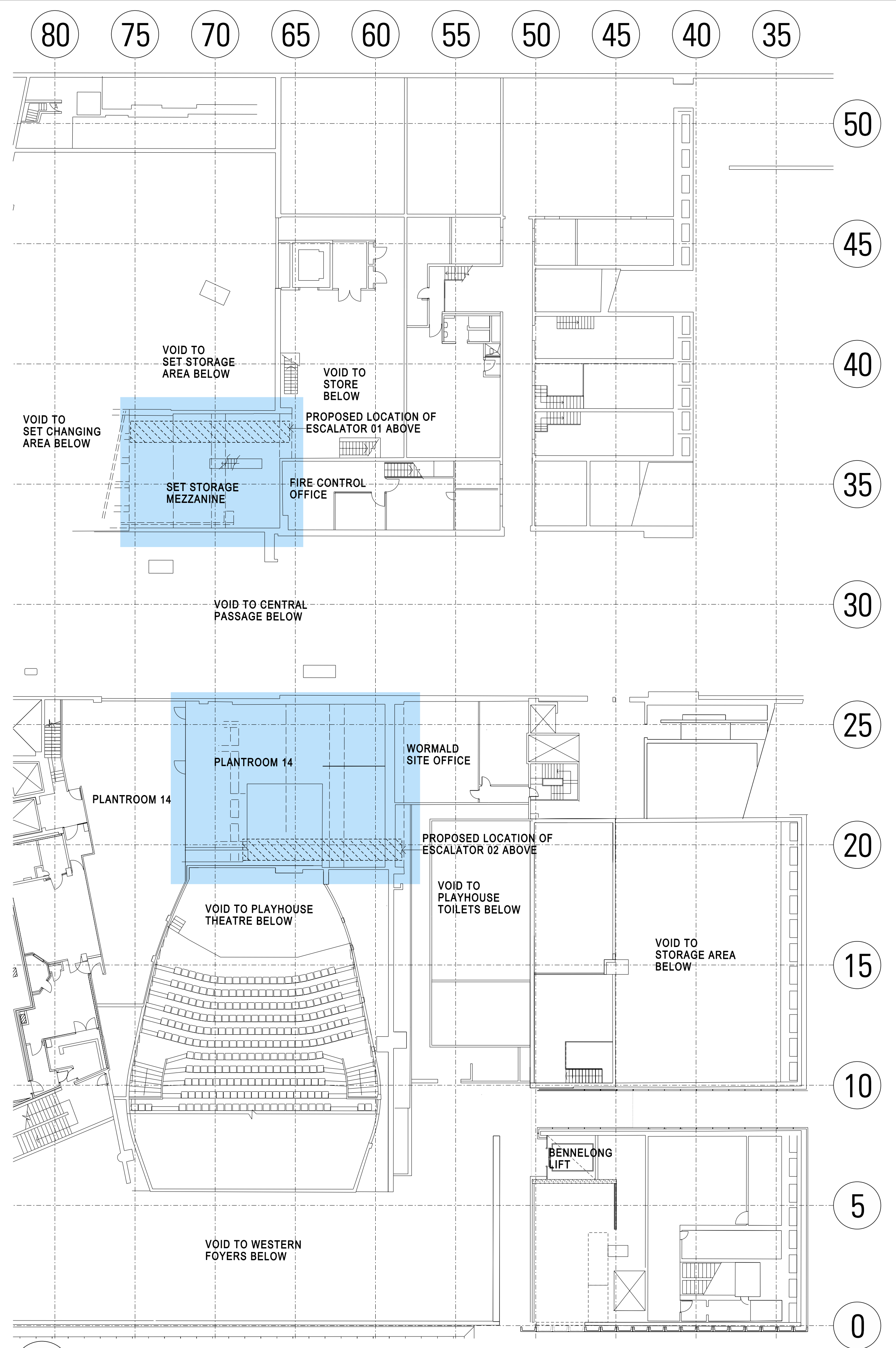
02 LEVEL 021' ESCALATORS LOCATION PLAN SCALE 1:200
