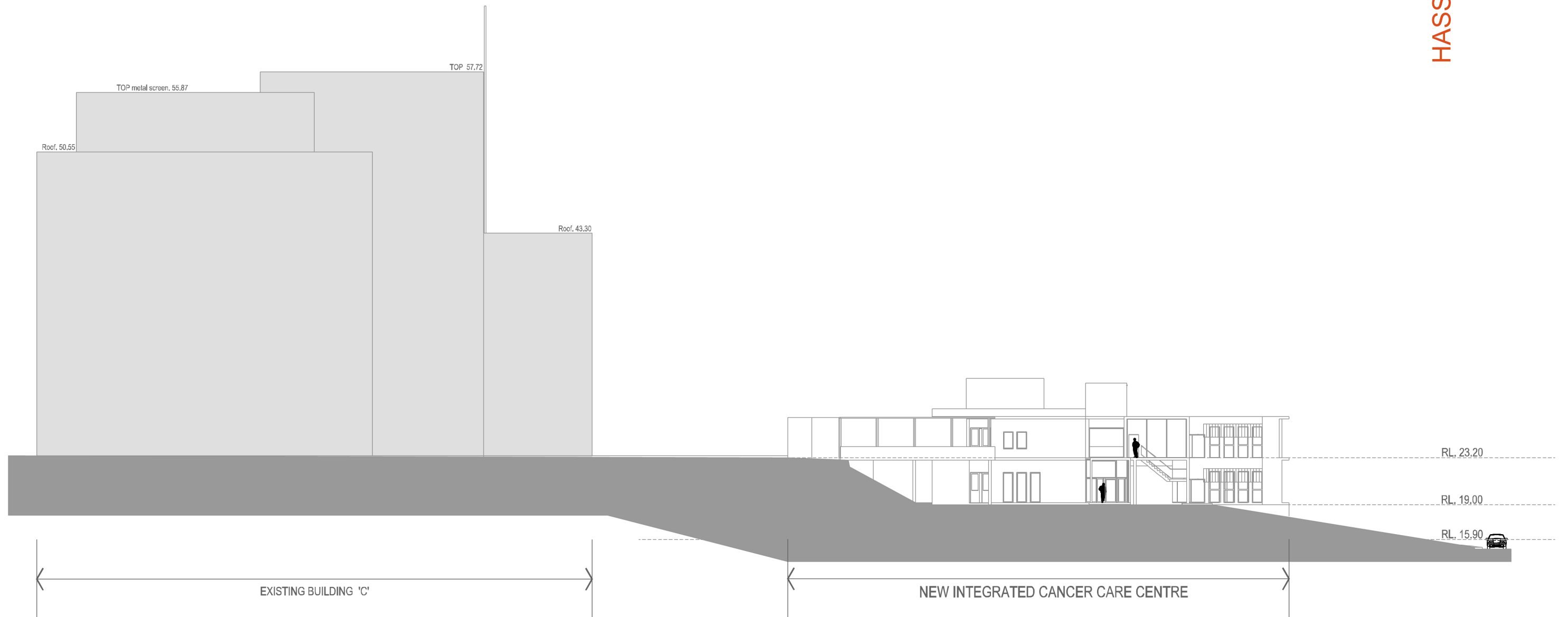
LISMORE BASE HOSPITAL NEW INTEGRATED CANCER CARE CENTRE EAST ELEVATION
