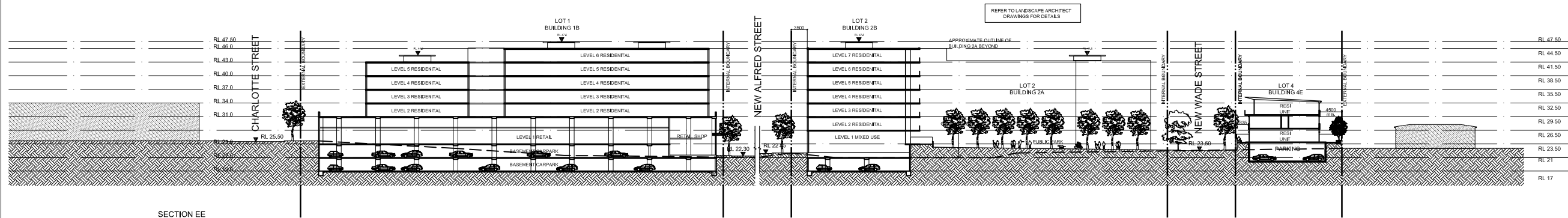
SECTION EE LOTS 1, 2 & 4 BULKY GOODS, RETAIL/RESIDENTIAL BUILDING & RESIDENTIAL TOWNHOUSES
