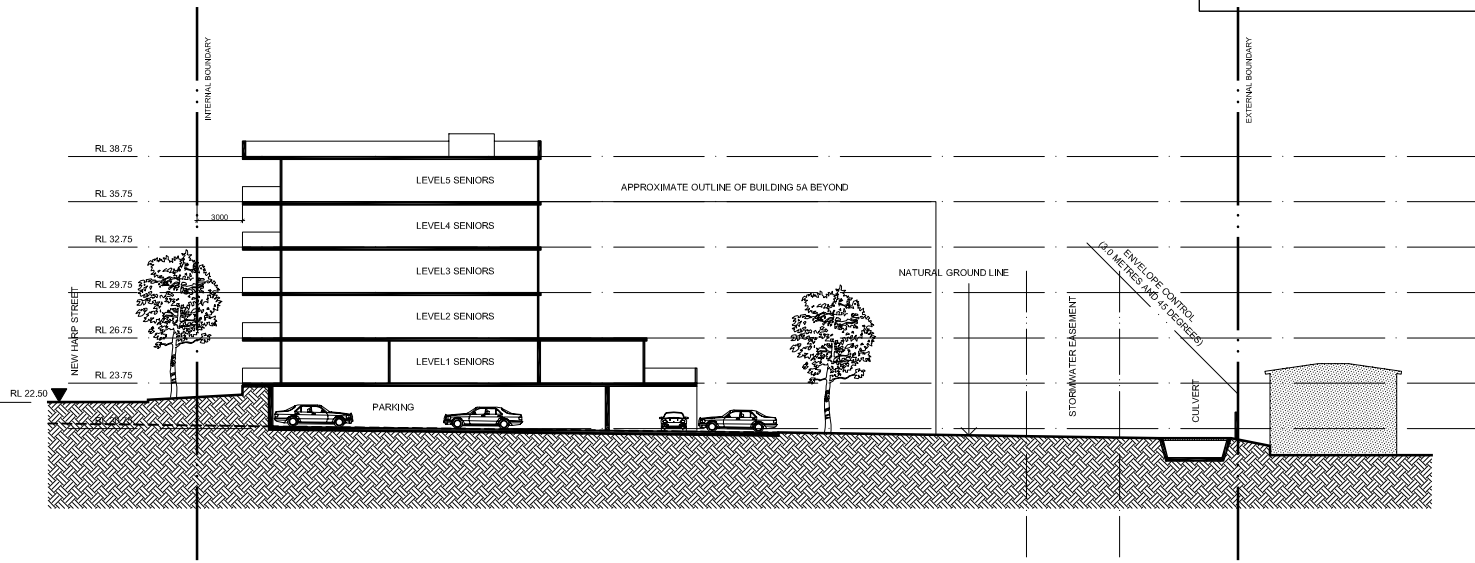
SECTION DD LOT 5B SENIORS LIVING COMPLEX
