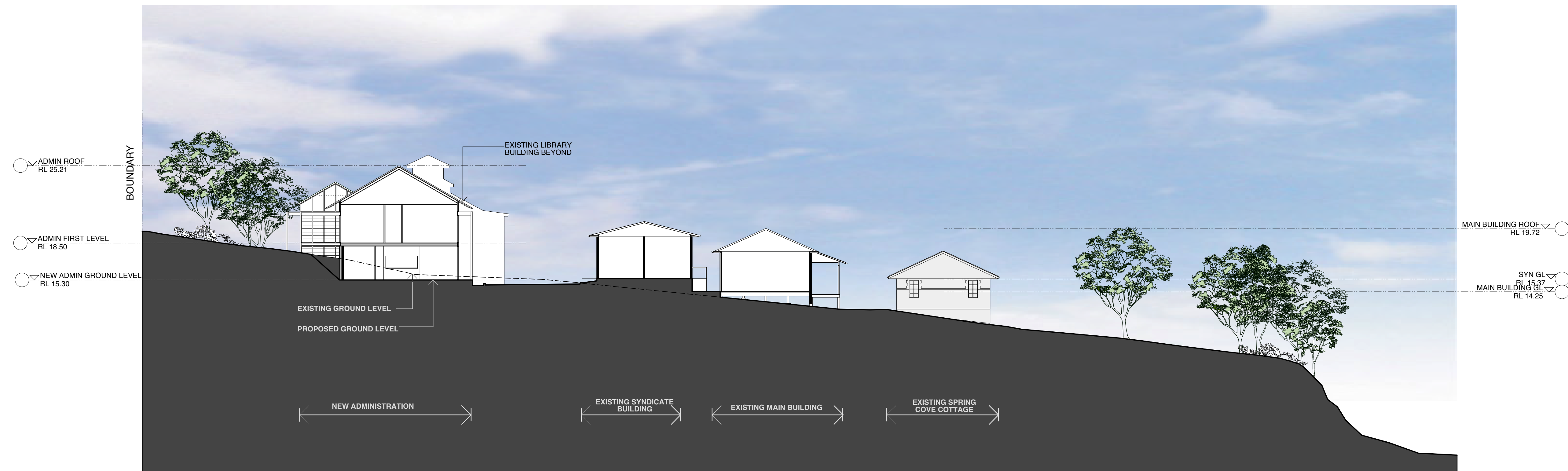
SECTION 08 WEST THROUGH MAIN BUILDING AND ADMIN SCALE 1:200
