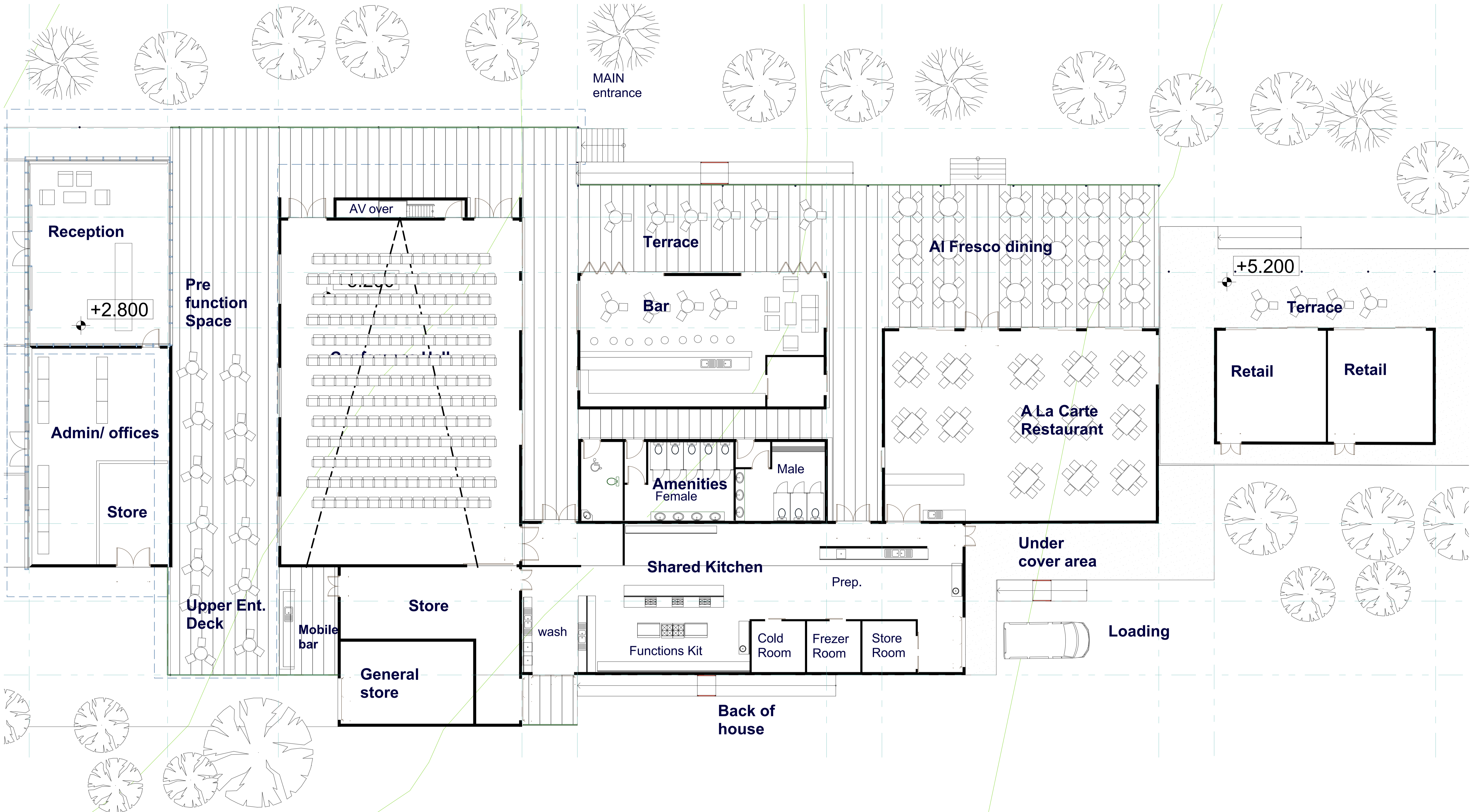
1 0. GROUND FLOOR PLAN 1:100
