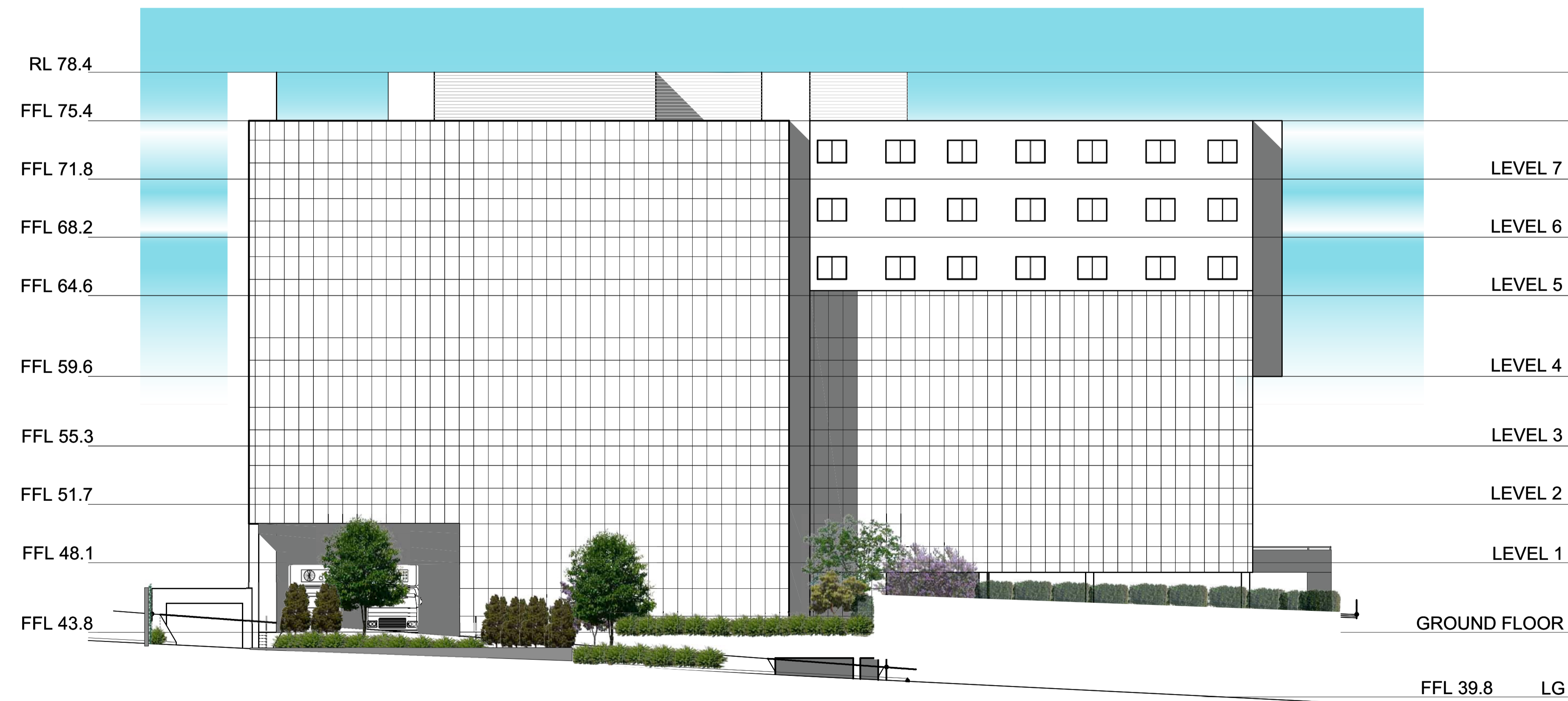
URUNGA PARADE ELEVATION
