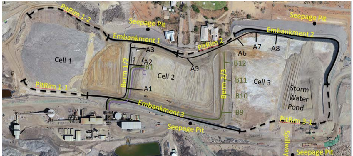
Figure 3-1 Layout of the Delivery and Return Lines at Blackwood Pit
