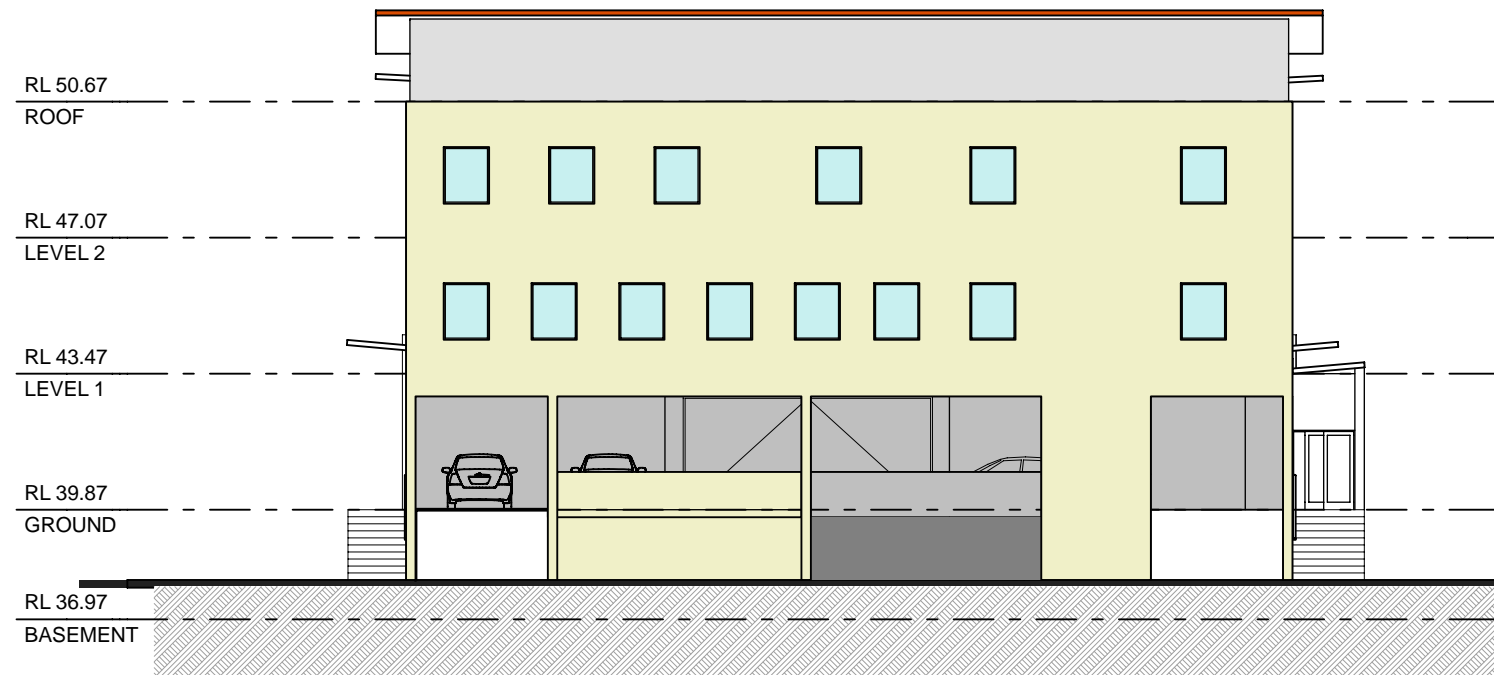
SOUTH ELEVATION
