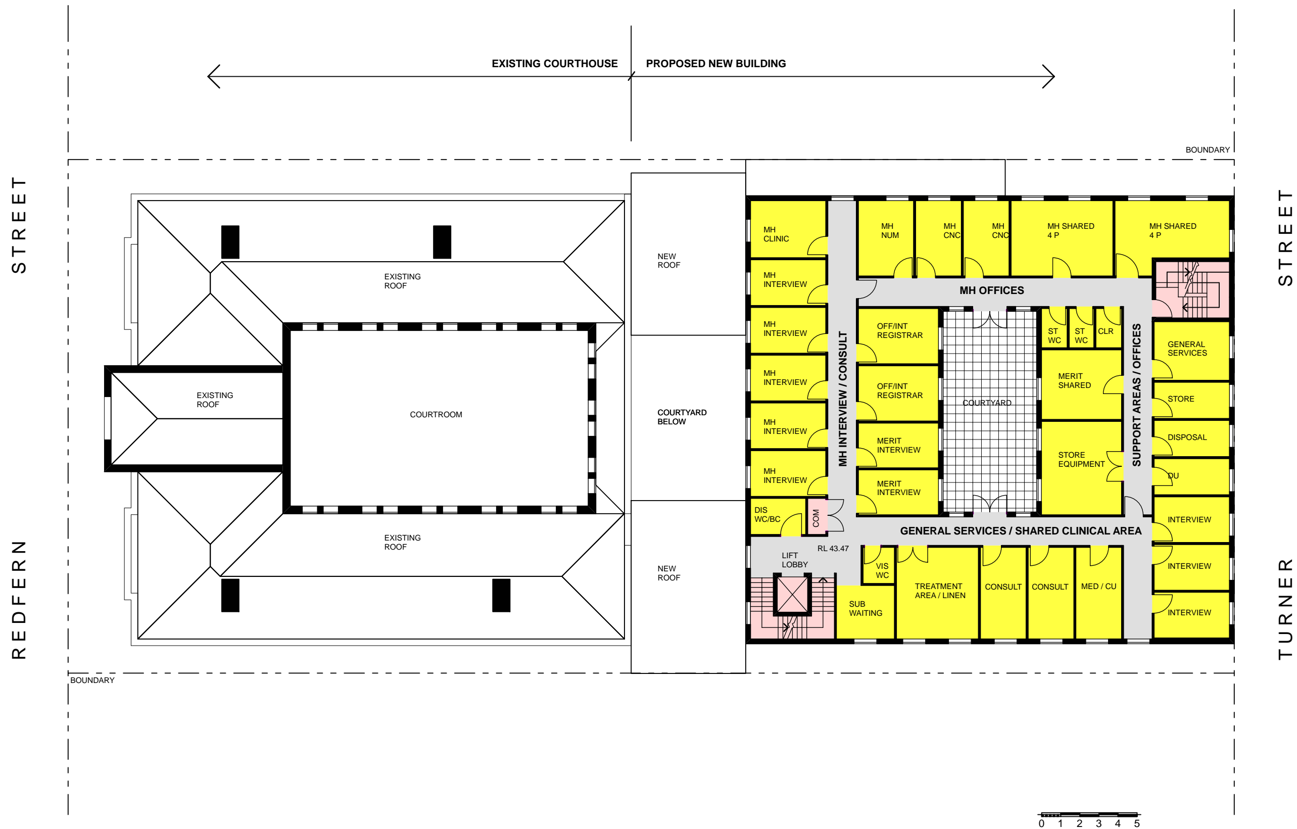
LEVEL 1 FLOOR PLAN
