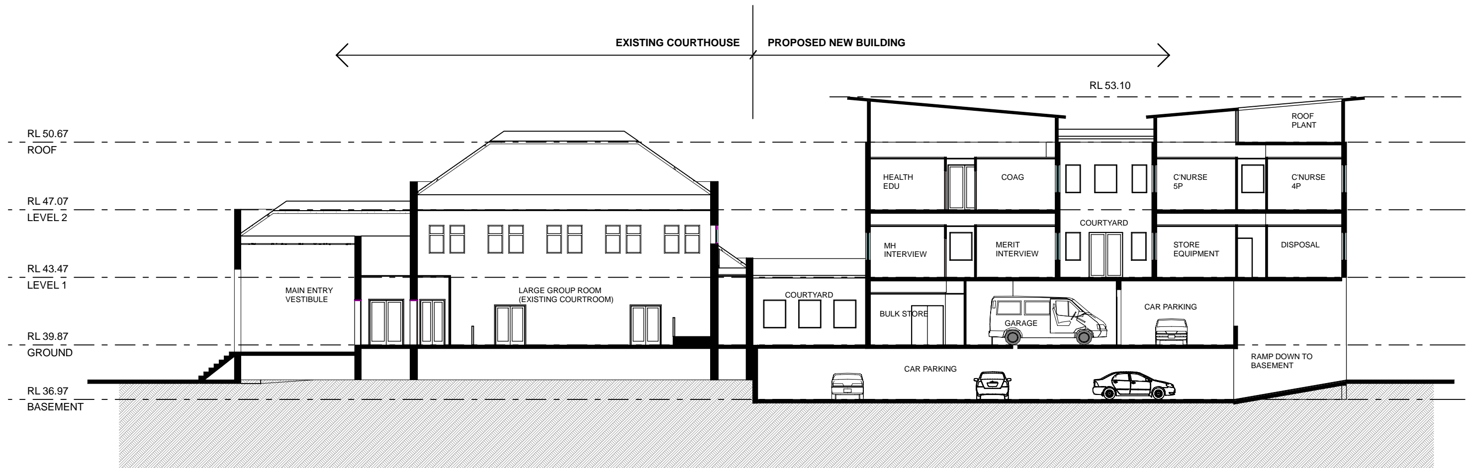
NORTH SOUTH SECTION
