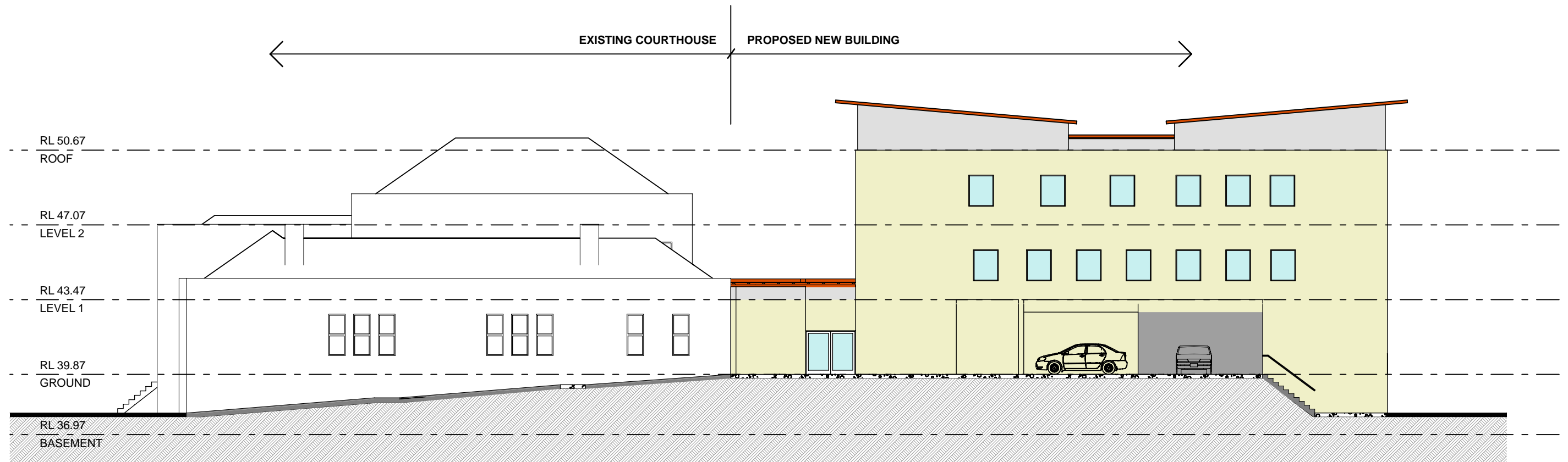
SOUTH ELEVATION
