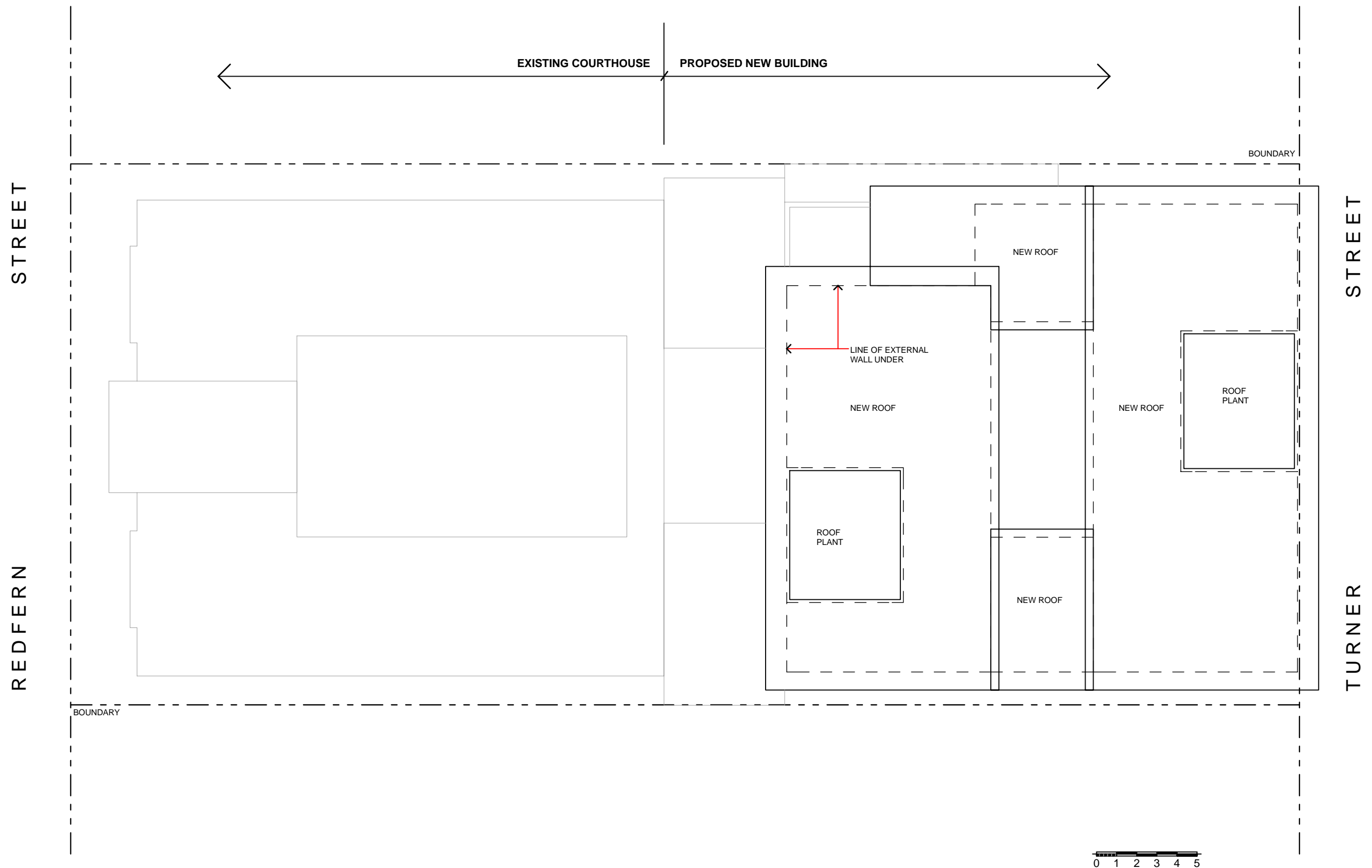
ROOF PLAN
