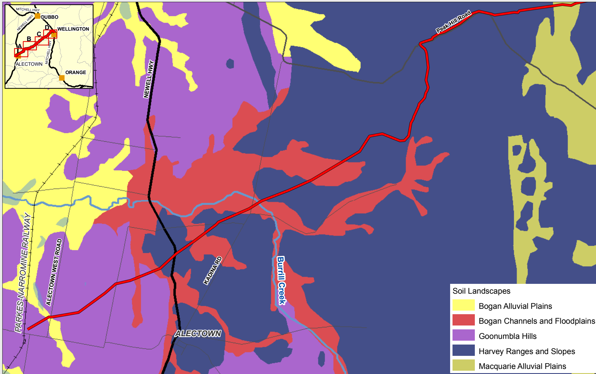
Figure C-1 Pipeline Section A - Soils
