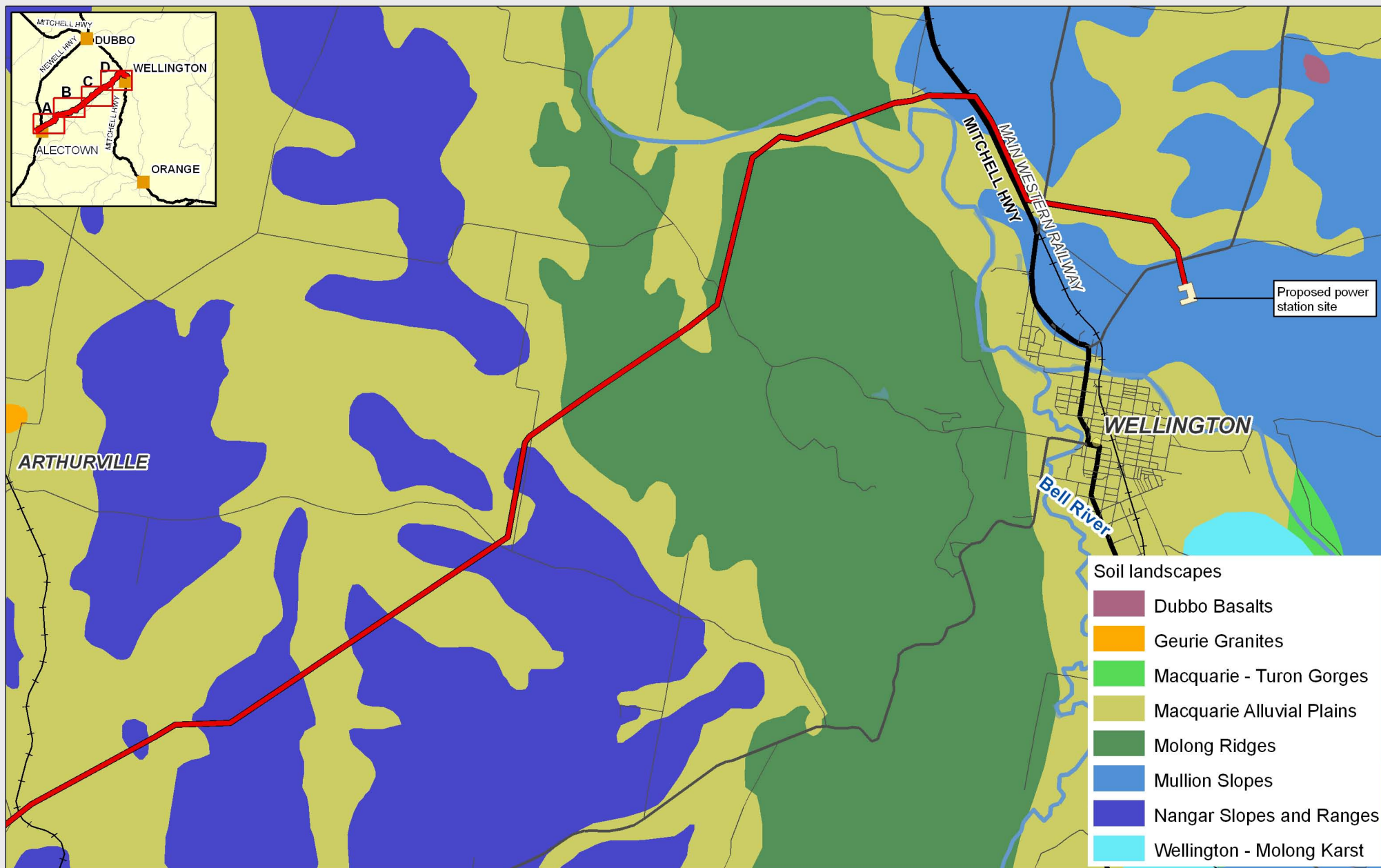
Figure C-4 Pipeline Section D - Soils
