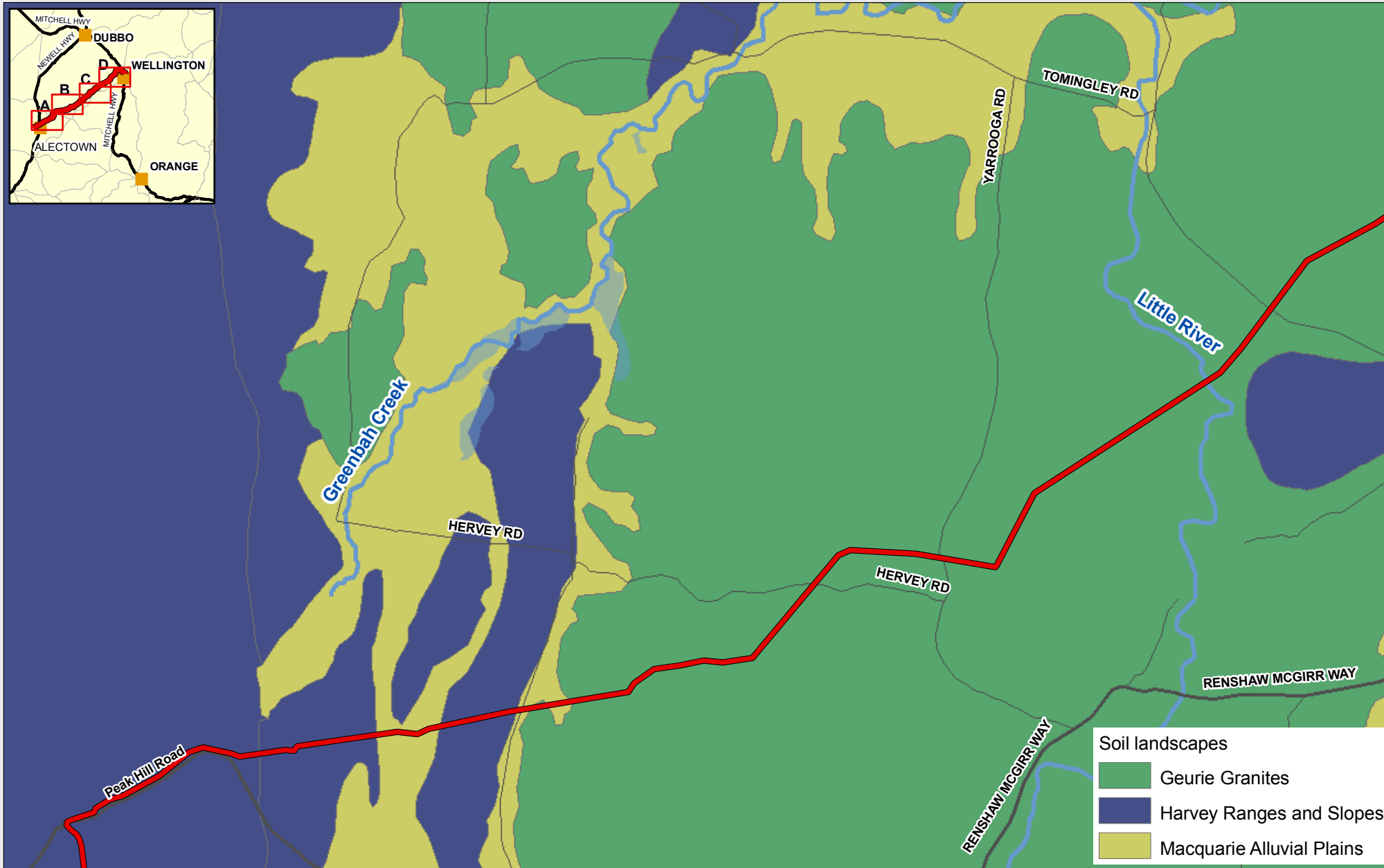
Figure C-2 Pipeline Section B - Soils
