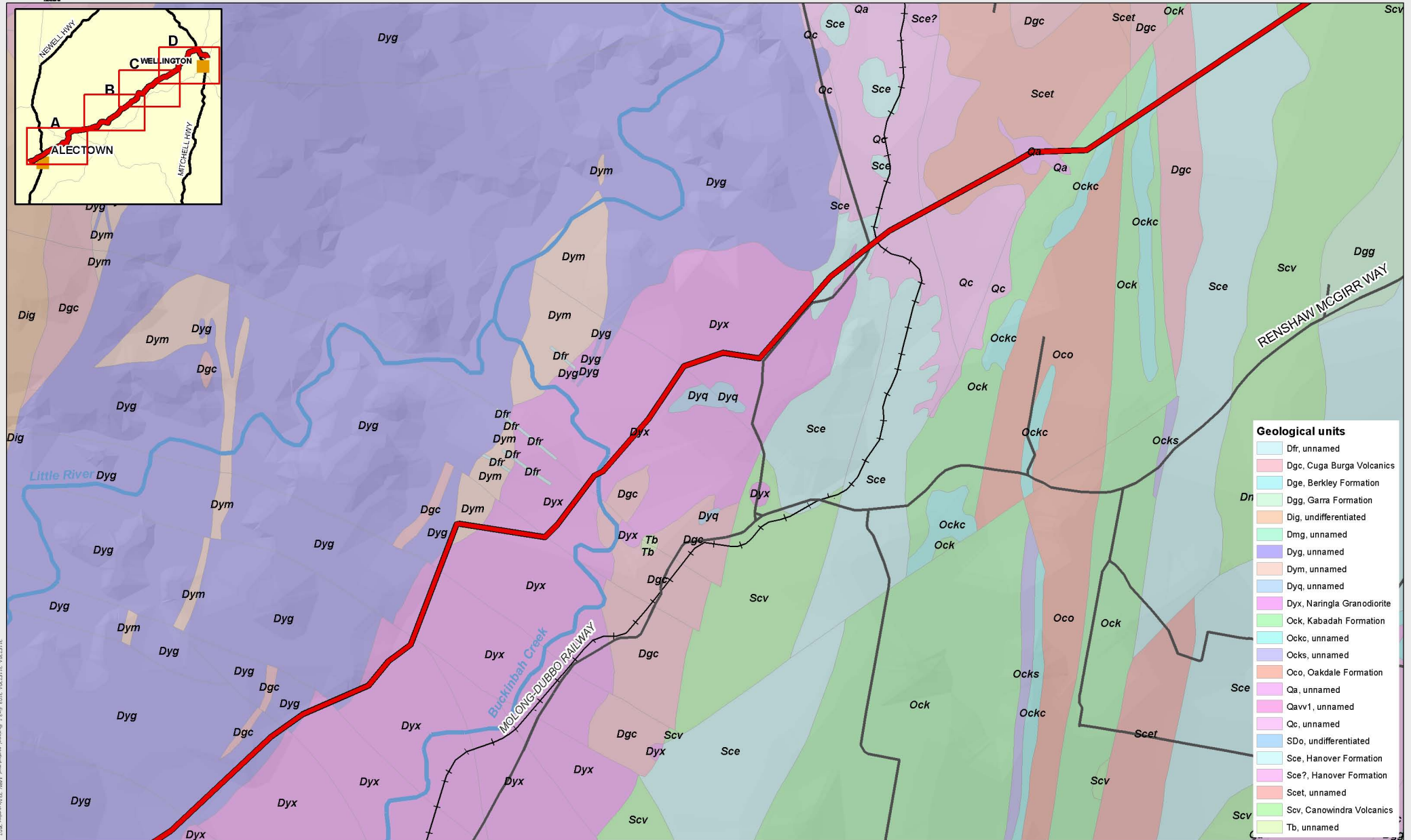
Figure B-3: Pipeline Section C - Geology
