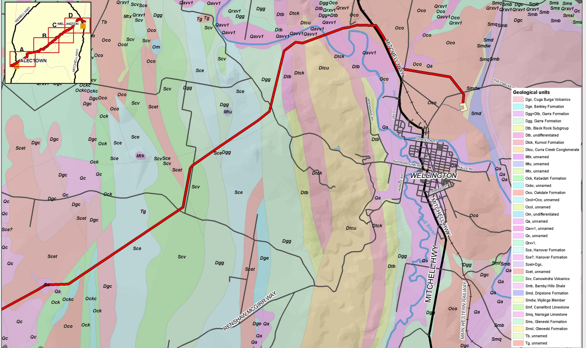
Figure B-4 Pipeline Section D- Geology
