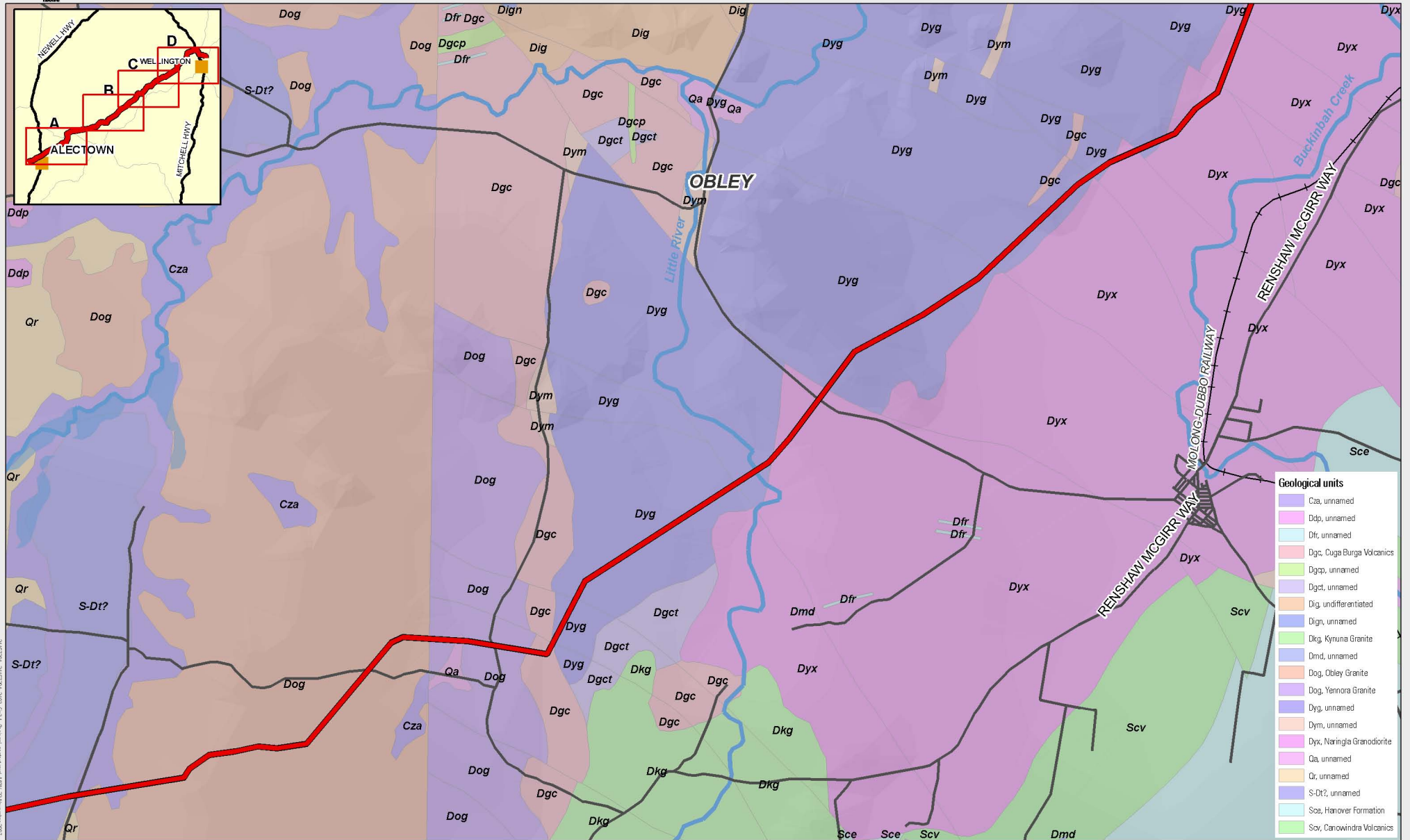
Figure B-2 Pipeline Section B - Geology
