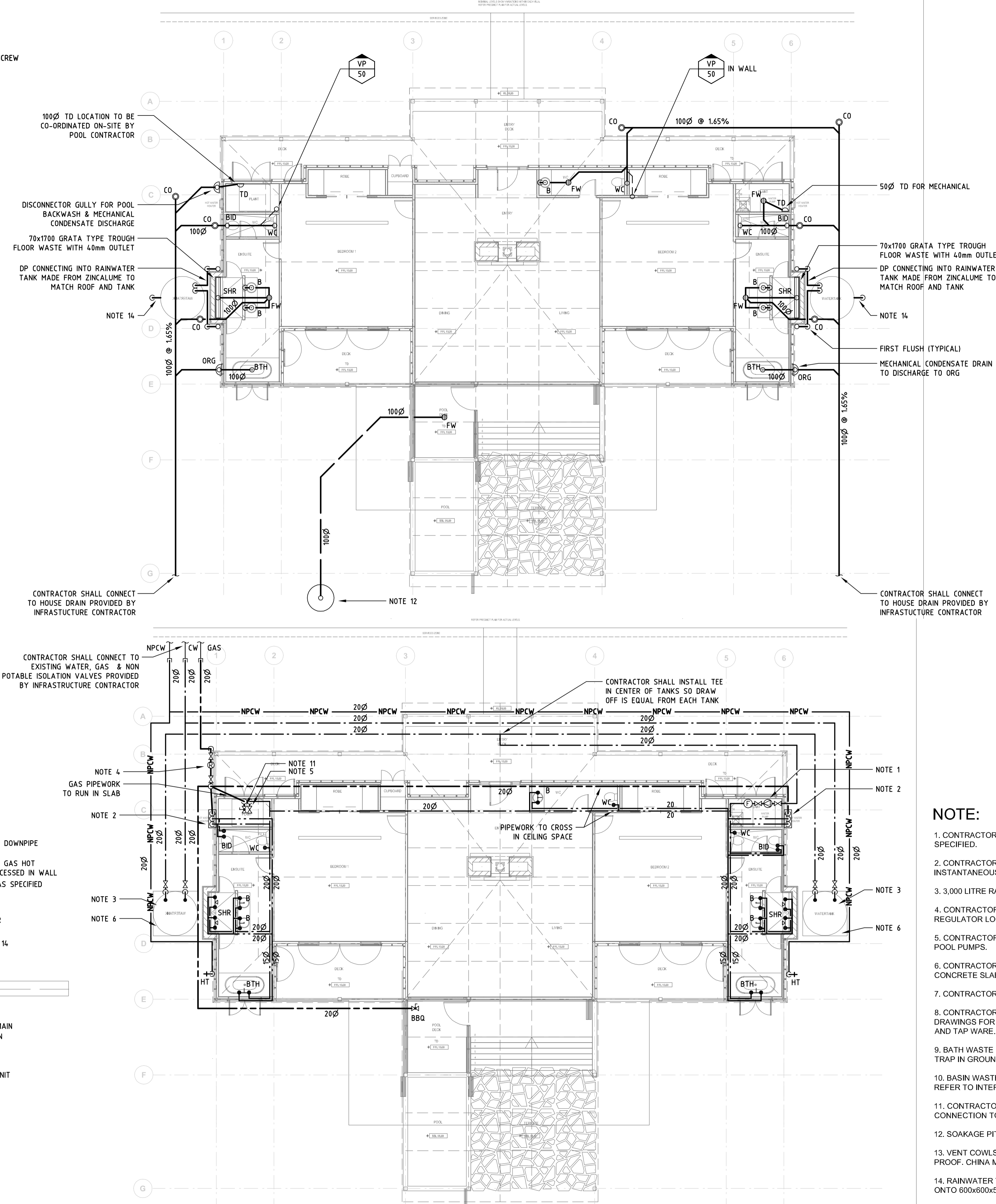
WATER & GAS LAYOUT
