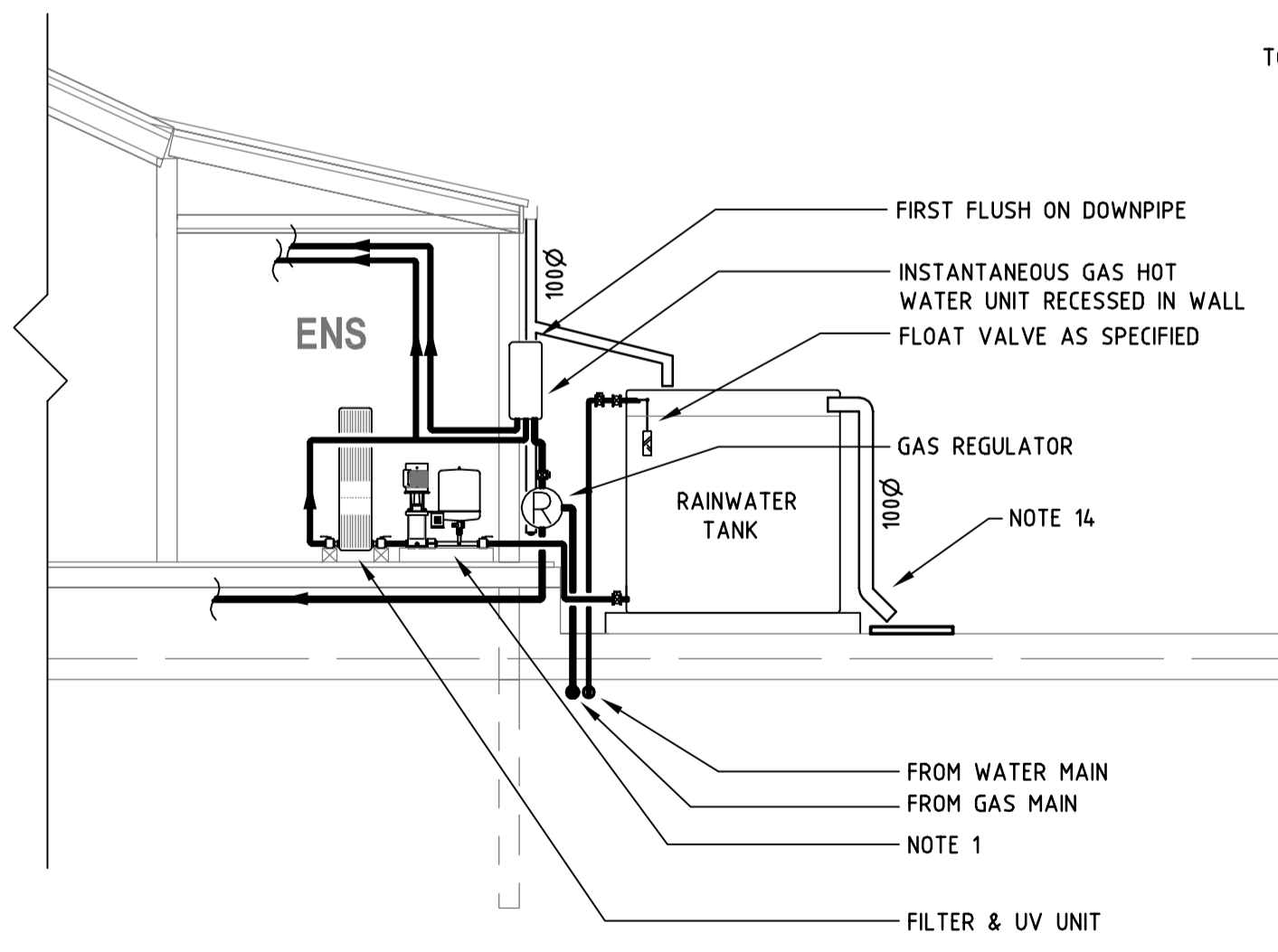
TYPICAL PLANT ROOM SECTION NOT TO SCALE
