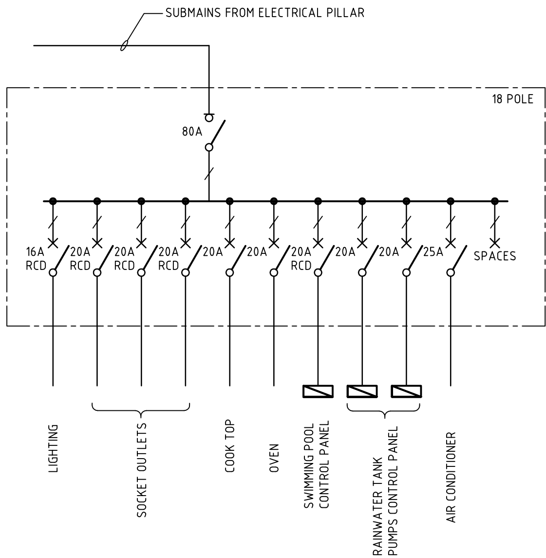
OWNER'S VILLA-DB SCHEMATIC
