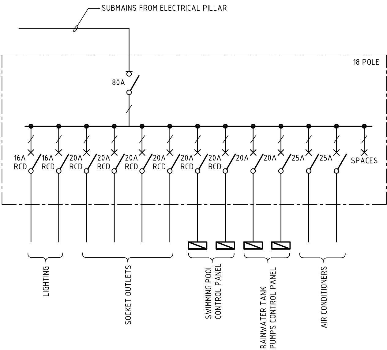
DUPLEX VILLA-DB SCHEMATIC
