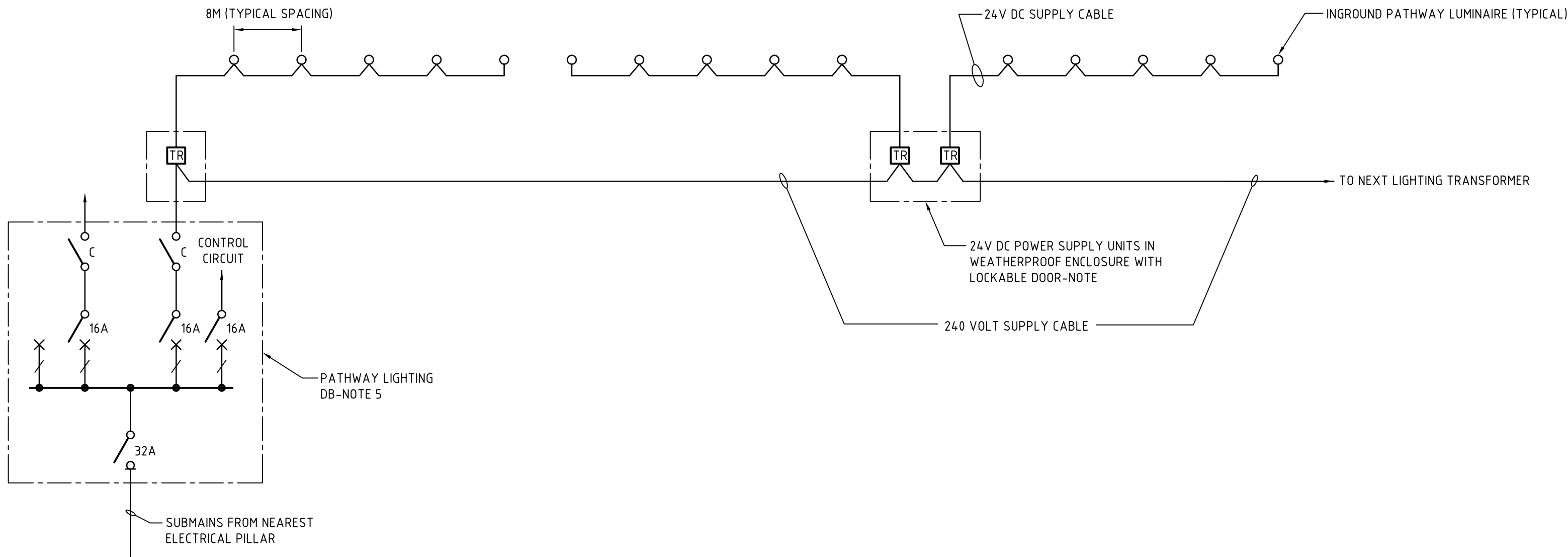
PATHWAY LIGHTING ARRANGEMENT DIAGRAM (TYPICAL FOR PATHWAY LIGHTING AT RESORT PRECINCT)
