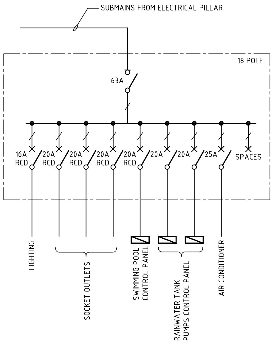
2 BEDROOM VILLA-DB SCHEMATIC
