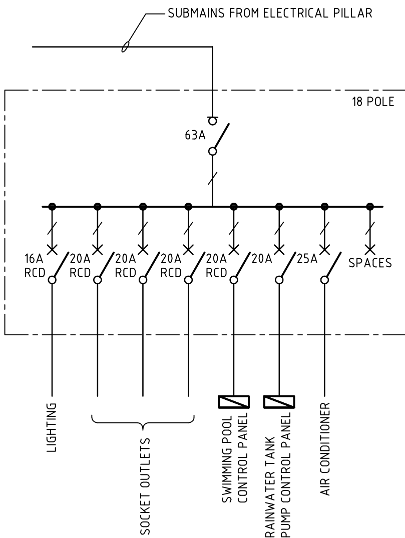
1 BEDROOM VILLA-DB SCHEMATIC
