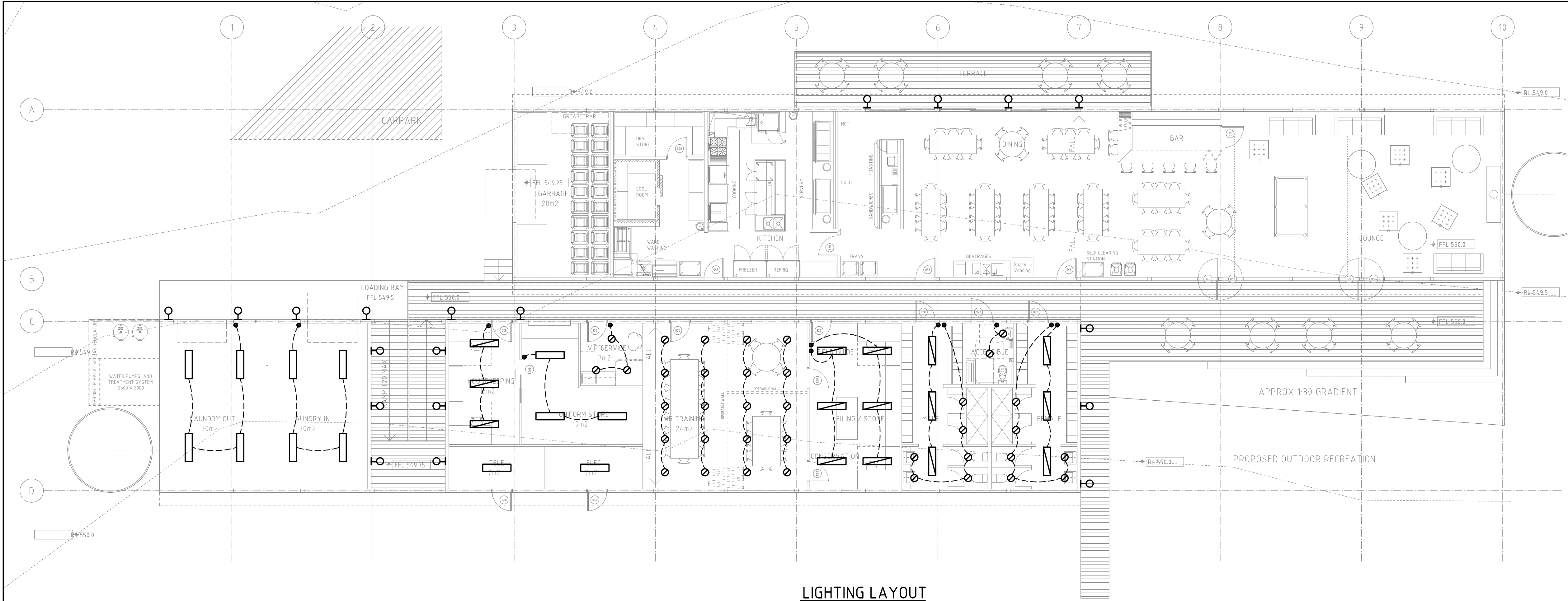
LIGHTING LAYOUT
