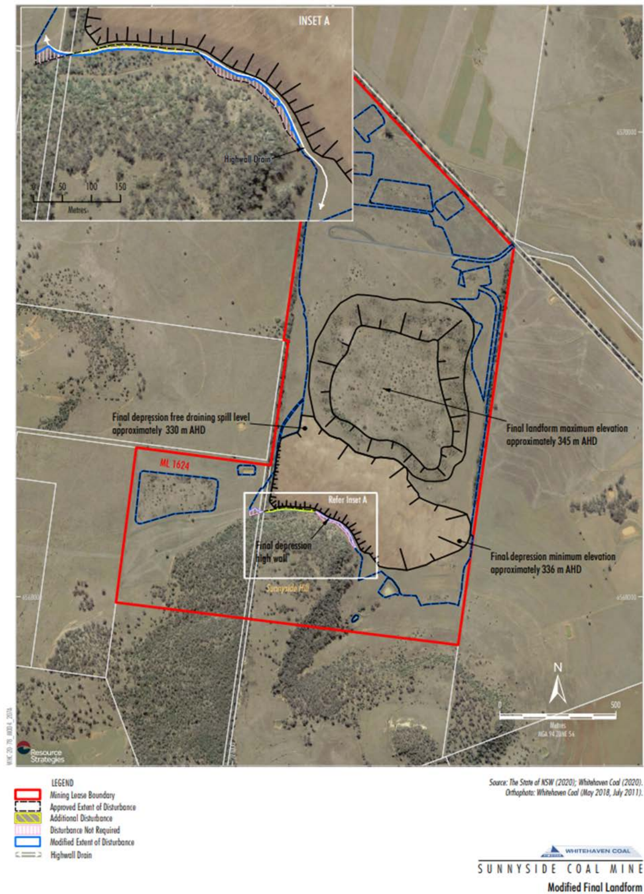
Figure 4: Final Landform
