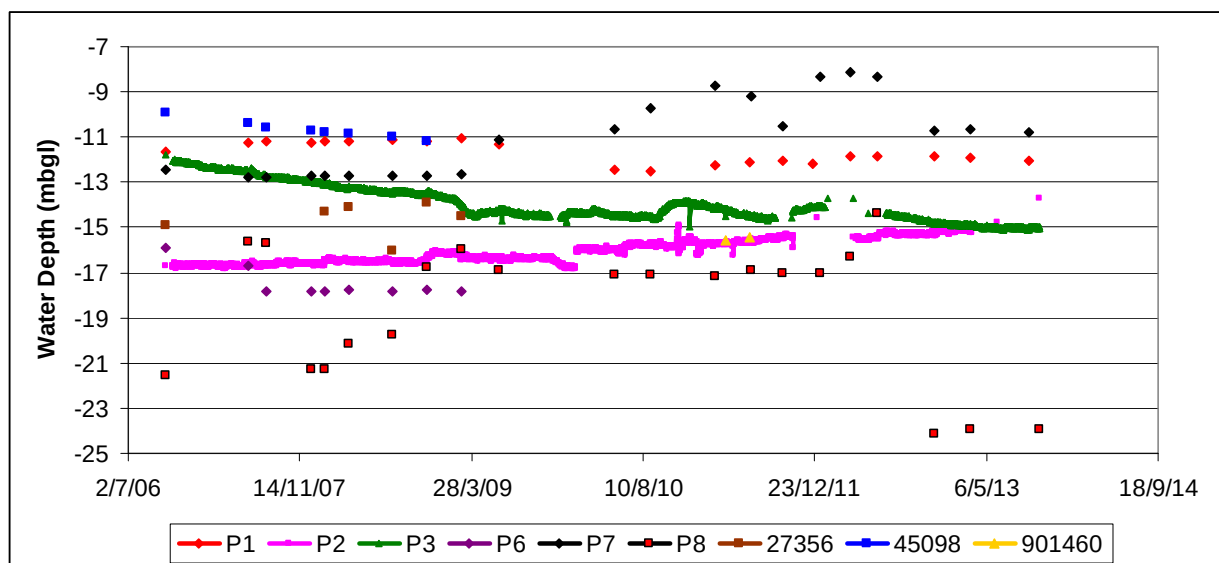
Figure 3 Observed Water Level Change
