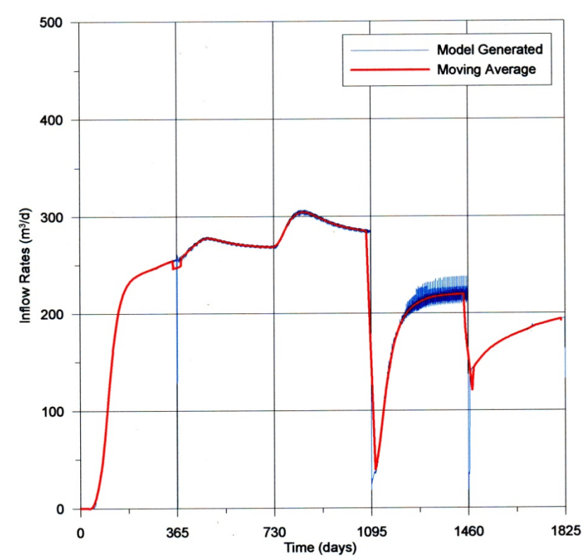
Figure 2 Modelled Pit Groundwater Inflow
