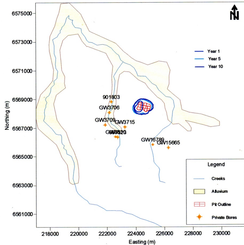
Figure 1 Predicted Drawdown <5 years in Hoskissons Seam Overburden
