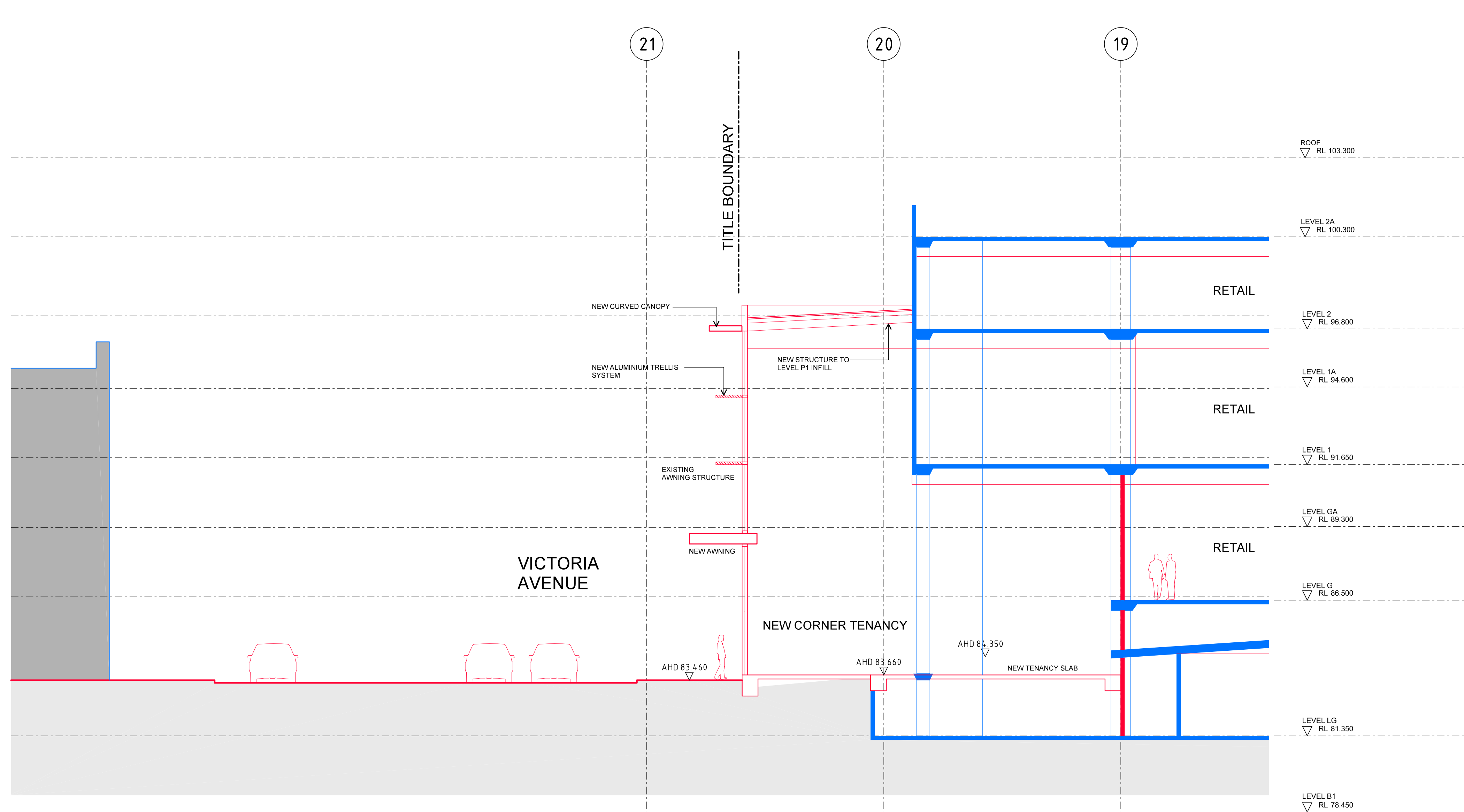
01 SECTION - NEW RETAIL TENANCY --- SCALE 1:100 VICTORIA AVE
