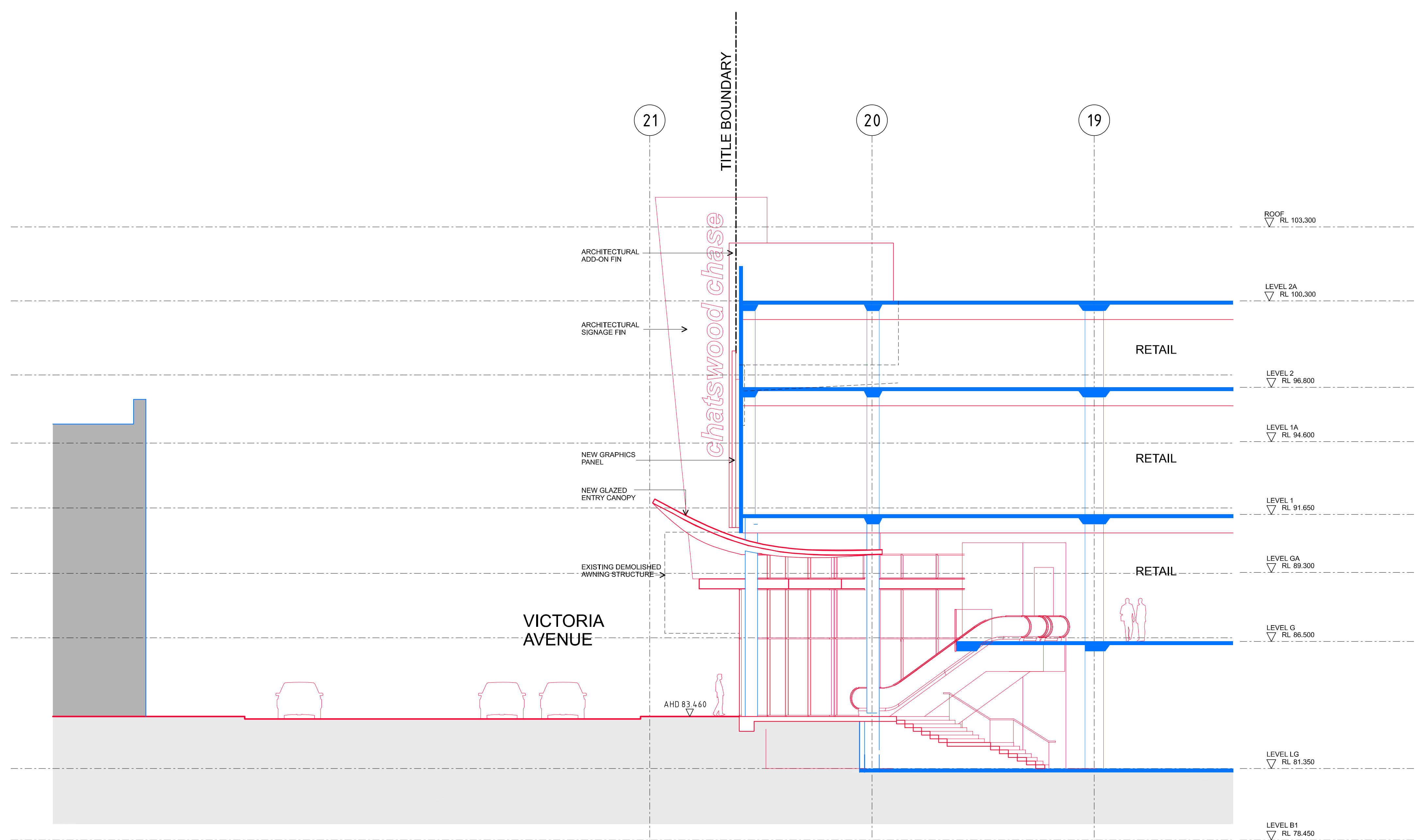
02 SECTION - VICTORIA AVE MAIN ENTRY SCALE 1:100 VICTORIA AVE
