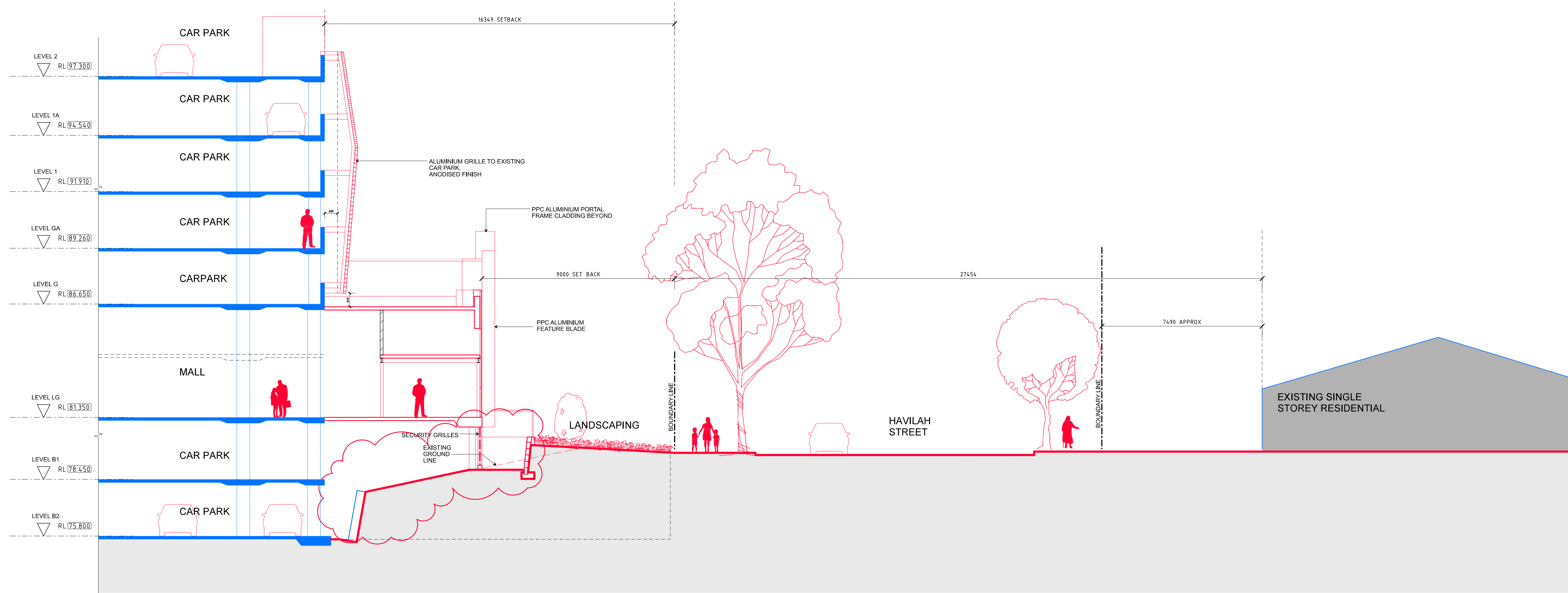
07 SECTION - LOWER GROUND RETAIL & SCREEN SCALE 1:100 HAVILAH STREET
