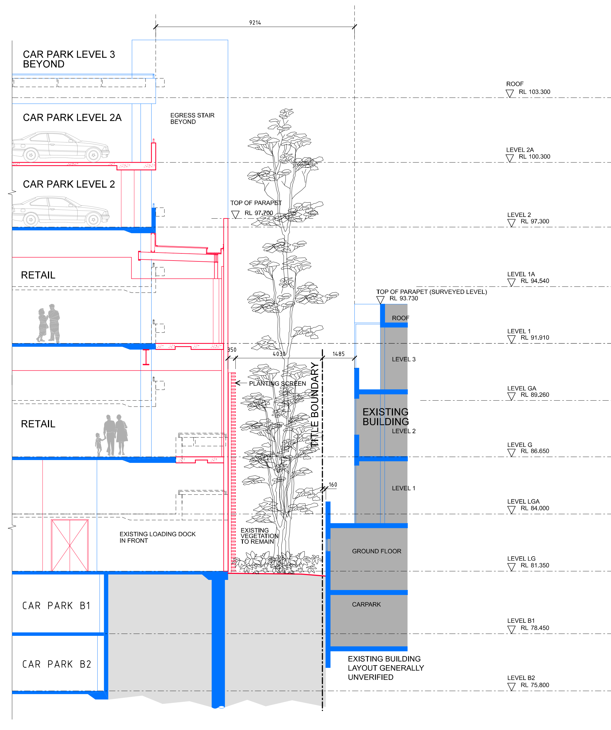
10 SECTION - RETAIL EXTENSION OF EXISTING CARPARK DECKS SCALE 1:100 HAVILAH STREET
