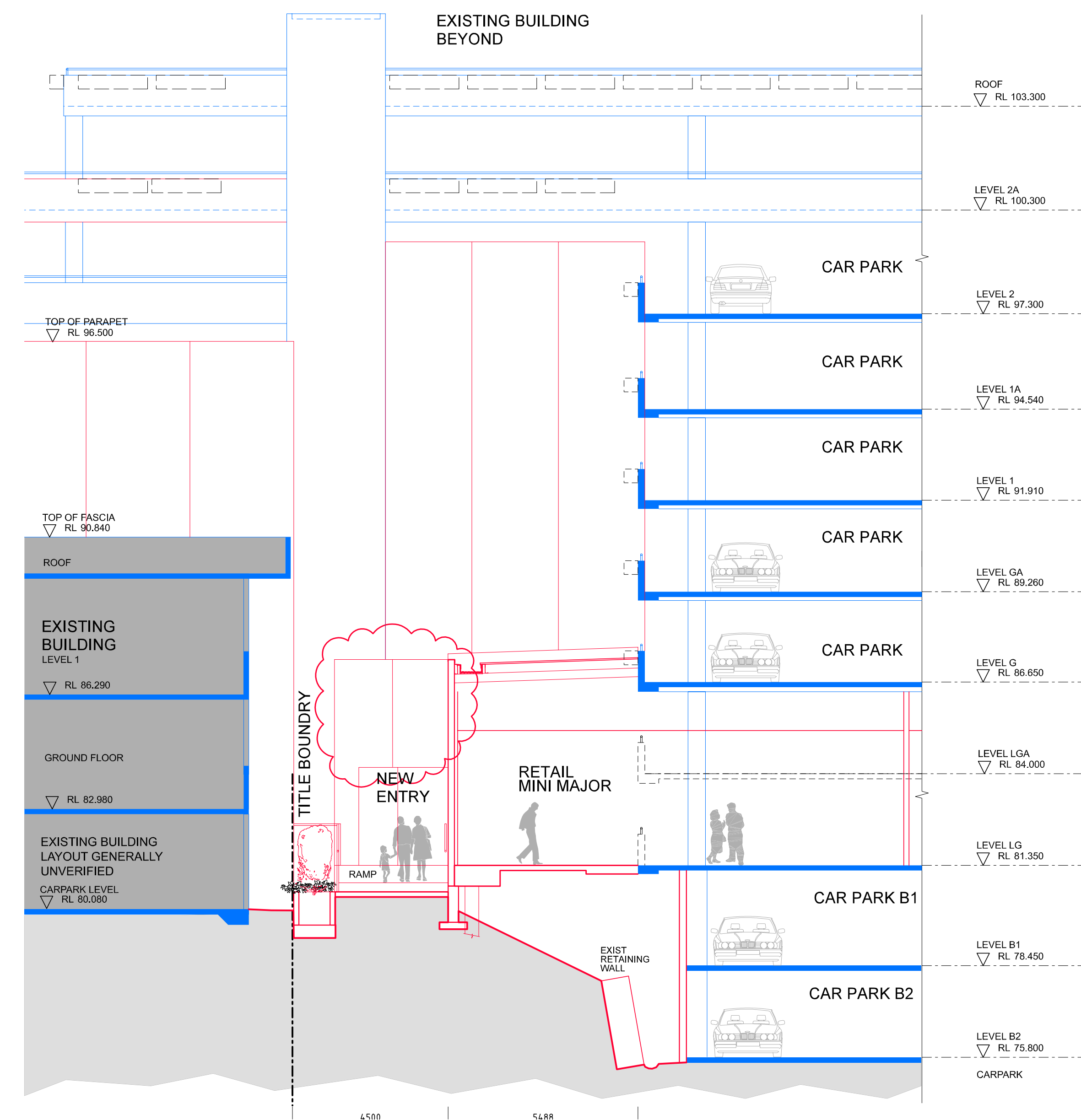
08 SECTION - HAVILAH STREET ENTRANCE SCALE 1:100 HAVILAH STREET
