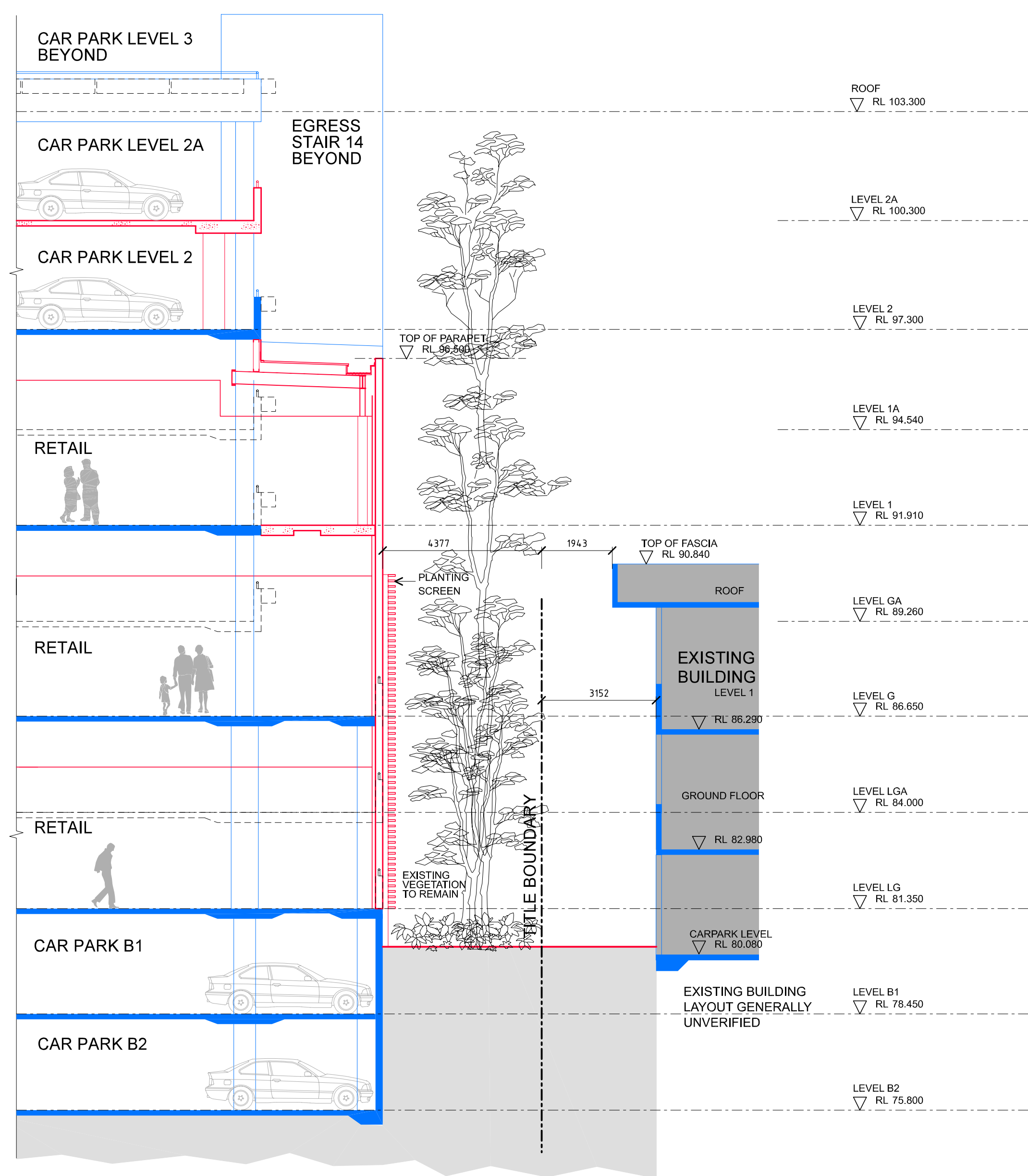
09 SECTION - RETAIL EXTENSION OF EXISTING CARPARK DECKS SCALE 1:100 HAVILAH STREET
