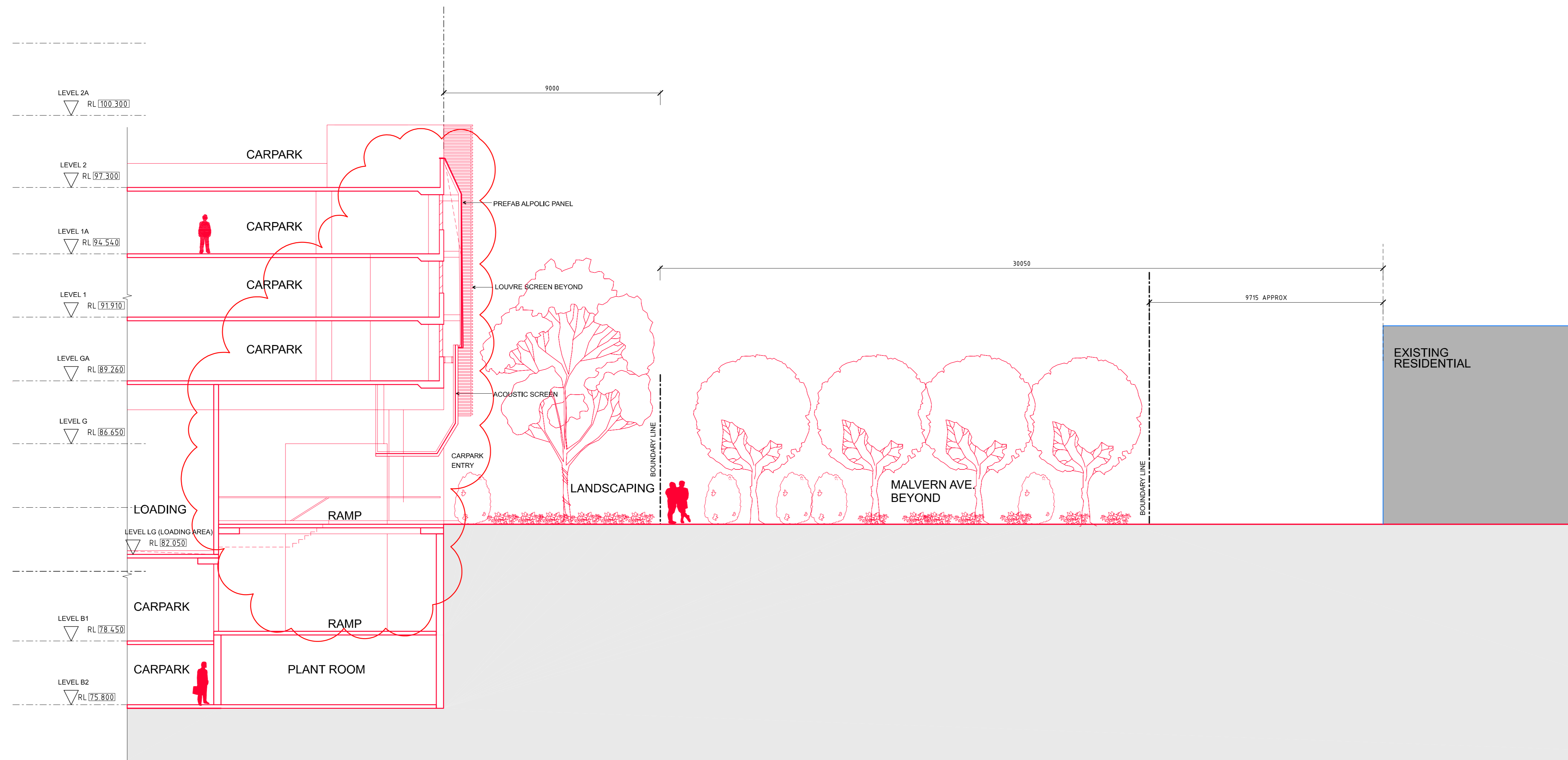
17 SECTION-CARPARK ENTRY SCALE 1:100 MALVERN AVENUE
