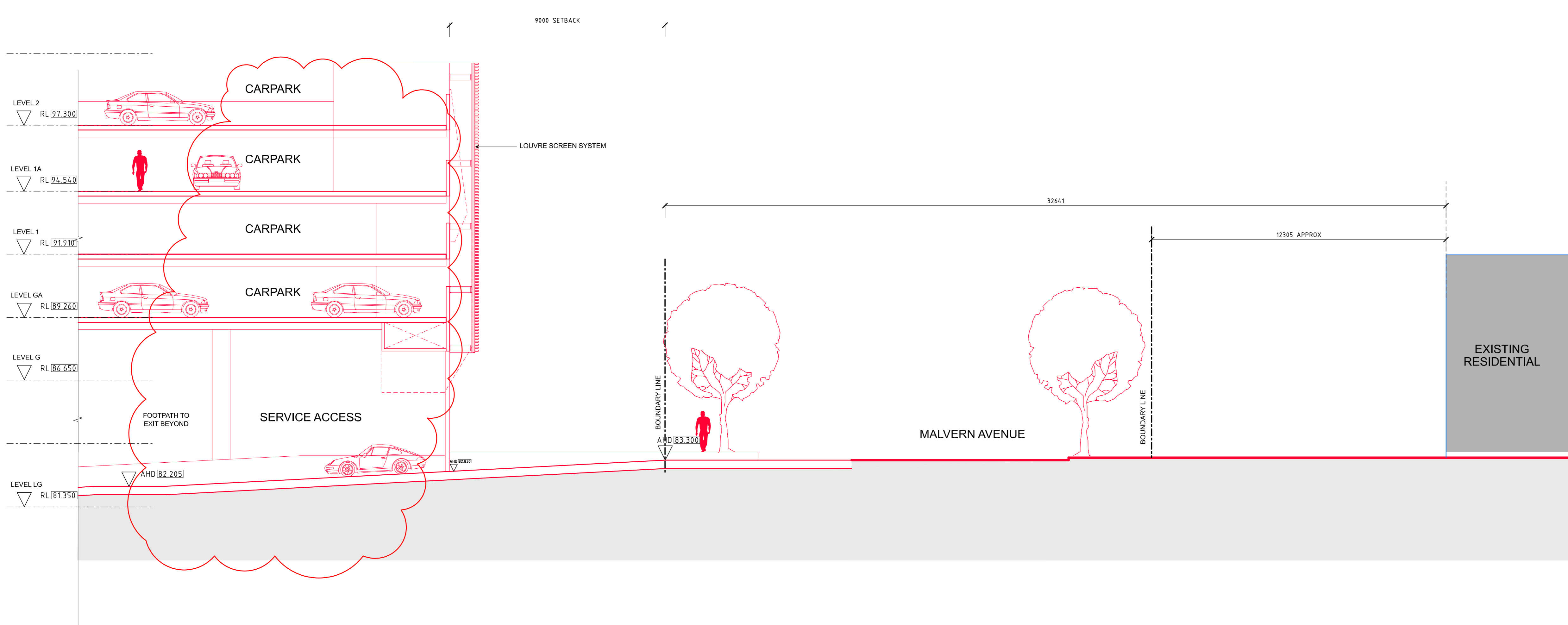
18 SECTION-SERVICE ENTRY SCALE 1:100 MALVERN AVENUE
